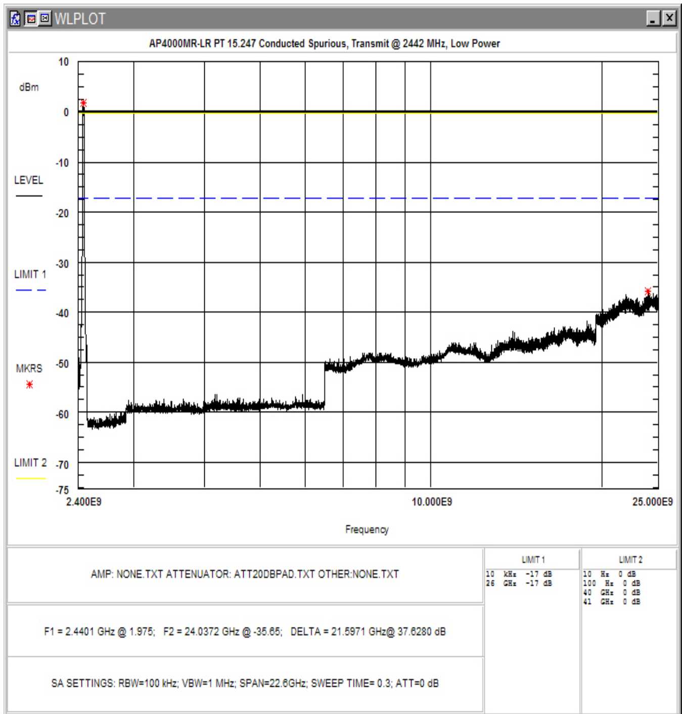
Figure 4-12. Conducted Spurious Emissions, Low Power: Mid Channel 2.4 - 25GHz
