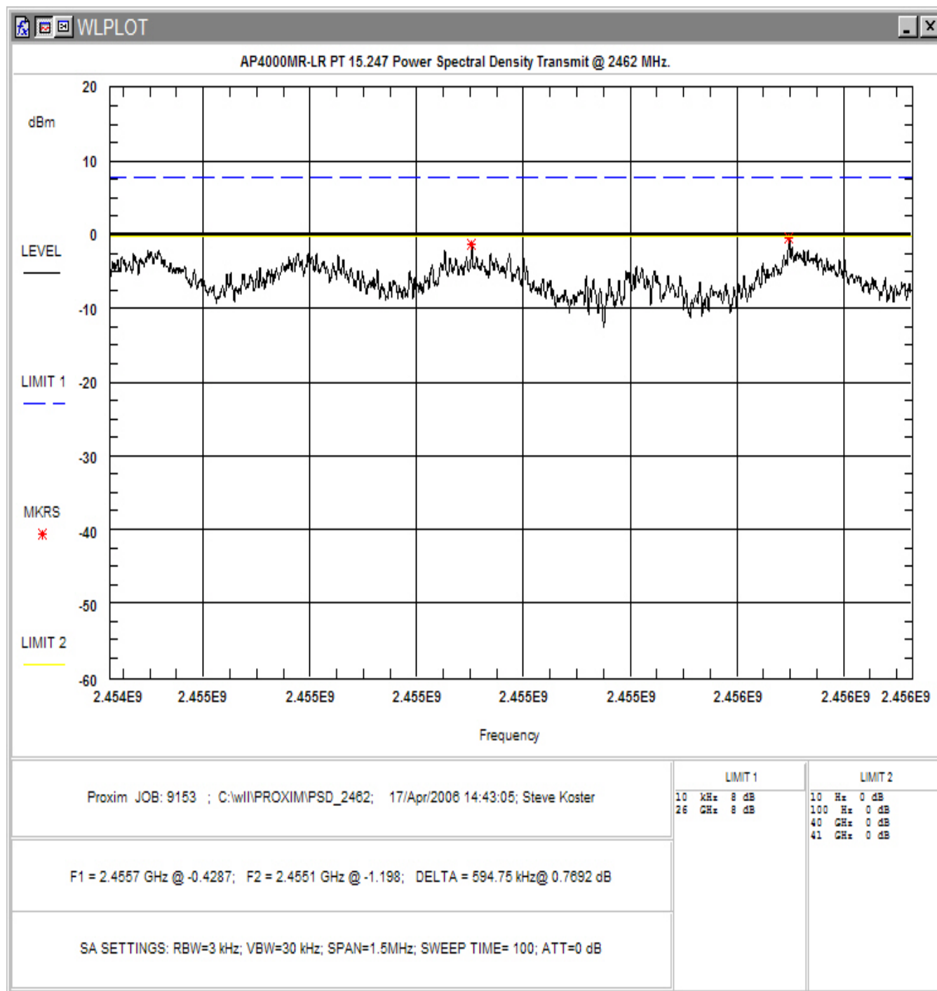
Figure 4-7: Power Spectral Density, High Channel
