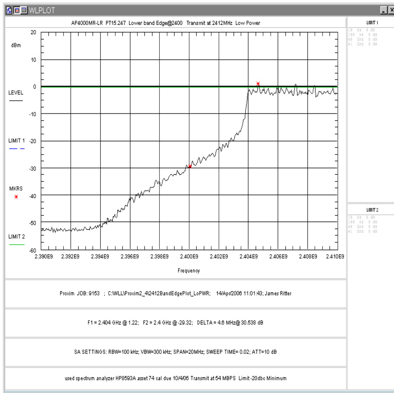
Figure 4-8. Conducted Spurious Emissions, Low Power: Low Channel Band Edge
