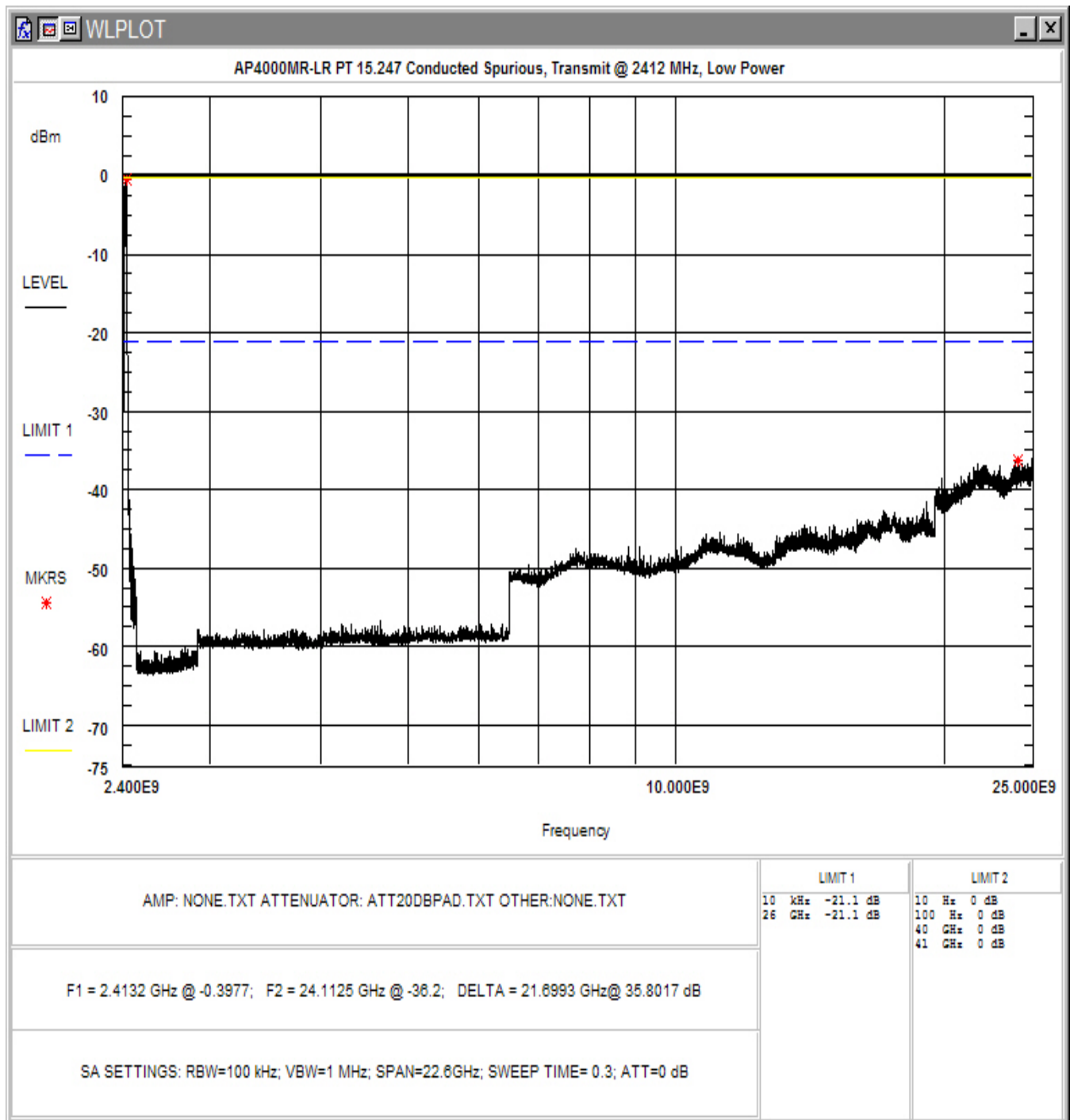
Figure 4-10. Conducted Spurious Emissions, Low Power: Low Channel 2.4– 25GHz
