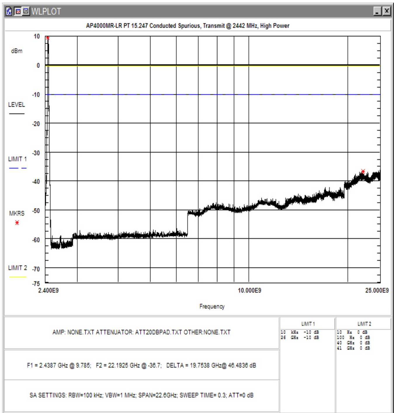
Figure 4-20. Conducted Spurious Emissions, High Power: Mid Channel 2.4 - 25GHz
