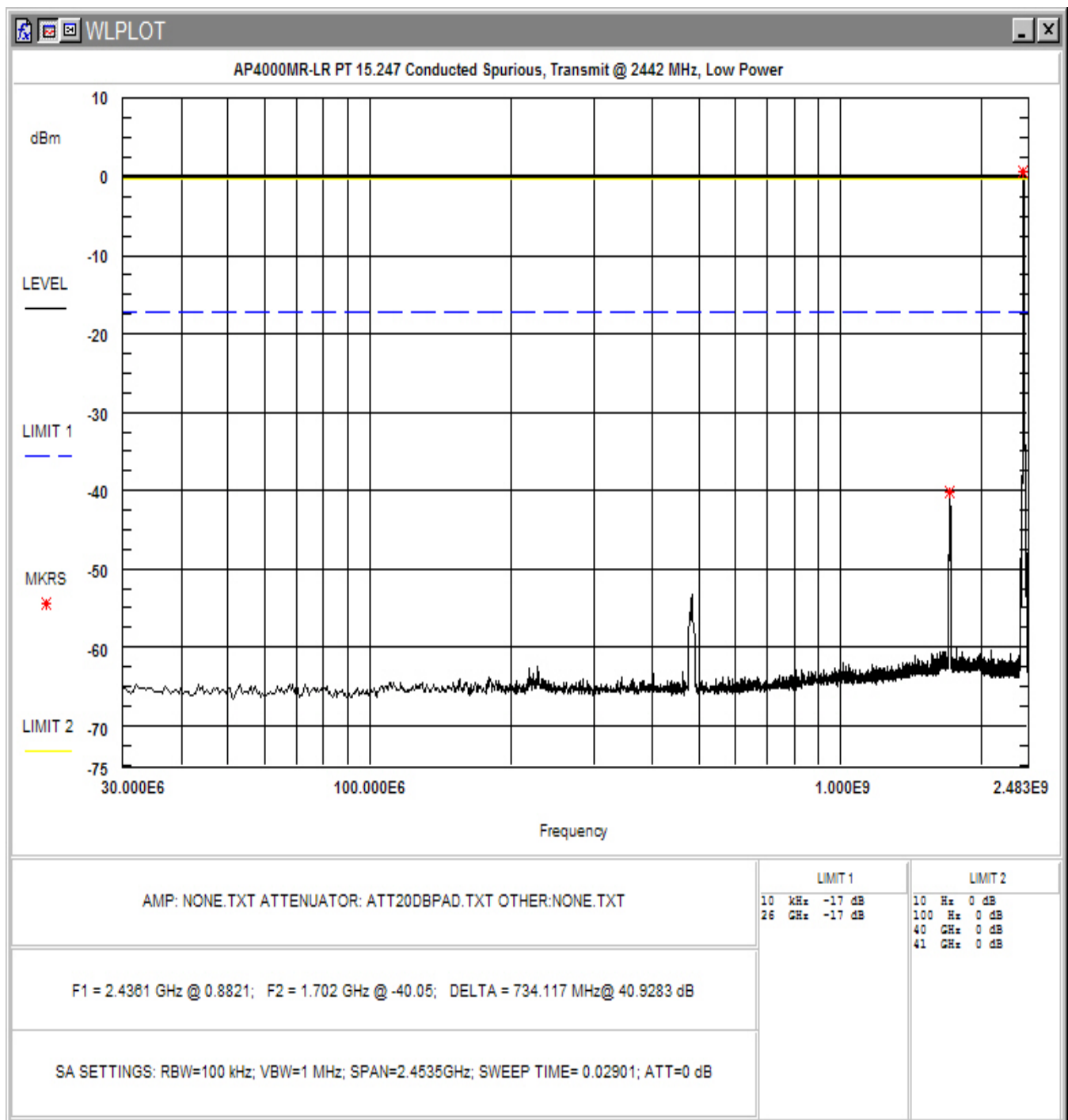
Figure 4-11. Conducted Spurious Emissions, Low Power: Mid Channel 30 – 2483MHz
