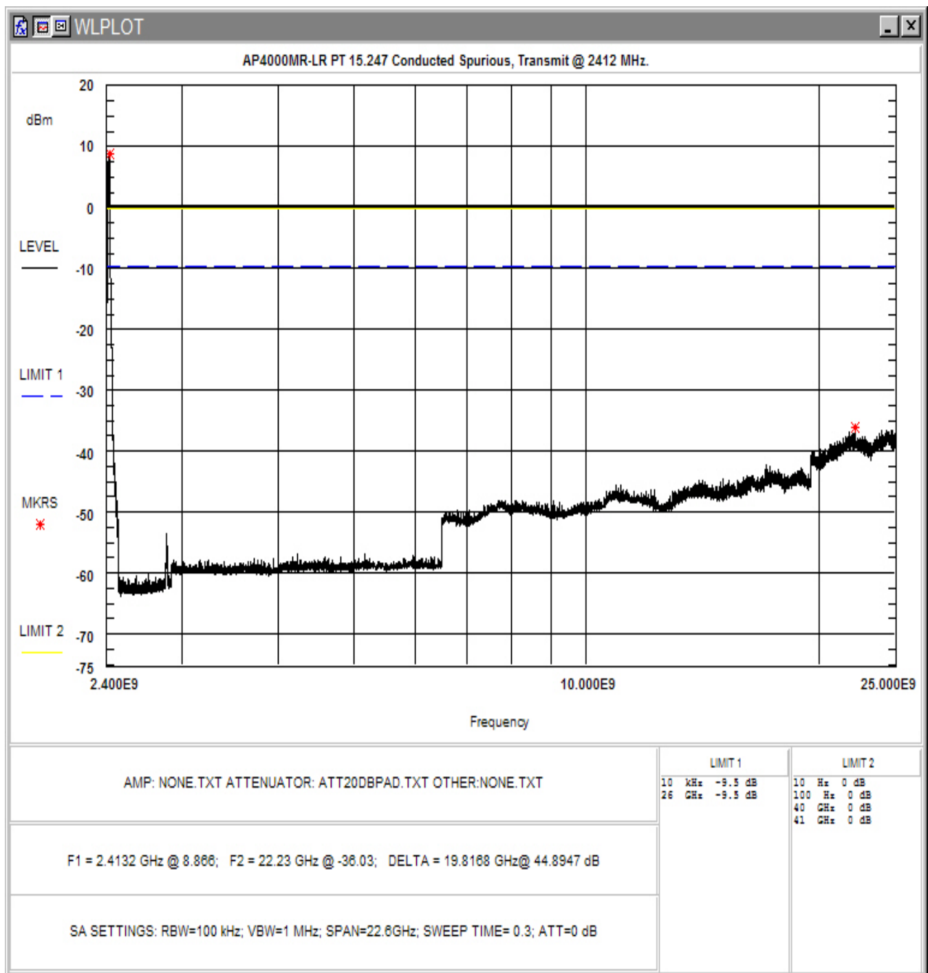
Figure 4-18. Conducted Spurious Emissions, High Power: Low Channel 2.4 – 25GHz
