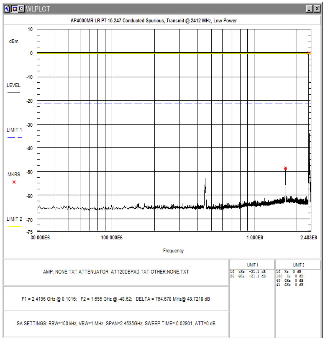
Figure 4-9. Conducted Spurious Emissions, Low Power: Low Channel 30 - 2483MHz
