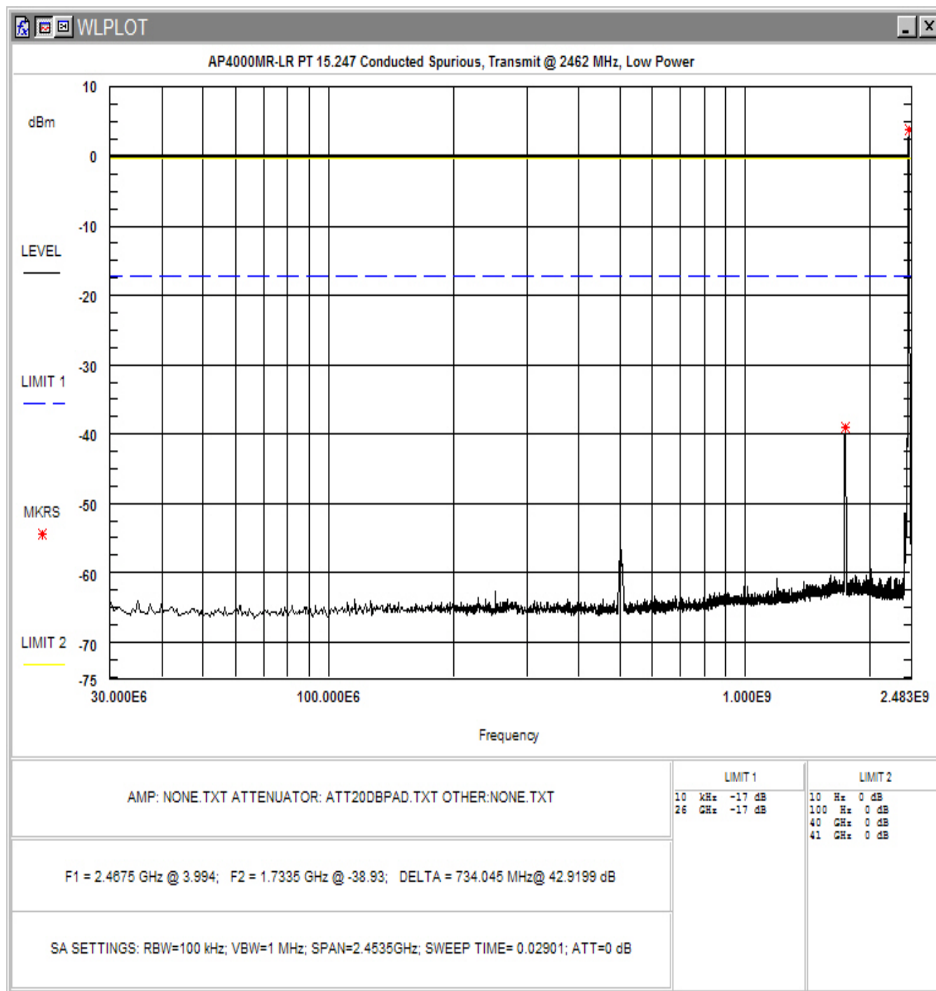
Figure 4-14. Conducted Spurious Emissions, Low Power: High Channel 30 – 2483MHz
