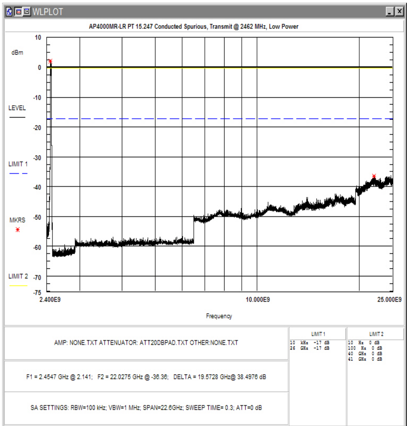
Figure 4-15. Conducted Spurious Emissions, Low Power: High Channel 2.4 - 25GHz
