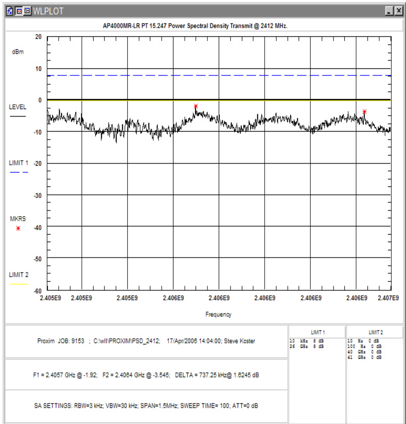
Figure 4-5: Power Spectral Density, Low Channel
