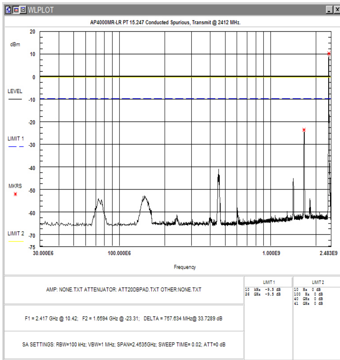
Figure 4-17. Conducted Spurious Emissions, High Power: Low Channel 30 - 2483MHz
