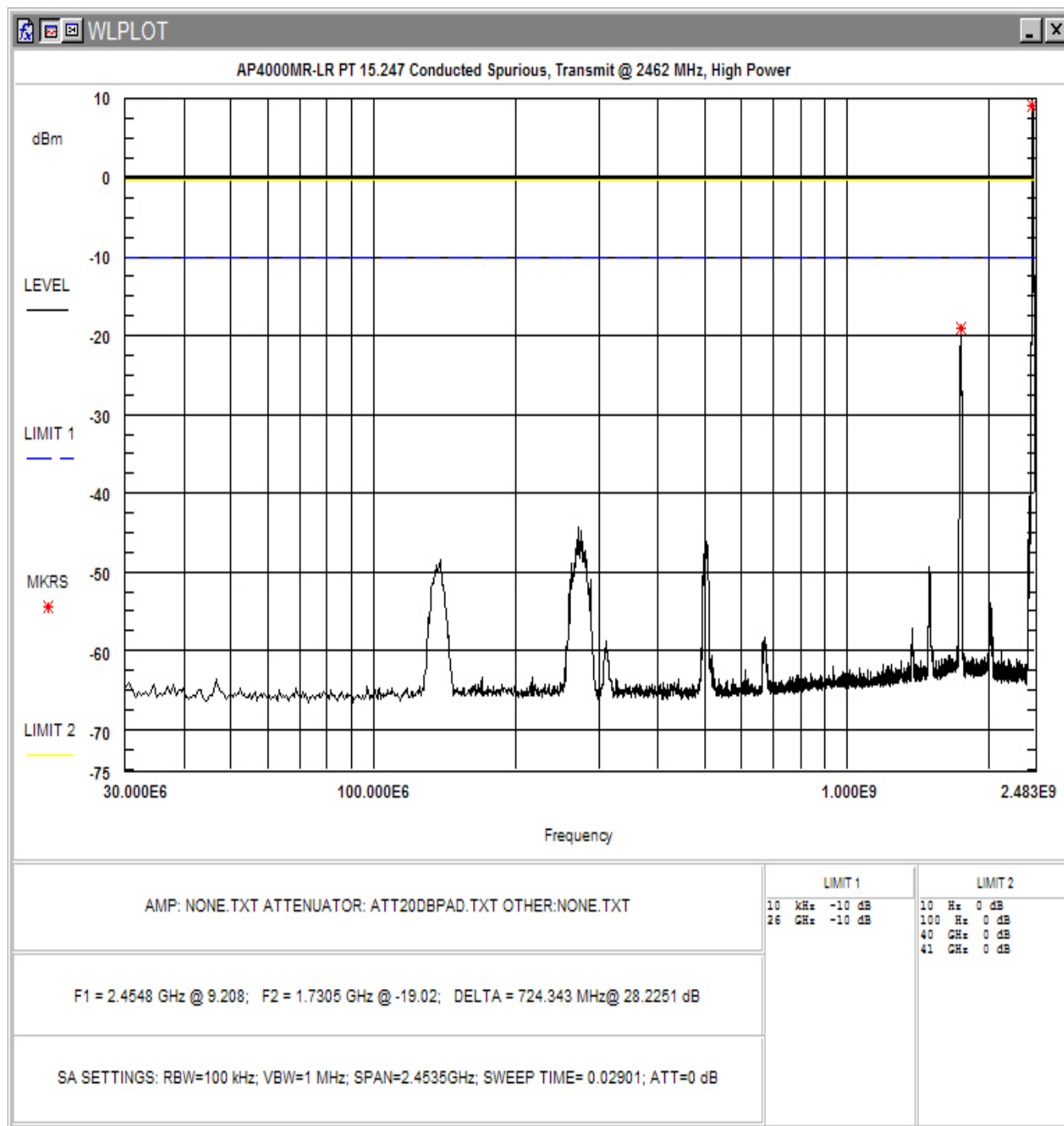
Figure 4-22. Conducted Spurious Emissions, High Power: High Channel 30 – 2483MHz
