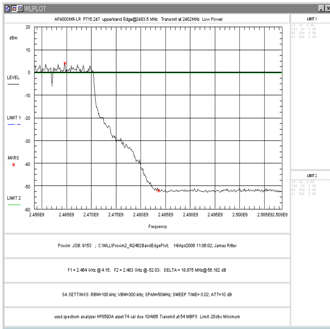
Figure 4-13. Conducted Spurious Emissions, Low Power: High Channel Band Edge
