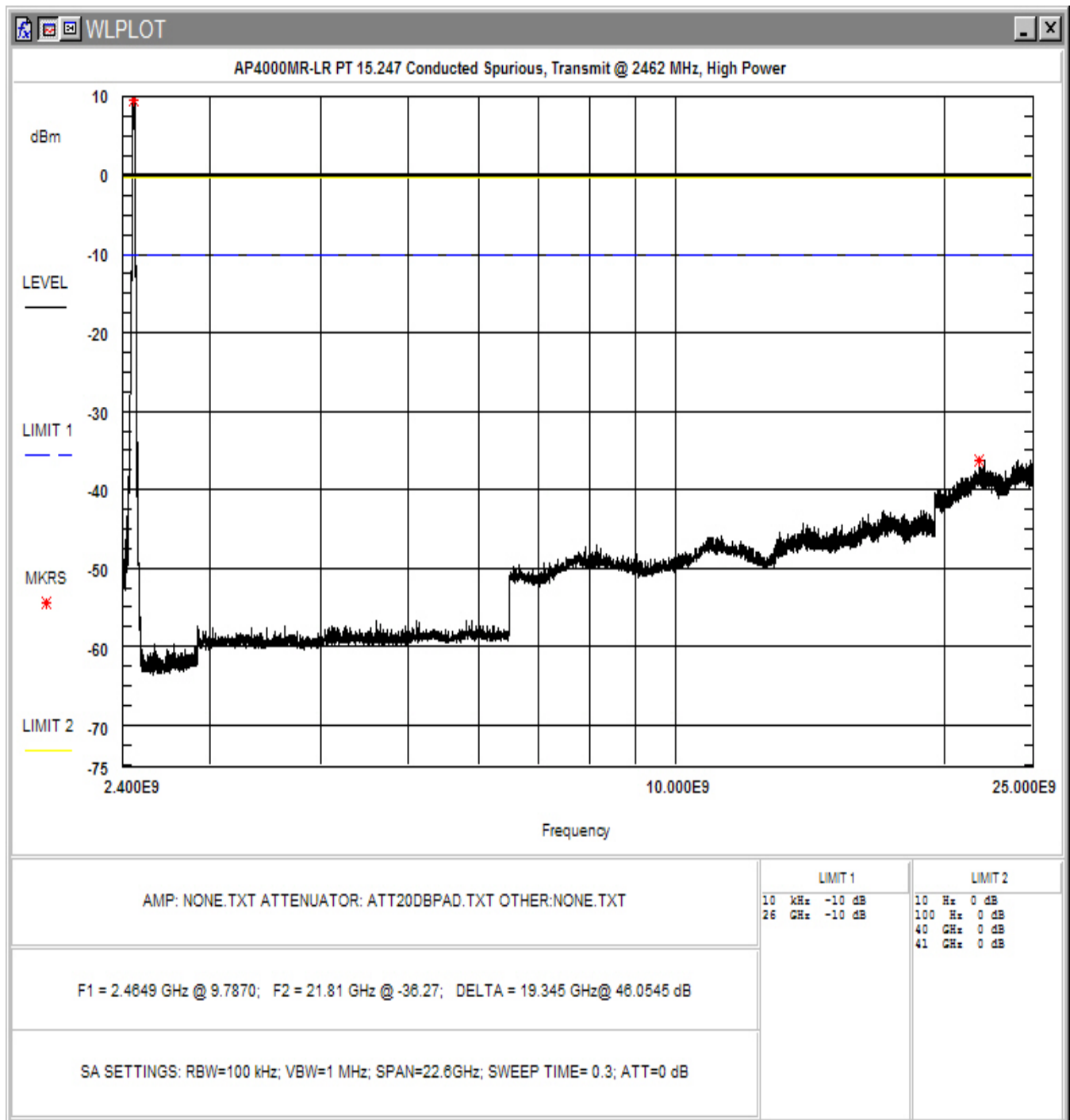
Figure 4-23. Conducted Spurious Emissions, High Power: High Channel 2.4 - 25GHz
