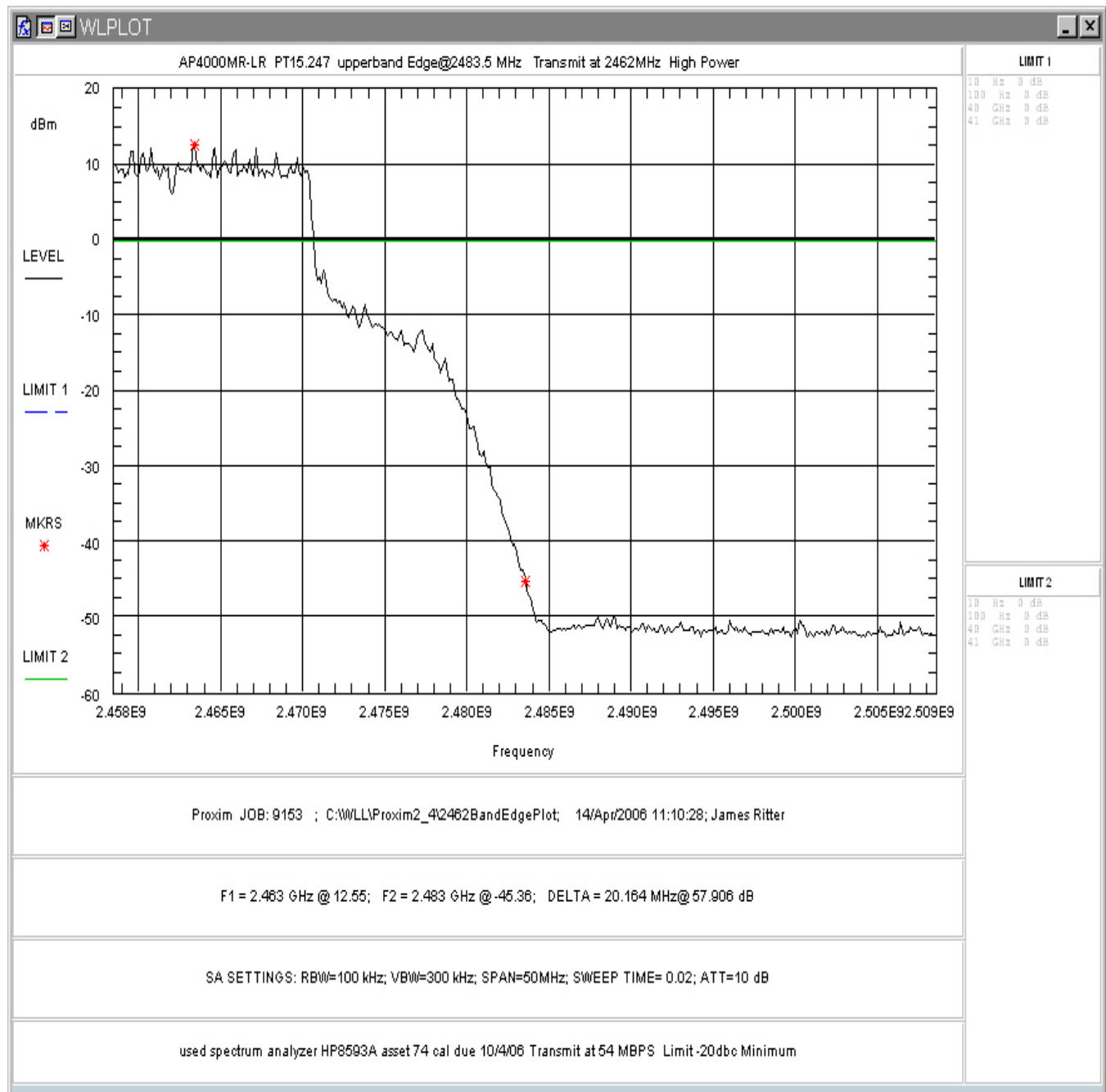
Figure 4-21. Conducted Spurious Emissions, High Power: High Channel Band Edge
