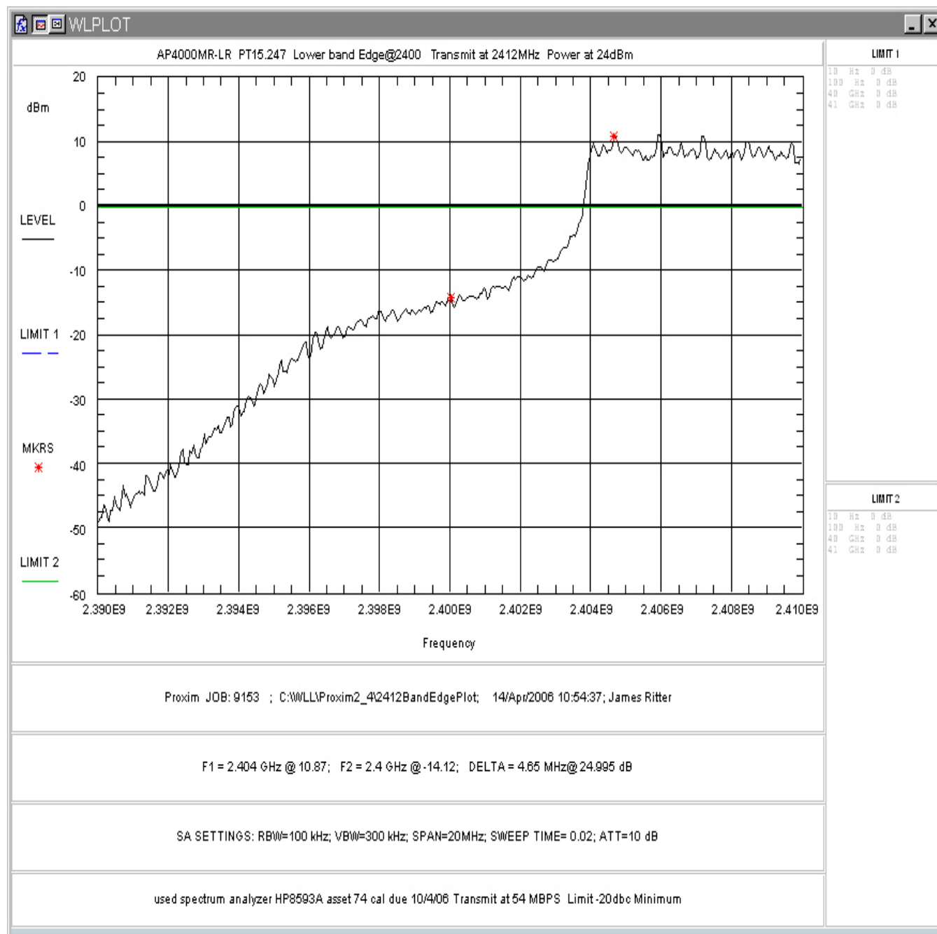
Figure 4-16. Conducted Spurious Emissions, High Power: Low Channel Band Edge
