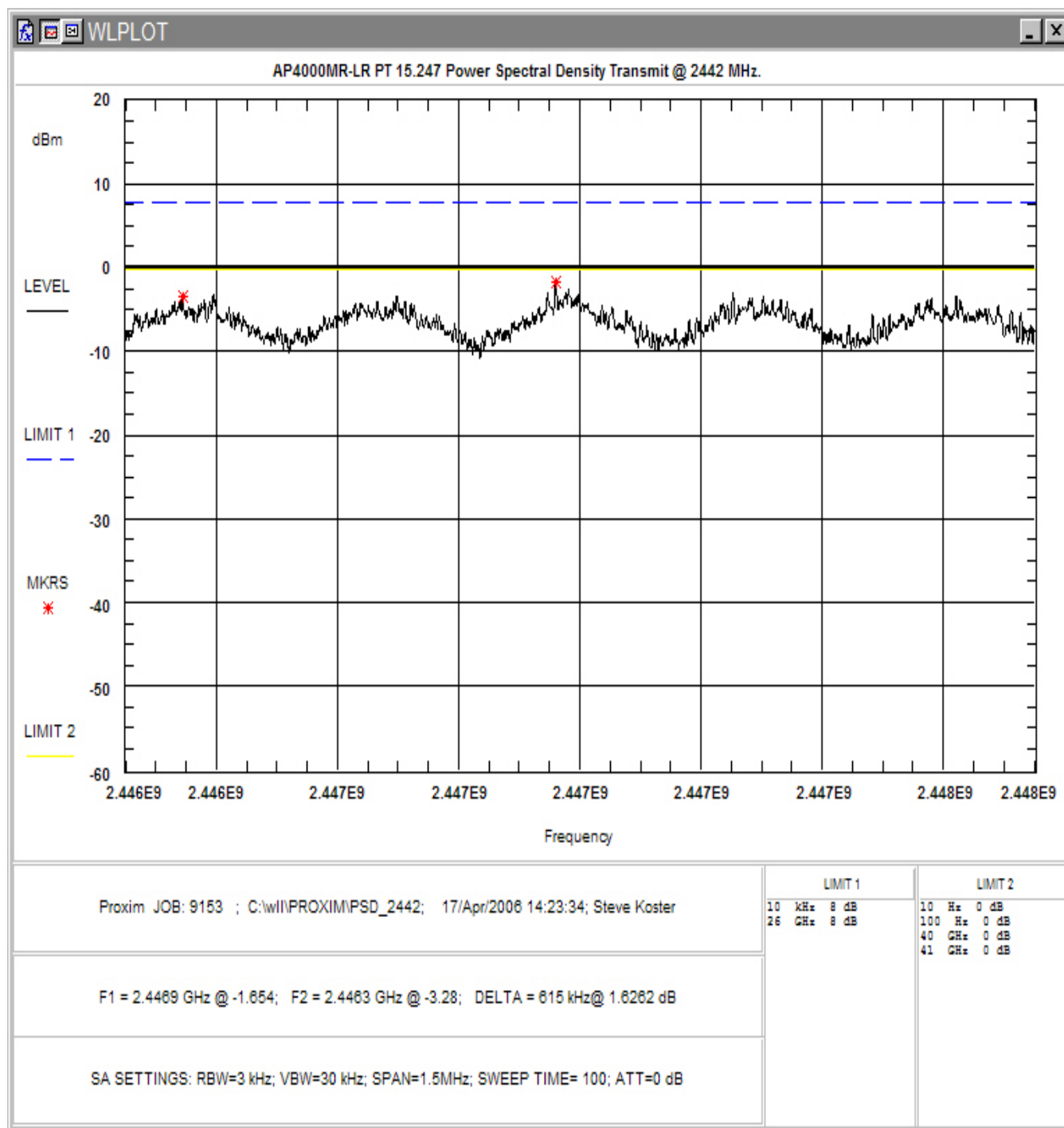
Figure 4-6: Power Spectral Density, Mid Channel
