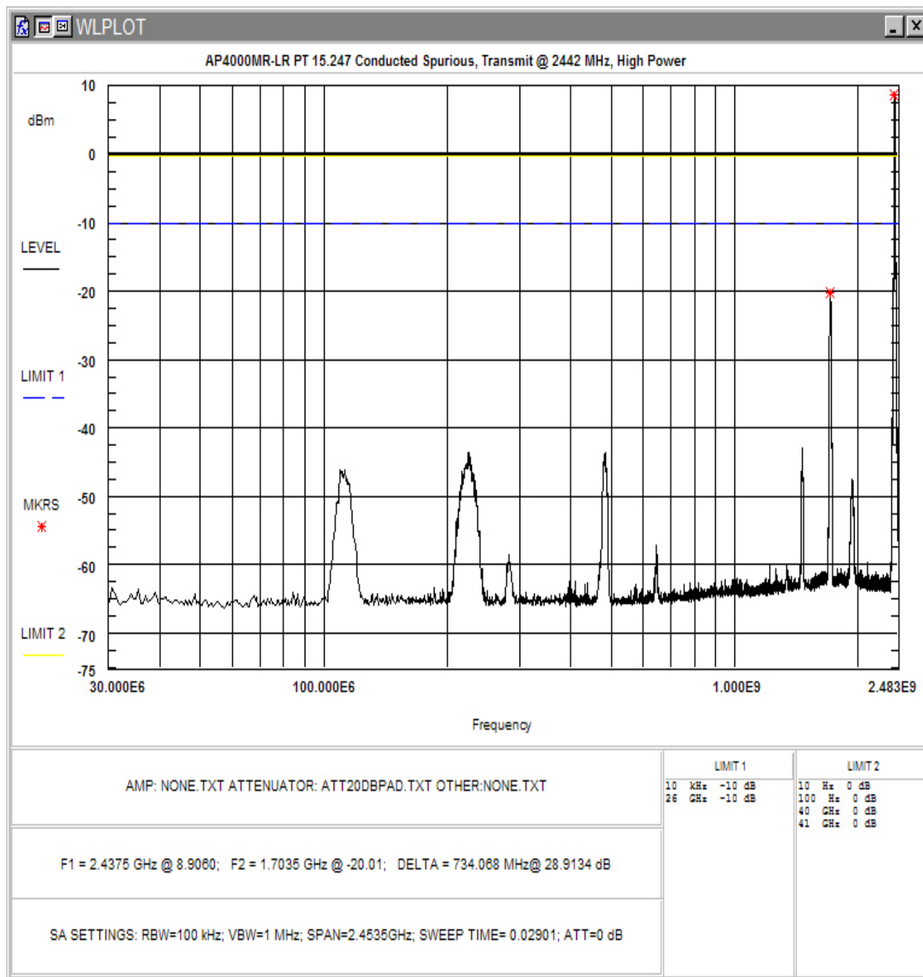
Figure 4-19. Conducted Spurious Emissions, High Power: Mid Channel 30 – 2483MHz
