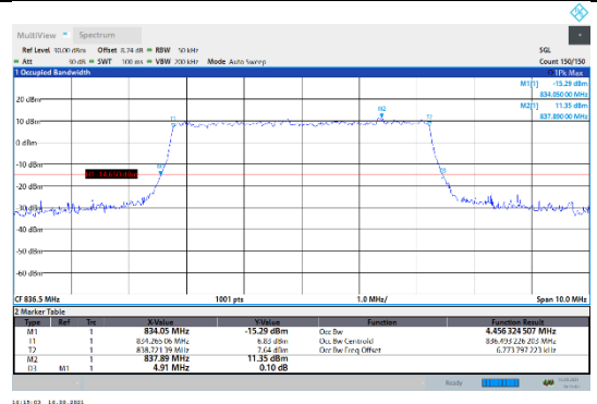
N5-15kHz-5MHz-CP-QPSK-Mid-Outer_Full---PASS
