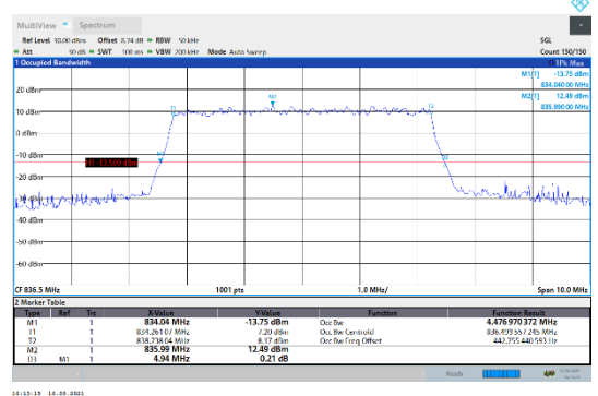
N5-15kHz-5MHz-DFT-64QAM-Mid-Outer_Full---PASS
