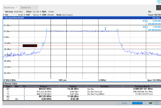
N5-15kHz-5MHz-CP-64QAM-High-Outer Full---PASS
