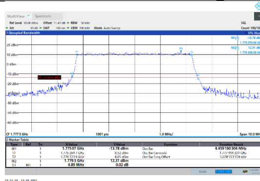
N66-15kHz-5MHz-CP-16QAM-High-Outer_Full---PASS
