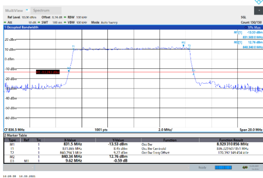
N5-15kHz-10MHz-DFT-64QAM-Mid-Outer_Full---PASS
