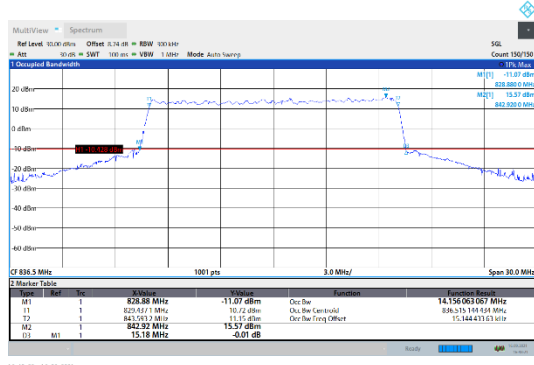
N5-15kHz-15MHz-CP-16QAM-Mid-Outer_Full---PASS
