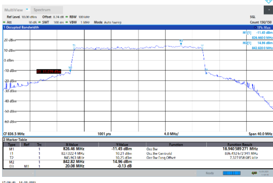
N5-15kHz-20MHz-CP-QPSK-Mid-Outer_Full---PASS
