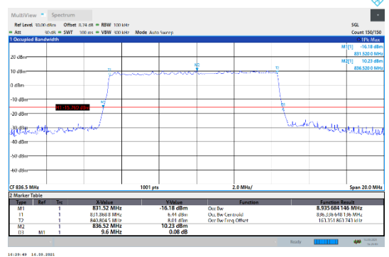
N5-15kHz-10MHz-DFT-256QAM-Mid-Outer_Full---PASS
