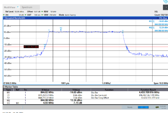
N5-15kHz-5MHz-CP-QPSK-High-Outer Full---PASS
