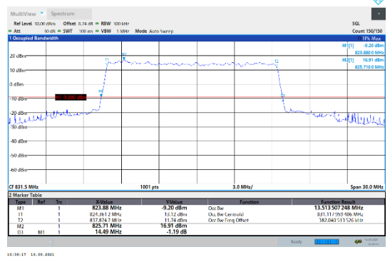
N5-15kHz-15MHz-DFT-16QAM-Low-Outer_Full---PASS
