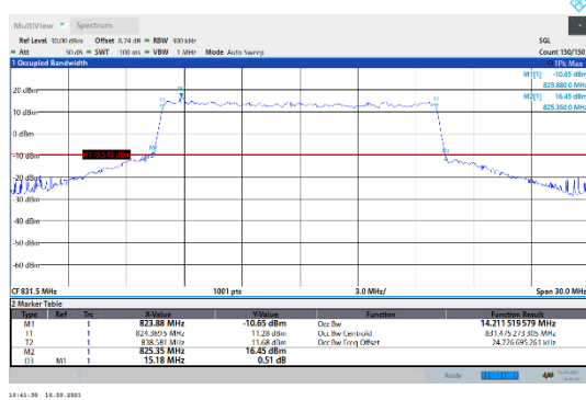
N5-15kHz-15MHz-CP-QPSK-Low-Outer_Full---PASS
