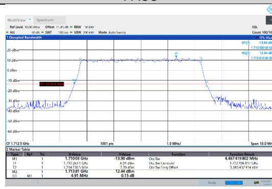
N66-15kHz-5MHz-DFT-256QAM-Low-Outer_Full---PASS
