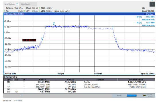
N5-15kHz-5MHz-CP-256QAM-High-Outer_Full---PASS
