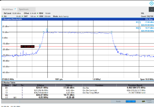
N5-15kHz-5MHz-CP-QPSK-Low-Outer_Full---PASS
