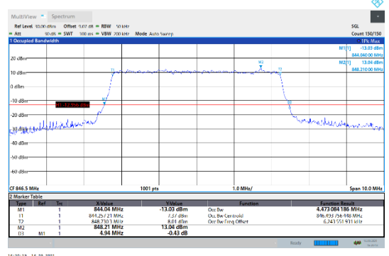
N5-15kHz-5MHz-CP-16QAM-High-Outer Full---PASS
