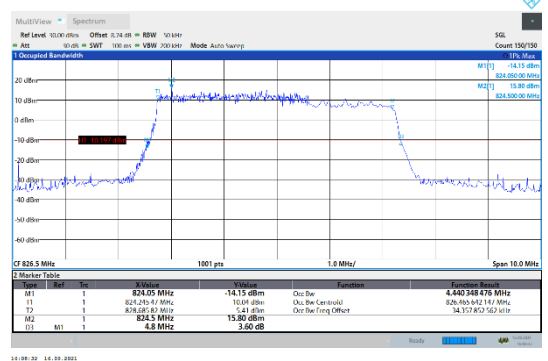
N5-15kHz-5MHz-DFT-256QAM-Low-Outer_Full---PASS
