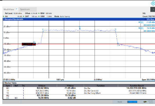
N5-15kHz-15MHz-CP-64QAM-Low-Outer_Full---PASS
