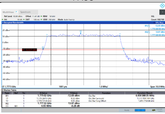
N66-15kHz-5MHz-DFT-64QAM-High-Outer_Full---PASS
