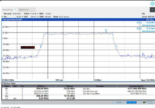
N5-15kHz-5MHz-DFT-256QAM-Mid-Outer_Full---PASS
