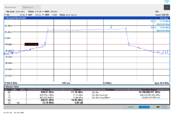
N5-15kHz-15MHz-CP-QPSK-Mid-Outer_Full---PASS
