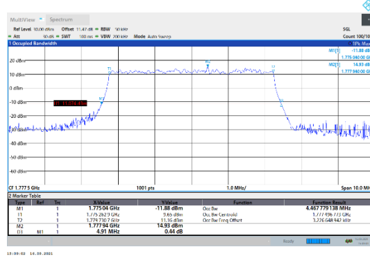
N66-15kHz-5MHz-DFT-16QAM-High-Outer_Full---PASS
