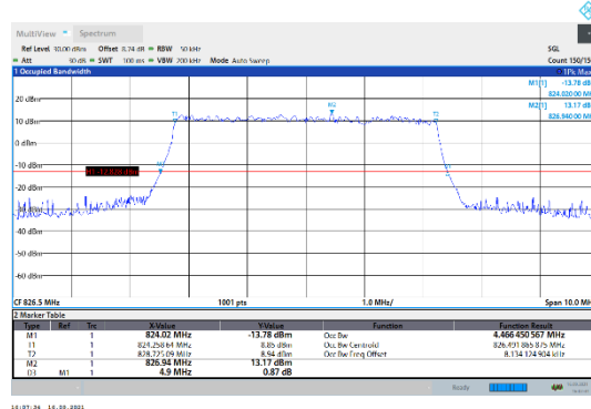
N5-15kHz-5MHz-DFT-16QAM-Low-Outer_Full---PASS
