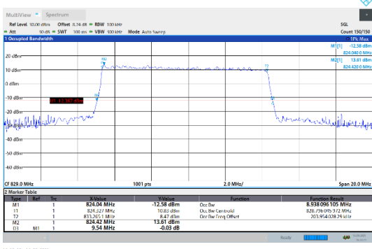
N5-15kHz-10MHz-DFT-16QAM-Low-Outer_Full---PASS
