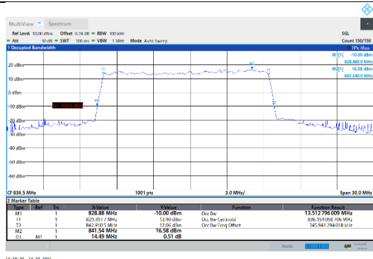
N5-15kHz-15MHz-DFT-16QAM-Mid-Outer_Full---PASS
