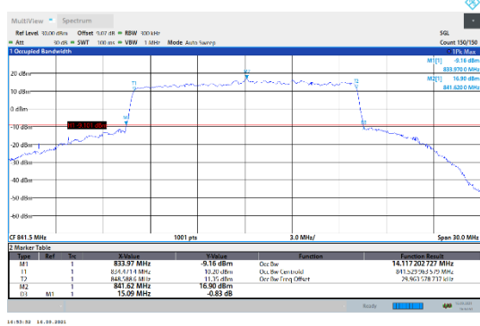
N5-15kHz-15MHz-CP-64QAM-High-Outer_Full---PASS
