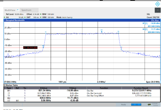
N5-15kHz-10MHz-CP-16QAM-Mid-Outer_Full---PASS
