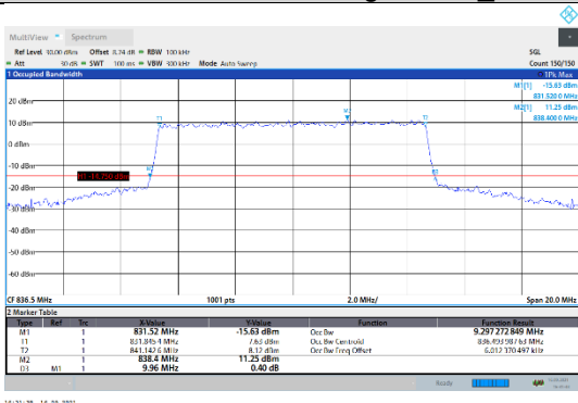
N5-15kHz-10MHz-CP-64QAM-Mid-Outer Full---PASS
