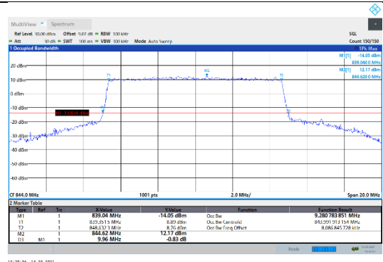
N5-15kHz-10MHz-CP-QPSK-High-Outer_Full---PASS
