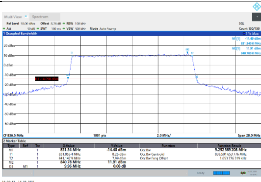
N5-15kHz-10MHz-CP-QPSK-Mid-Outer_Full---PASS
