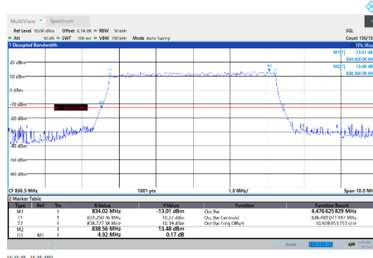
N5-15kHz-5MHz-DFT-QPSK-Mid-Outer_Full---PASS
