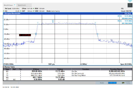
N5-15kHz-10MHz-DFT-64QAM-High-Outer_Full---PASS
