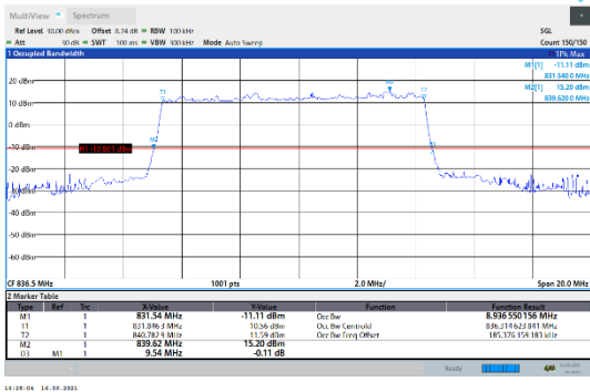
N5-15kHz-10MHz-DFT-QPSK-Mid-Outer_Full---PASS
