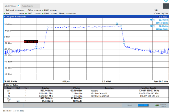
N5-15kHz-15MHz-DFT-QPSK-Mid-Outer_Full---PASS
