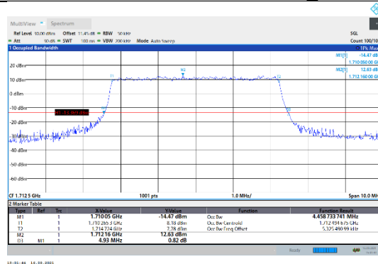
N66-15kHz-5MHz-CP-16QAM-Low-Outer_Full---PASS
