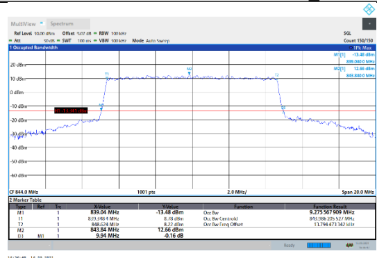
N5-15kHz-10MHz-CP-64QAM-High-Outer Full---PASS
