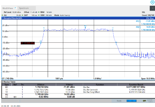
N66-15kHz-5MHz-DFT-16QAM-Mid-Outer_Full---PASS
