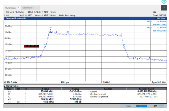
N5-15kHz-5MHz-CP-256QAM-Low-Outer Full---PASS
