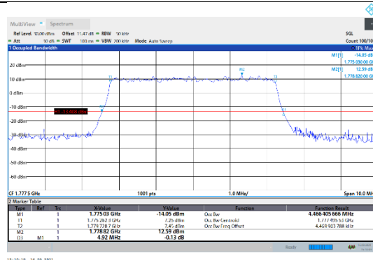
N66-15kHz-5MHz-DFT-256QAM-High-Outer_Full---PASS
