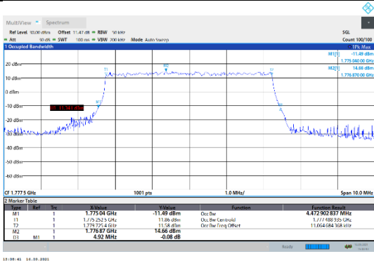
N66-15kHz-5MHz-DFT-QPSK-High-Outer_Full---PASS
