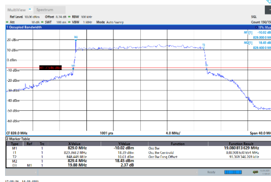
N5-15kHz-20MHz-CP-QPSK-High-Outer_Full---PASS
