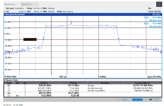
N5-15kHz-10MHz-DFT-QPSK-High-Outer_Full---PASS
