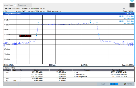
N5-15kHz-10MHz-DFT-16QAM-Mid-Outer_Full---PASS
