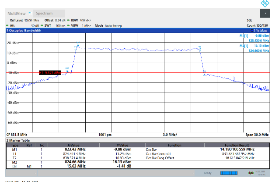
N5-15kHz-15MHz-CP-16QAM-Low-Outer_Full---PASS
