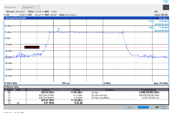
N5-15kHz-5MHz-CP-16QAM-Low-Outer_Full---PASS
