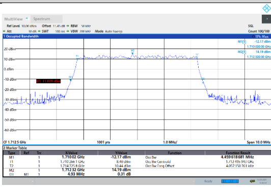
N66-15kHz-5MHz-DFT-64QAM-Low-Outer_Full---PASS
