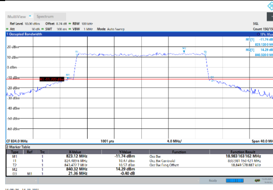
N5-15kHz-20MHz-CP-QPSK-Low-Outer_Full---PASS
