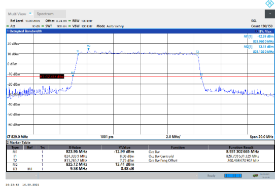
N5-15kHz-10MHz-DFT-64QAM-Low-Outer_Full---PASS
