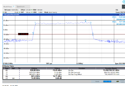
N5-15kHz-15MHz-DFT-64QAM-Mid-Outer_Full---PASS
