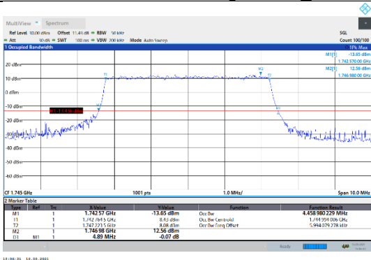
N66-15kHz-5MHz-CP-16QAM-Mid-Outer_Full---PASS
