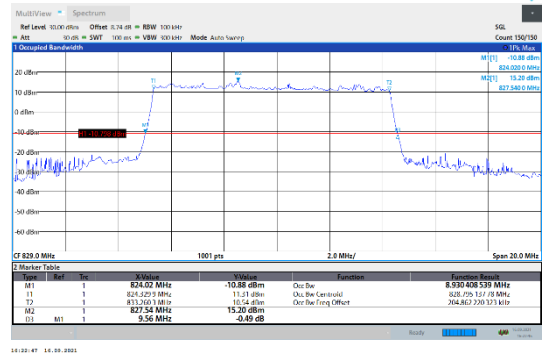
N5-15kHz-10MHz-DFT-QPSK-Low-Outer_Full---PASS
