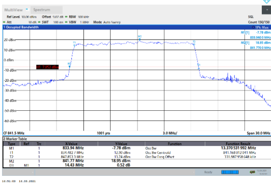
N5-15kHz-15MHz-DFT-QPSK-High-Outer_Full---PASS
