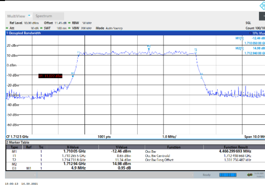
N66-15kHz-5MHz-DFT-16QAM-Low-Outer_Full---PASS
