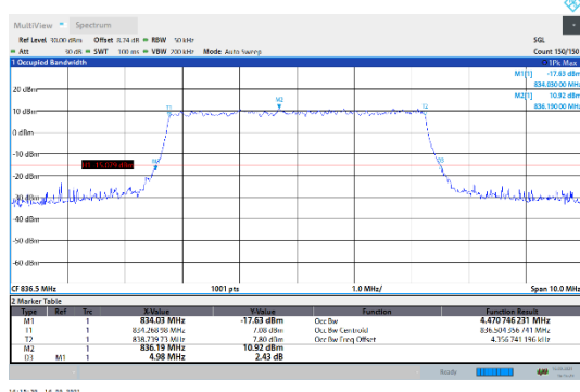
N5-15kHz-5MHz-CP-16QAM-Mid-Outer Full---PASS
