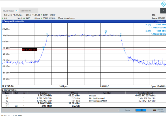
N66-15kHz-5MHz-DFT-256QAM-Mid-Outer_Full---PASS
