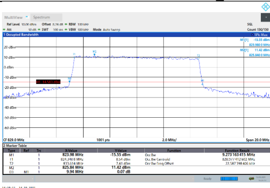
N5-15kHz-10MHz-CP-16QAM-Low-Outer_Full---PASS
