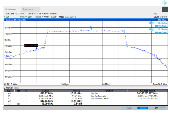
N5-15kHz-15MHz-CP-16QAM-High-Outer_Full---PASS
