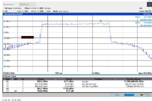
N5-15kHz-20MHz-DFT-QPSK-Mid-Outer_Full---PASS
