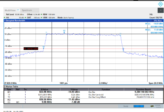
N5-15kHz-10MHz-CP-64QAM-Low-Outer_Full---PASS
