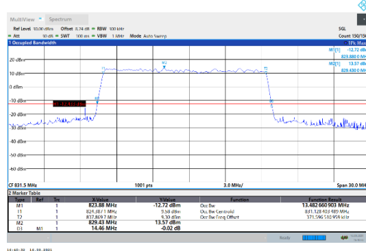
N5-15kHz-15MHz-DFT-256QAM-Low-Outer_Full---PASS
