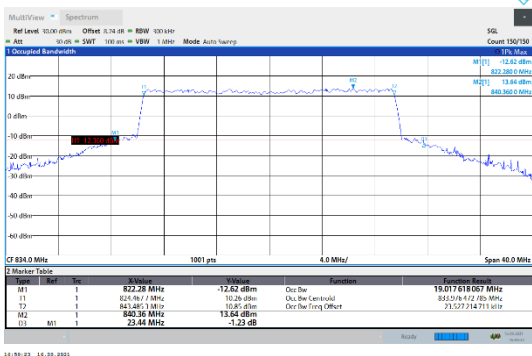
N5-15kHz-20MHz-CP-16QAM-Low-Outer_Full---PASS
