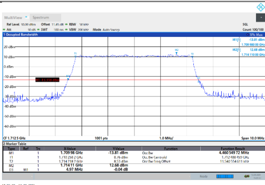
N66-15kHz-5MHz-CP-QPSK-Low-Outer_Full---PASS
