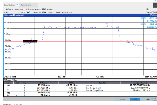
N5-15kHz-20MHz-CP-64QAM-Low-Outer_Full---PASS
