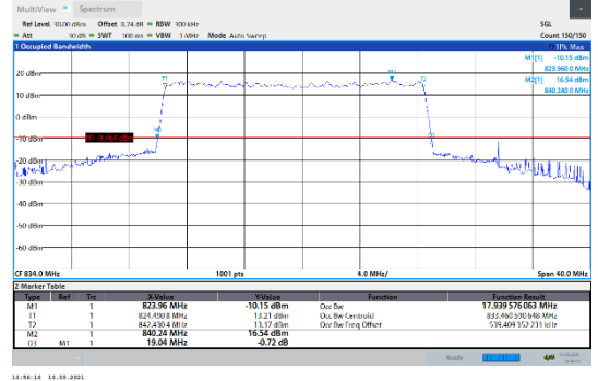
N5-15kHz-20MHz-DFT-QPSK-Low-Outer_Full---PASS
