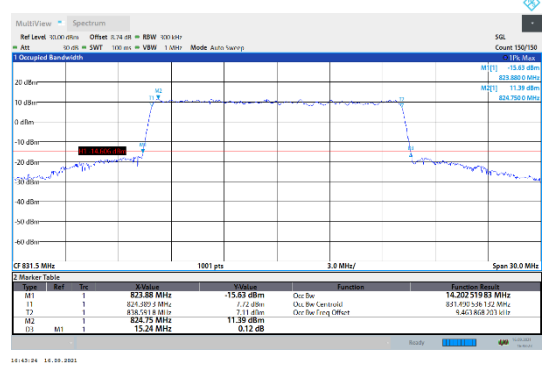
N5-15kHz-15MHz-CP-256QAM-Low-Outer_Full---PASS
