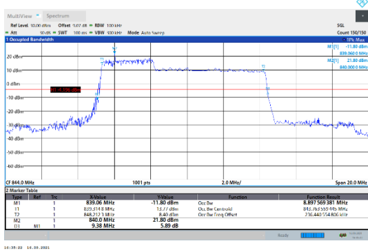
N5-15kHz-10MHz-DFT-256QAM-High-Outer_Full---PASS
