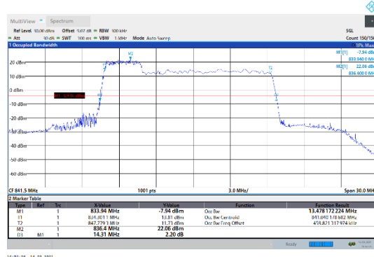
N5-15kHz-15MHz-DFT-256QAM-High-Outer_Full---PASS
