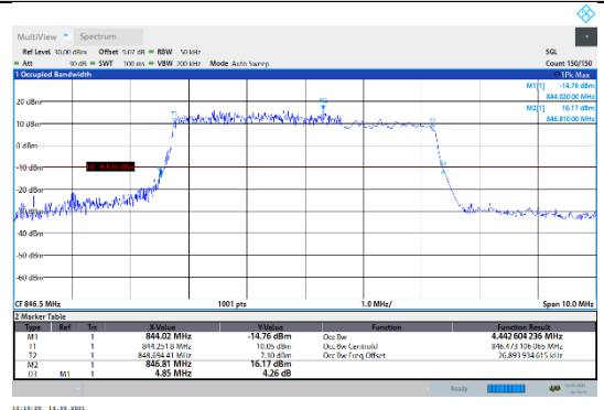
N5-15kHz-5MHz-DFT-256QAM-High-Outer_Full---PASS
