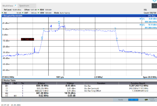
N5-15kHz-10MHz-CP-256QAM-High-Outer_Full---PASS
