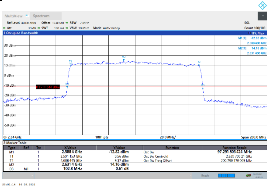
N41-30kHz-100MHz-CP-256QAM-High-Outer_Full---PASS
