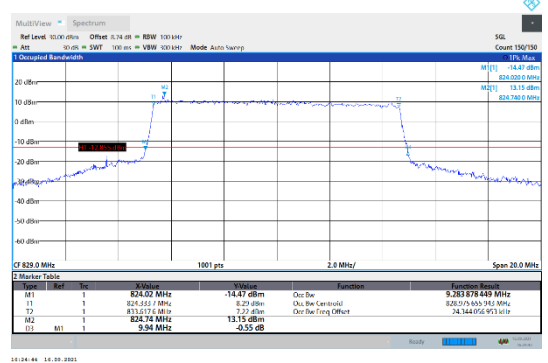
N5-15kHz-10MHz-CP-QPSK-Low-Outer_Full---PASS
