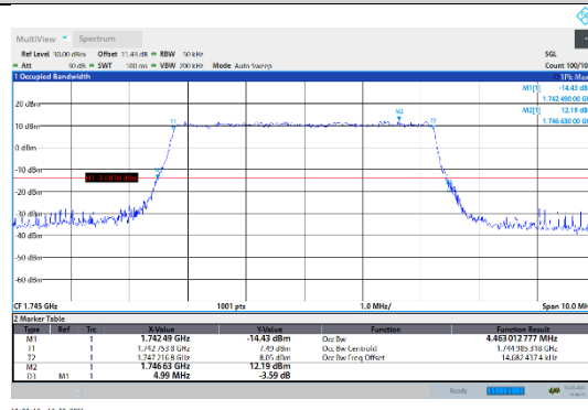
N66-15kHz-5MHz-CP-QPSK-Mid-Outer_Full---PASS
