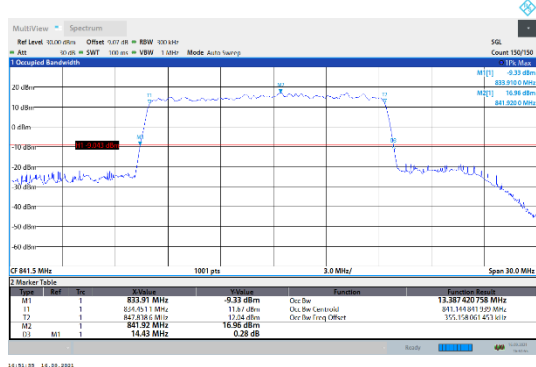
N5-15kHz-15MHz-DFT-64QAM-High-Outer_Full---PASS
