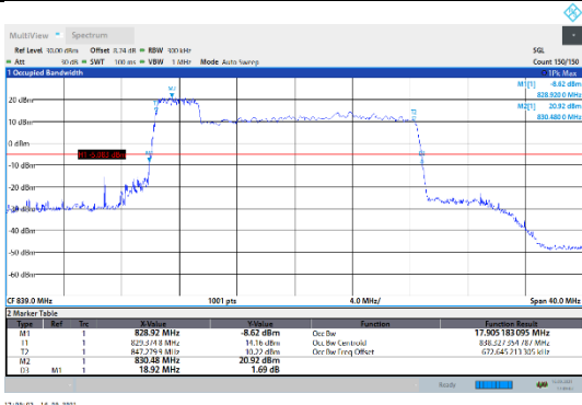
N5-15kHz-20MHz-DFT-256QAM-High-Outer_Full---PASS
