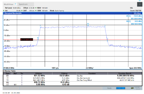
N5-15kHz-10MHz-CP-256QAM-Mid-Outer_Full---PASS
