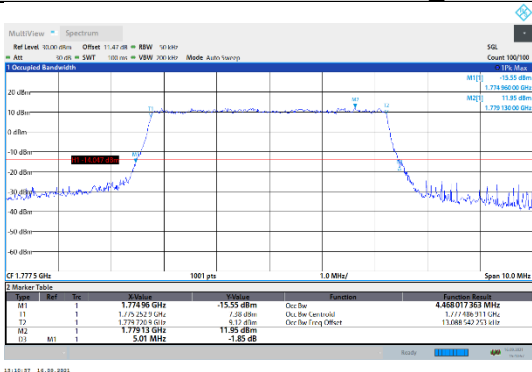
N66-15kHz-5MHz-CP-QPSK-High-Outer_Full---PASS
