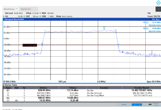
N5-15kHz-15MHz-DFT-256QAM-Mid-Outer_Full---PASS
