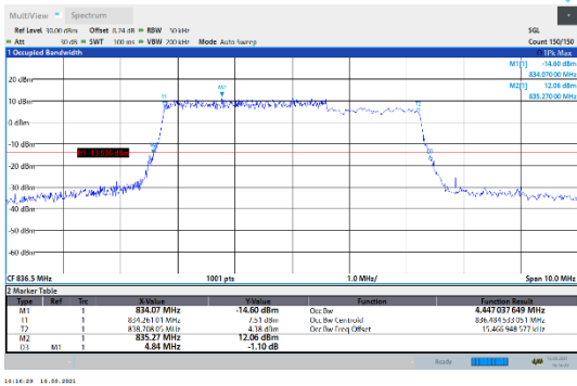
N5-15kHz-5MHz-CP-256QAM-Mid-Outer_Full---PASS
