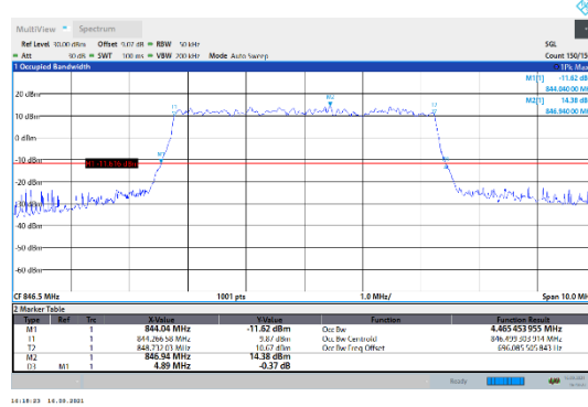
N5-15kHz-5MHz-DFT-16QAM-High-Outer_Full---PASS
