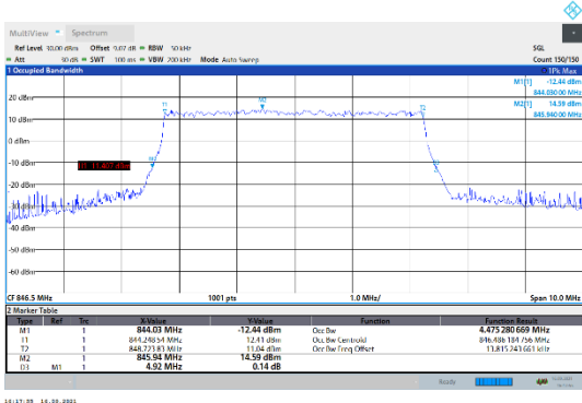
N5-15kHz-5MHz-DFT-QPSK-High-Outer_Full---PASS
