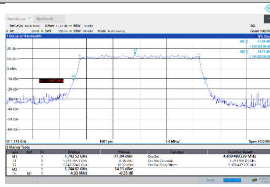
N66-15kHz-5MHz-DFT-64QAM-Mid-Outer_Full---PASS
