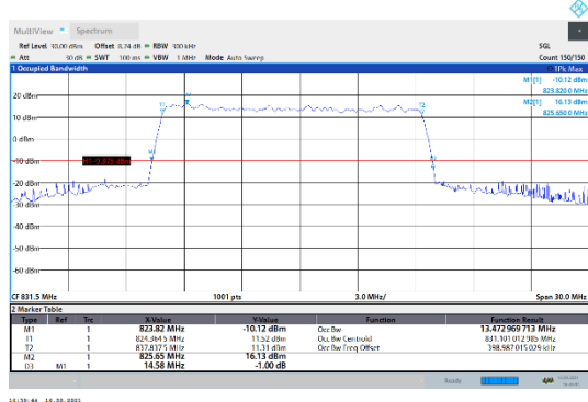
N5-15kHz-15MHz-DFT-64QAM-Low-Outer_Full---PASS
