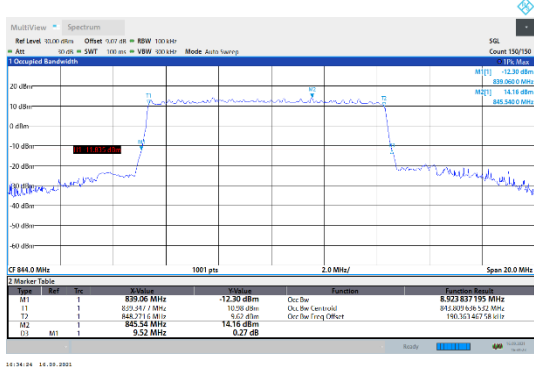
N5-15kHz-10MHz-DFT-16QAM-High-Outer_Full---PASS
