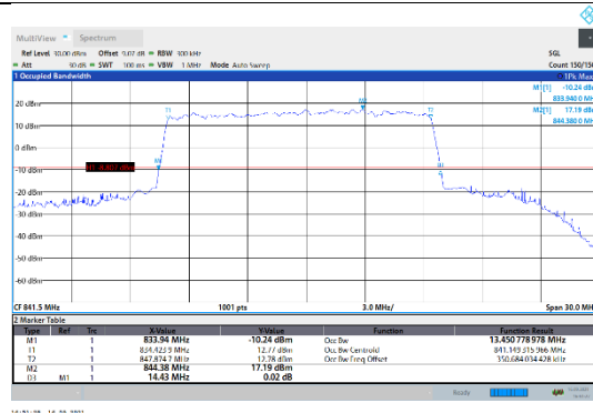
N5-15kHz-15MHz-DFT-16QAM-High-Outer_Full---PASS
