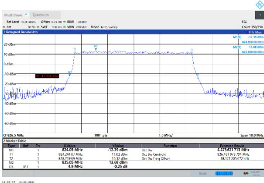
N5-15kHz-5MHz-DFT-QPSK-Low-Outer_Full---PASS
