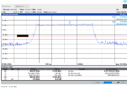
N5-15kHz-5MHz-DFT-16QAM-Mid-Outer_Full---PASS
