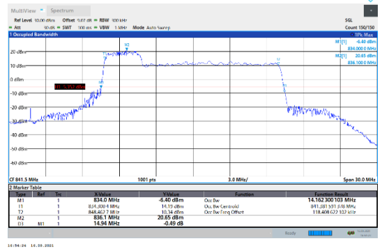
N5-15kHz-15MHz-CP-256QAM-High-Outer_Full---PASS
