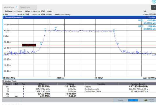
N5-15kHz-5MHz-CP-64QAM-Low-Outer Full---PASS
