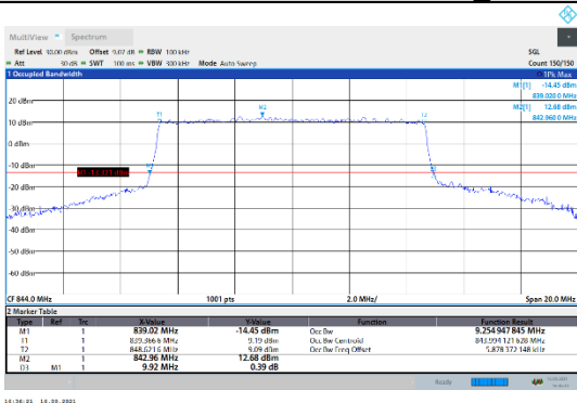
N5-15kHz-10MHz-CP-16QAM-High-Outer_Full---PASS
