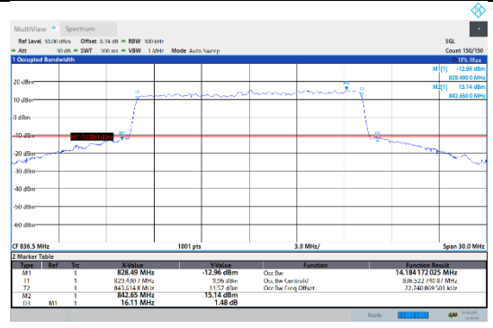
N5-15kHz-15MHz-CP-64QAM-Mid-Outer_Full---PASS
