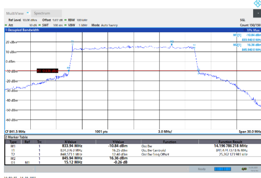
N5-15kHz-15MHz-CP-QPSK-High-Outer_Full---PASS
