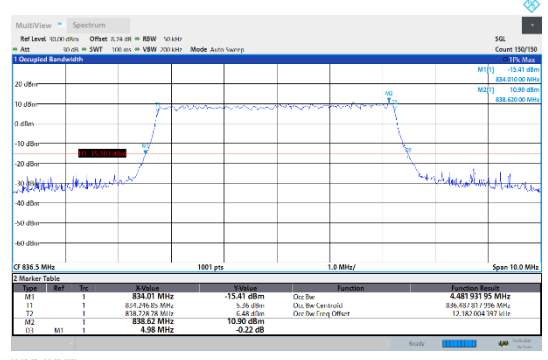
N5-15kHz-5MHz-CP-64QAM-Mid-Outer Full---PASS
