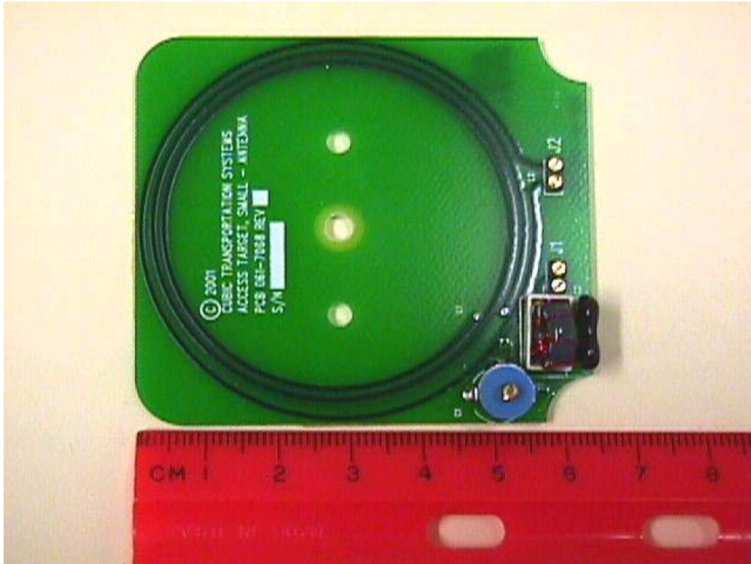
PCB ANTENNA SIDE
