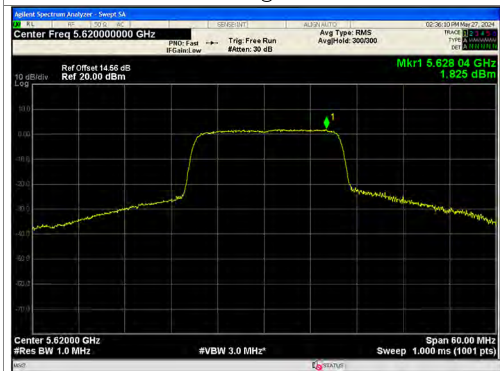
PSD NVNT ax40 242@61 5630MHz Ant2
