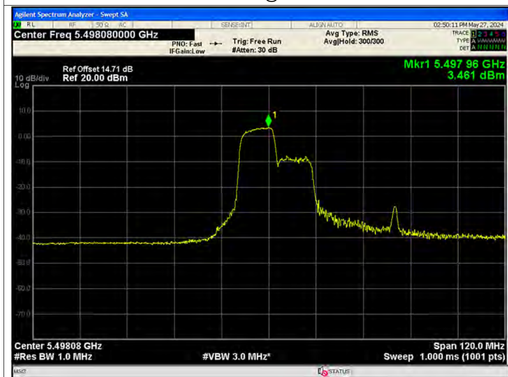
PSD NVNT ax80 106@53 5530MHz Ant1
