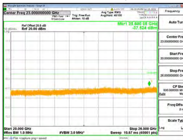
Band7-20G-26G / 10MHz / High CH / 16QAM
