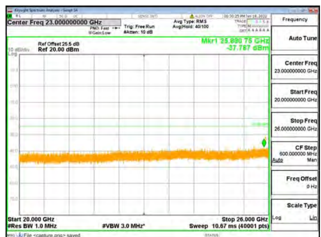
Band7-20G-26G / 10MHz / Low CH / 64QAM
