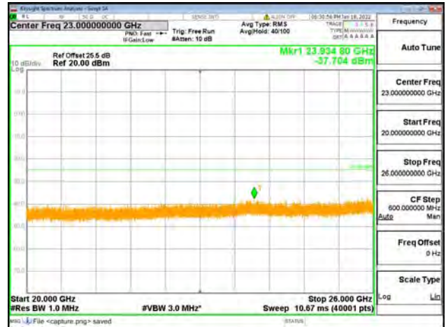
Band7-20G-26G / 10MHz / Mid CH / 16QAM
