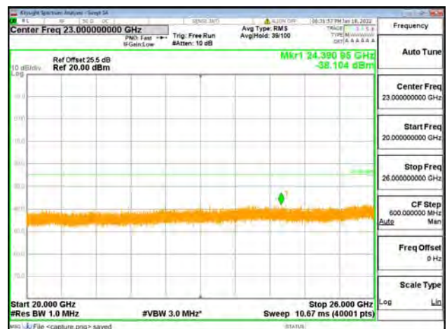
Band7-20G-26G / 10MHz / Mid CH / 64QAM
