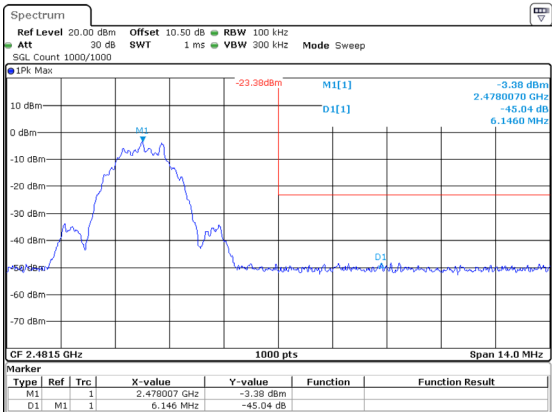
BLE_2M_High_Channel
