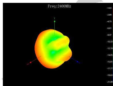
Phi = 90 freq=2400MHz
