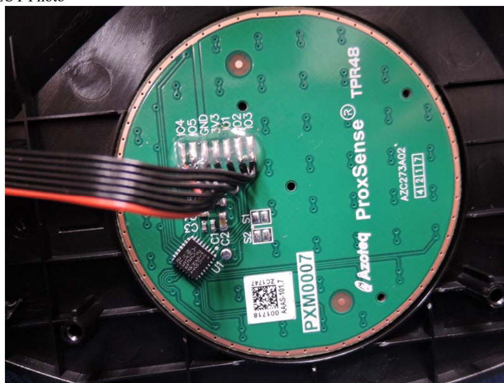
(7) EUT Photo
