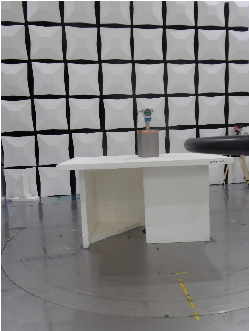
Test setup semi anechoic chamber (9 kHz to 30 MHz)
