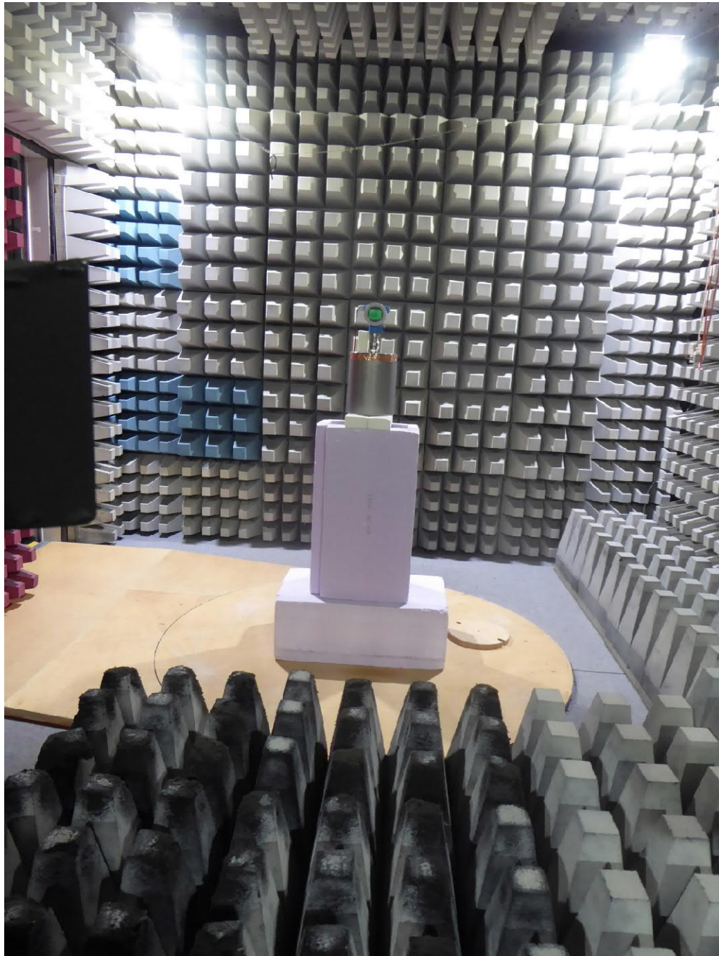
Test setup fully anechoic chamber with (12 GHz to 26.5 GHz)
