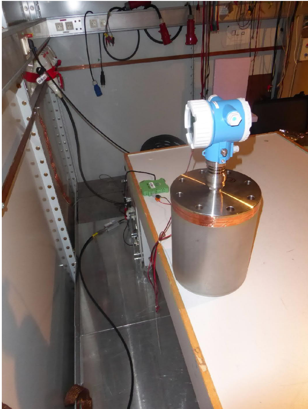
Test setup AC powerline conductec emissions
