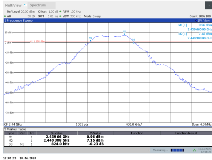
BLE_1M_Ant0_2440
