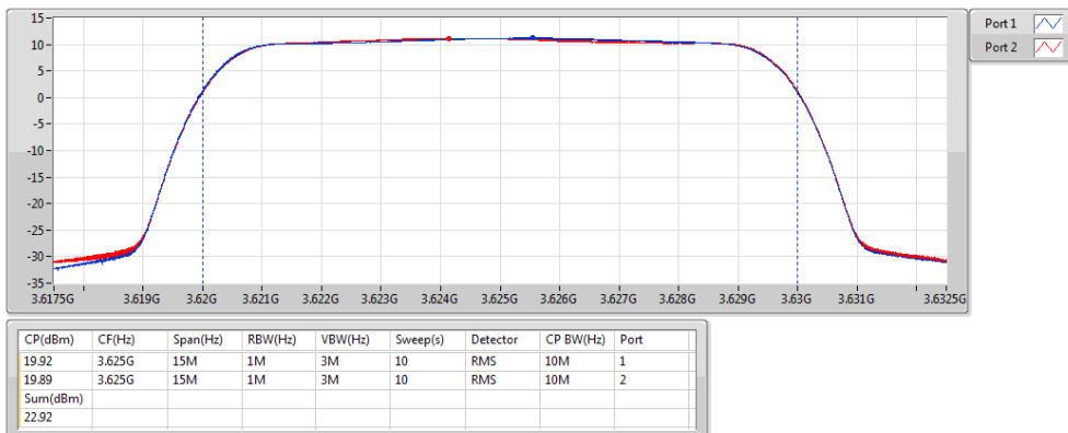
Band 48_LTE_10MHz_Nss1,16QAM_2TX 3625MHz_16QAM_RB 50,#RB 0
