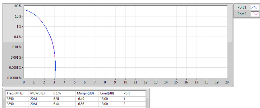
Band 48_LTE_20MHz_Nss1,64QAM_2TX 3690MHz_64QAM_RB 100,#RB 0
