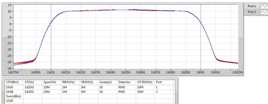
Band 48_LTE_10MHz_Nss1,16QAM_2TX 3625MHz_16QAM_RB 50,#RB 0
