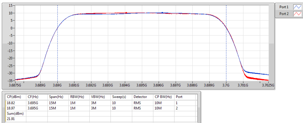
Band 48_LTE_10MHz_Nss1,64QAM_2TX 3695MHz_64QAM_RB 50,#RB 0
