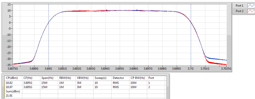
Band 48_LTE_10MHz_Nss1,64QAM_2TX 3695MHz_64QAM_RB 50,#RB 0
