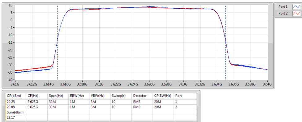
Band 48_LTE_20MHz_Nss1,16QAM_2TX 3625MHz_16QAM_RB 100,#RB 0
