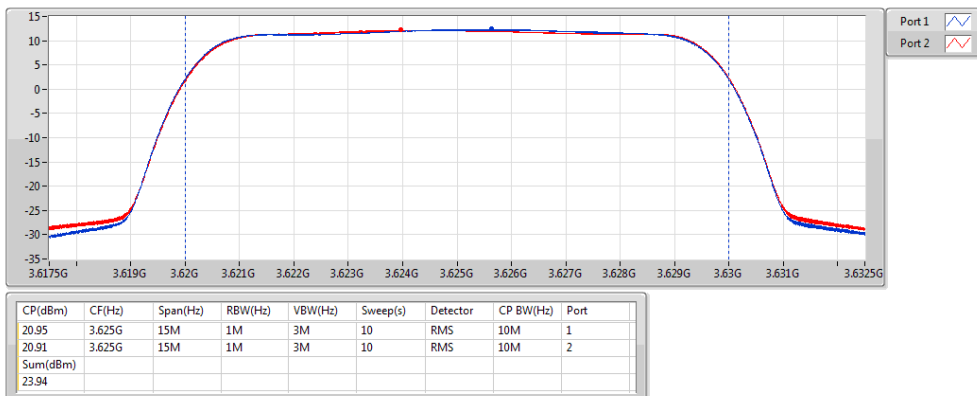
Band 48_LTE_10MHz_Nss1,QPSK_2TX 3625MHz_QPSK_RB 50,#RB 0
