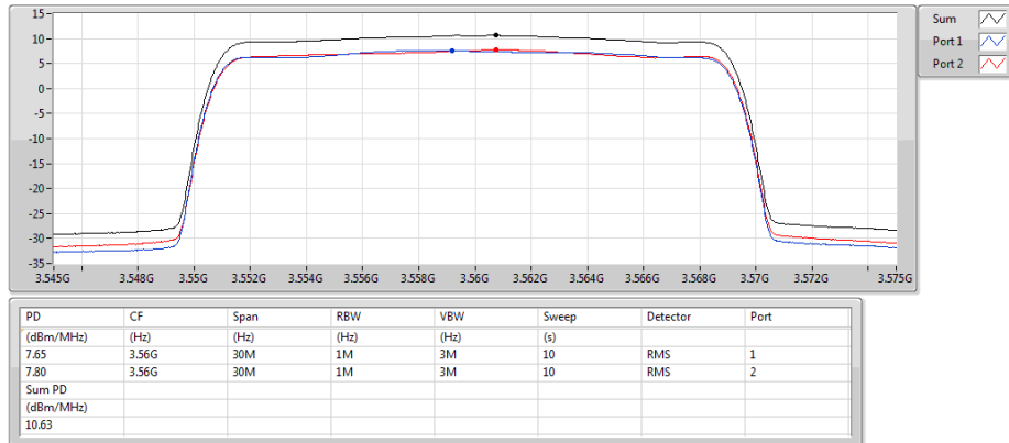
Band 48_LTE_20MHz_Nss1,64QAM_2TX 3560MHz_64QAM_RB 100,#RB 0
