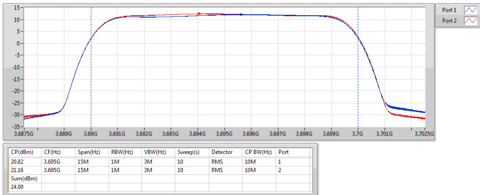
Band 48_LTE_10MHz_Nss1,QPSK_2TX 3695MHz_QPSK_RB 50,#RB 0
