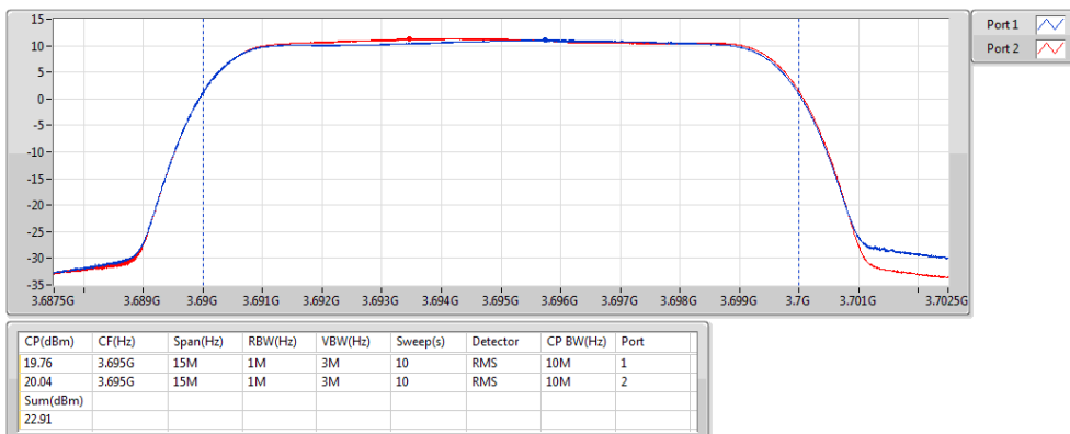
Band 48_LTE_10MHz_Nss1,16QAM_2TX 3695MHz_16QAM_RB 50,#RB 0
