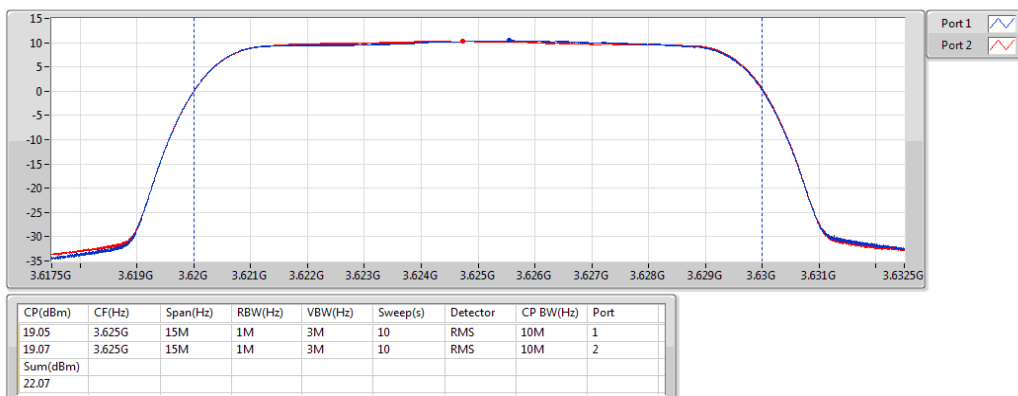
Band 48_LTE_10MHz_Nss1,64QAM_2TX 3625MHz_64QAM_RB 50,#RB 0
