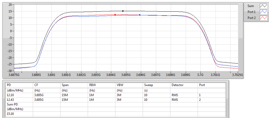
Band 48_LTE_10MHz_Nss1,QPSK_2TX 3695MHz_QPSK_RB 50,#RB 0
