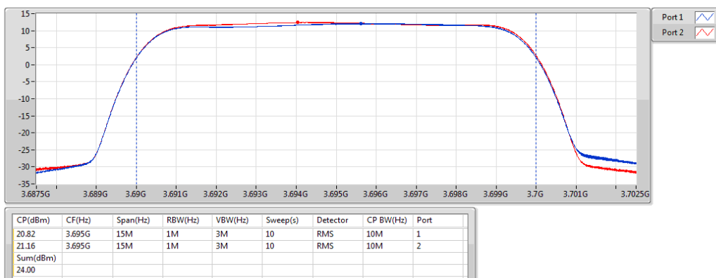
Band 48_LTE_10MHz_Nss1,QPSK_2TX 3695MHz_QPSK_RB 50,#RB 0
