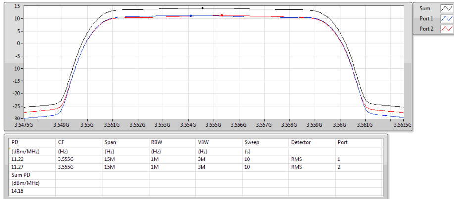
Band 48_LTE_10MHz_Nss1,16QAM_2TX 3555MHz_16QAM_RB 50,#RB 0
