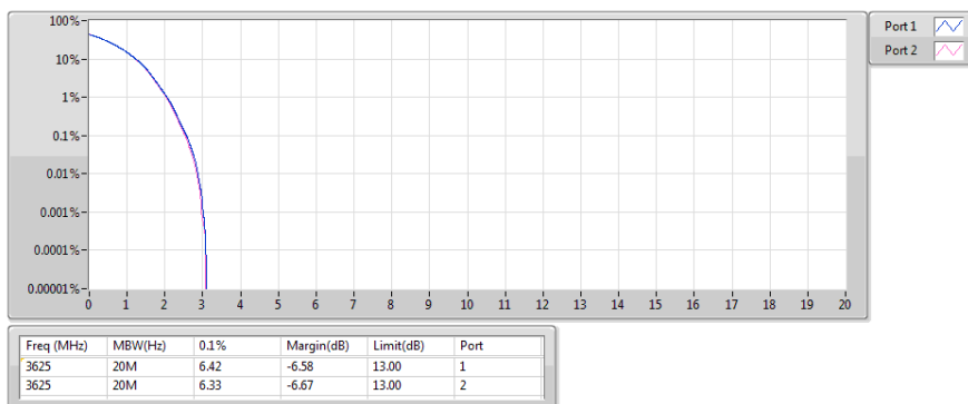
Band 48_LTE_20MHz_Nss1,64QAM_2TX 3625MHz_64QAM_RB 100,#RB 0
