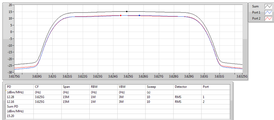
Band 48_LTE_10MHz_Nss1,QPSK_2TX 3625MHz_QPSK_RB 50,#RB 0
