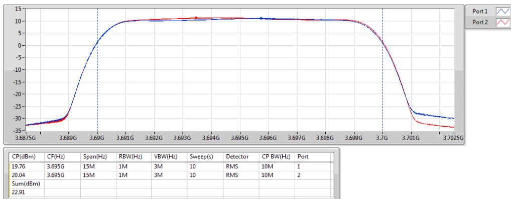
Band 48_LTE_10MHz_Nss1,16QAM_2TX 3695MHz_16QAM_RB 50,#RB 0
