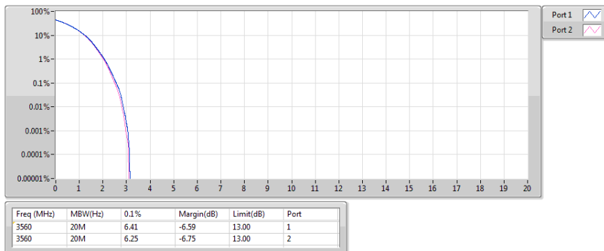
Band 48_LTE_20MHz_Nss1,64QAM_2TX 3560MHz_64QAM_RB 100,#RB 0
