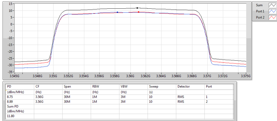
Band 48_LTE_20MHz_Nss1,16QAM_2TX 3560MHz_16QAM_RB 100,#RB 0
