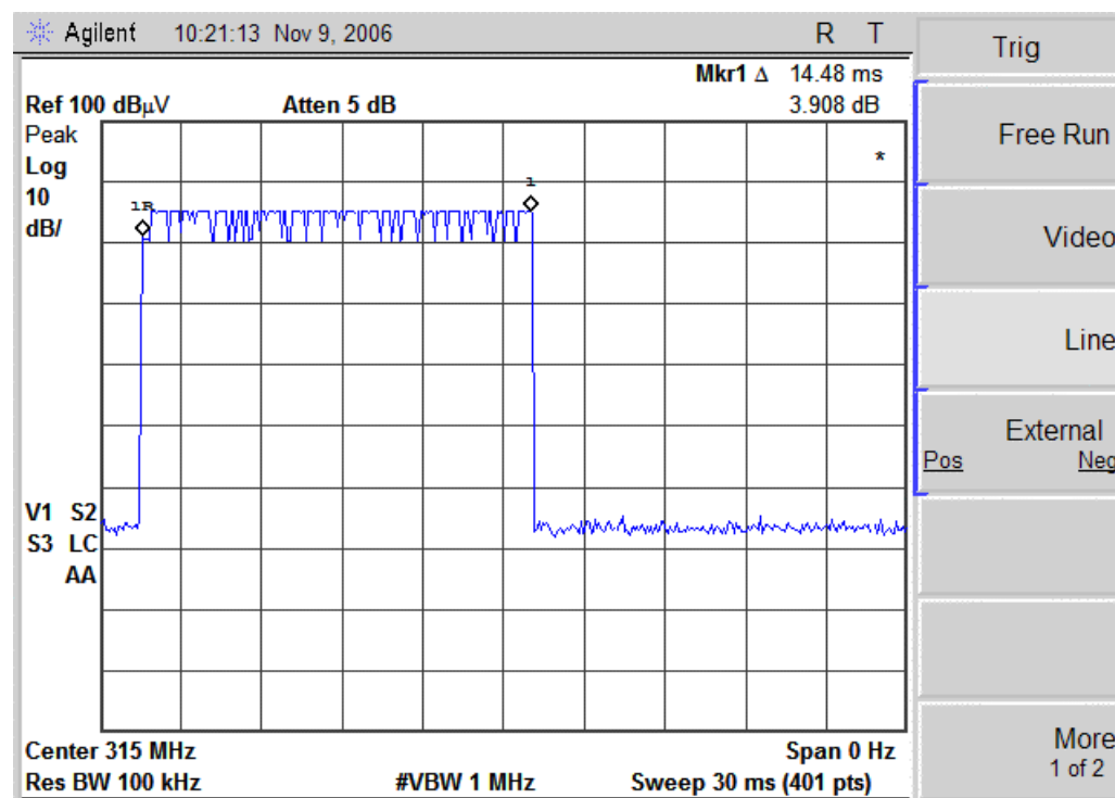
Figure 1. normal transmission
