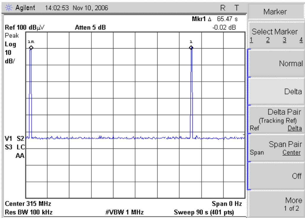
Figure 4. Transmission interval
