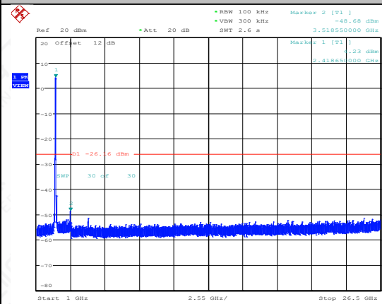
11N40MIMO-Ant2-2422-1000~26500-PASS
