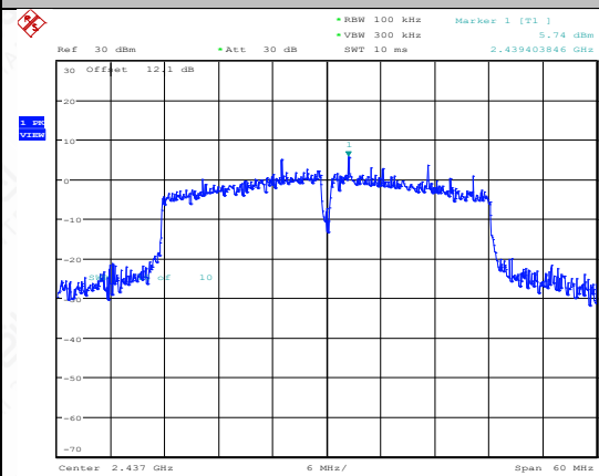
11N40MIMO-Ant2-2437-0~Reference-PASS
