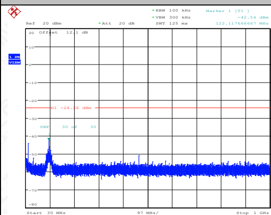
11N40MIMO-Ant2-2437-30~1000-PASS
