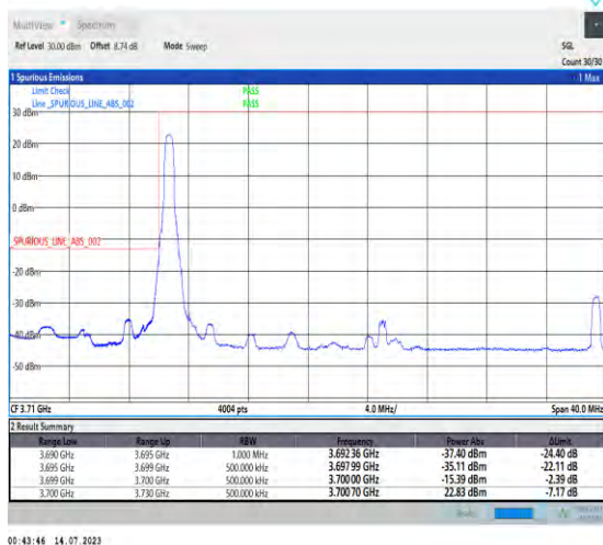
1-N77-3700-3980-PC1.5-30-30-L-4-CP-QPSK-Edge_1RB_Left-1@0-Ant3-1--PASS-see graph
