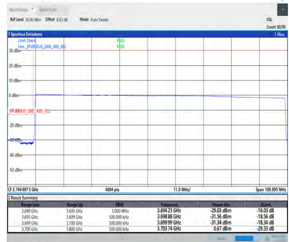
1-N77-3700-3980-PC1-30-100-L-6-CP-QPSK-Outer_Full-273@0-Ant3-1--PASS-see graph
