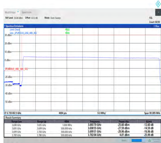
1-N77-3700-3980-PC1.5-30-80-L-3-DFT-PI2BPSK-Outer_Full-100@0-Ant3-1--PASS-see graph
