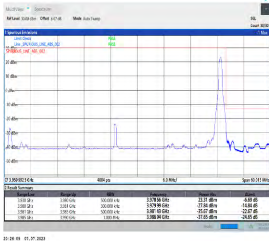
1-N77-3700-3980-PC1.5-30-50-H-2-DFT-PI2BPSK-Edge_1RB_Right-1@132-Ant3-1--PASS-see graph
