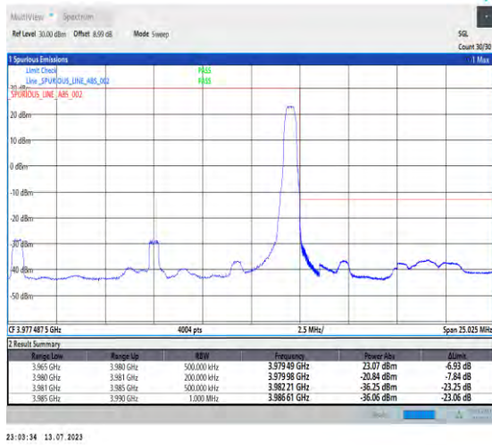
1-N77-3700-3980-PC1.5-30-15-H-2-DFT-PI2BPSK-Edge_1RB_Right-1@37-Ant3-1--PASS-see graph
