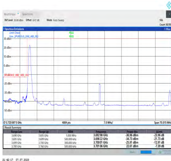
1-N77-3700-3980-PC1.5-30-60-L-4-CP-QPSK-Edge_1RB_Left-1@0-Ant3-1--PASS-see graph
