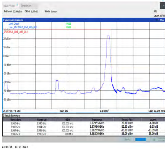
1-N77-3700-3980-PC1.5-30-20-H-2-DFT-PI2BPSK-Edge_1RB_Right-1@50-Ant3-1--PASS-see graph
