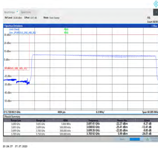
1-N77-3700-3980-PC1.5-30-50-L-6-CP-QPSK-Outer_Full-133@0-Ant3-1--PASS-see graph
