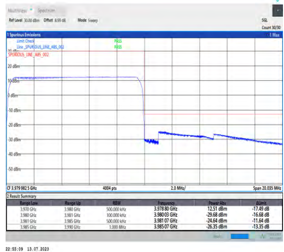
1-N77-3700-3980-PC1.5-30-10-H-6-CP-QPSK-Outer_Full-24@0-Ant3-1--PASS-see graph
