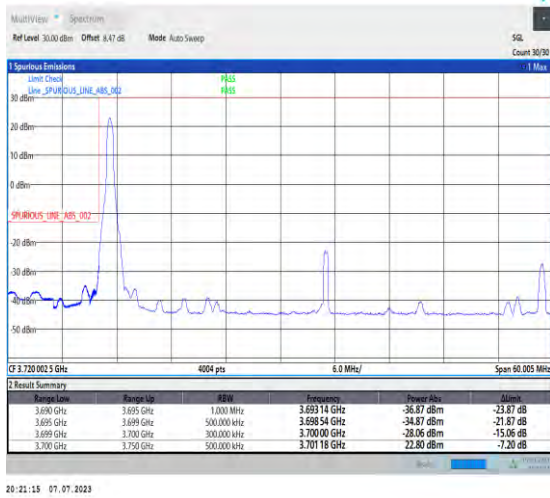
1-N77-3700-3980-PC1.5-30-50-L-1-DFT-PI2BPSK-Edge_1RB_Left-1@0-Ant3-1--PASS-see graph
