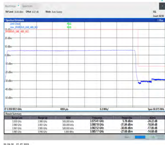
1-N77-3700-3980-PC1.5-30-50-H-6-CP-QPSK-Outet_Full-133@0-Ant3-1--PASS-see graph
