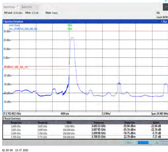
1-N77-3700-3980-PC1.5-30-15-L-4-CP-QPSK-Edge_1RB_Left-1@0-Ant3-1--PASS-see graph
