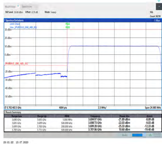
1-N77-3700-3980-PC1.5-30-15-L-6-CP-QPSK-Outer_Full-38@0-Ant3-1--PASS-see graph
