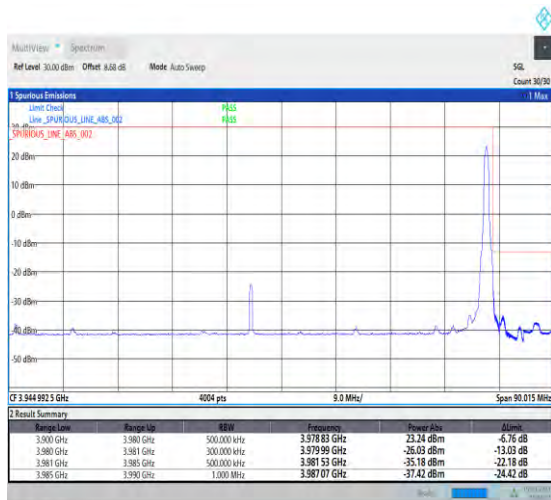
1-N77-3700-3980-PC1.5-30-80-H-2-DFT-PI2BPSK-Edge_1RB_Right-1@216-Ant3-1--PASS-see graph
