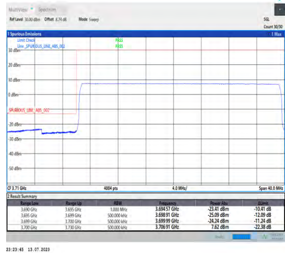
1-N77-3700-3980-PC1.5-30-30-L-3-DFT-PI2BPSK-Outer_Full-75@0-Ant3-1--PASS-see graph
