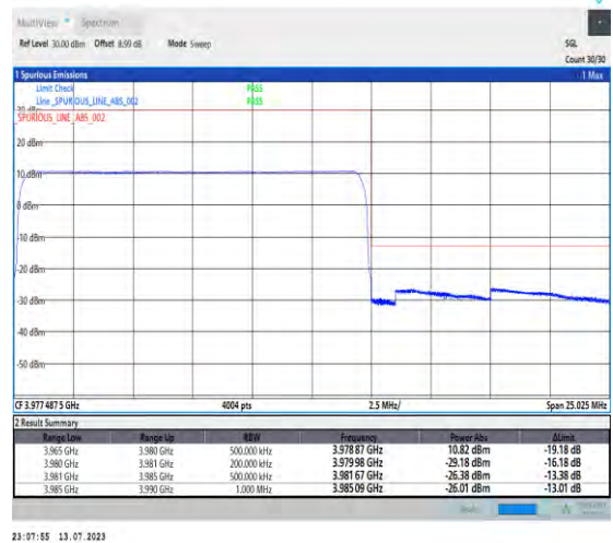
1-N77-3700-3980-PC1.5-30-15-H-6-CP-QPSK-Outer_Full-38@0-Ant3-1--PASS-see graph
