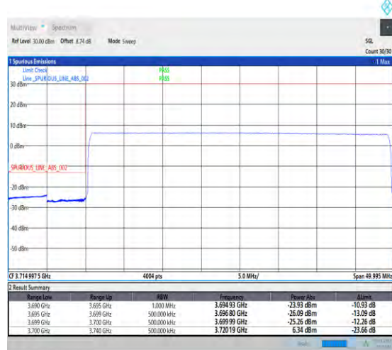
1-N77-3700-3980-PC1.5-30-40-L-6-CP-QPSK-Outer_Full-100@0-Ant3-1--PASS-see graph
