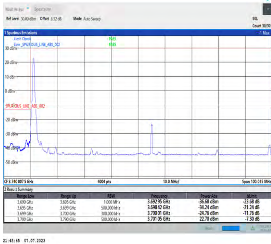
1-N77-3700-3980-PC1.5-30-90-L-1-DFT-PI2BPSK-Edge_1RB_Left-1@0-Ant3-1--PASS-see graph
