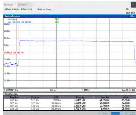
1-N77-3700-3980-PC1.5-30-80-L-3-DFT-PI2BPSK-Outer_Full-100@0-Ant3-1--PASS-see graph
