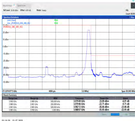
1-N77-3700-3980-PC1.5-30-20-H-5-CP-QPSK-Edge_1RB_Right-1@50-Ant3-1--PASS-see graph
