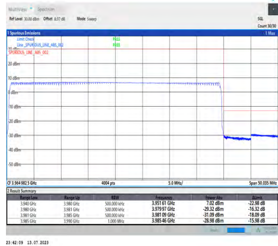
1-N77-3700-3980-PC1.5-30-40-H-3-DFT-PI2BPSK-Outet_Full-100@0-Ant3-1--PASS-see graph
