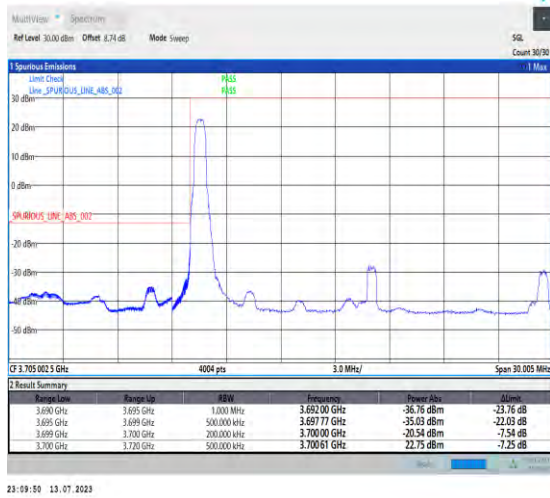
1-N77-3700-3980-PC1.5-30-20-L-1-DFT-PI2BPSK-Edge_1RB_Left-1@0-Ant3-1--PASS-see graph
