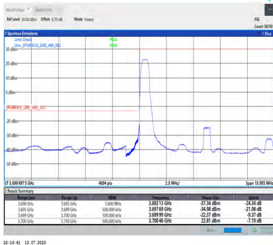
1-N77-3700-3980-PC1.5-30-10-L-1-DFT-PI2BPSK-Edge_1RB_Left-1@0-Ant3-1--PASS-see graph
