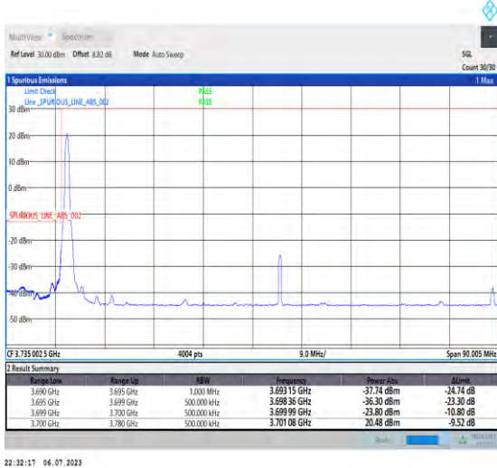
1-N77-3700-3980-PC1-30-80-L-1-DFT-PI2BPSK-Edge_1RB_Left-1@0-Ant3-1--PASS-see graph
