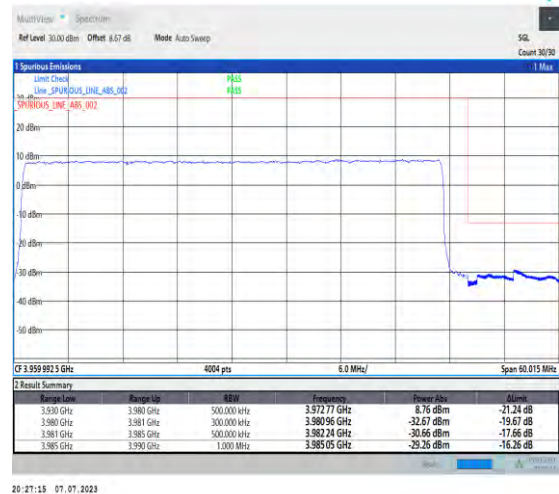
1-N77-3700-3980-PC1.5-30-50-H-3-DFT-PI2BPSK-Outet_Full-128@0-Ant3-1--PASS-see graph
