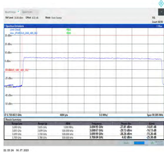
1-N77-3700-3980-PC1-30-80-L-3-DFT-PI2BPSK-Outer_Full-100@0-Ant3-1--PASS-see graph
