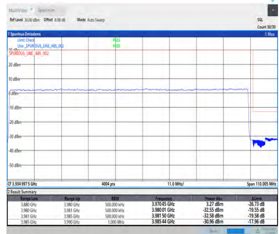
1-N77-3700-3980-PC1-30-100-H-3-DFT-PI2BPSK-Outer_Full-270@0-Ant3-1--PASS-see graph
