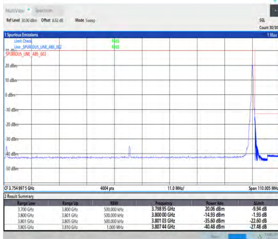
1-N77-3700-3980-PC1-30-100-H-2-DFT-PI2BPSK-Outer_Full-1@0-Ant3-1--PASS-see graph
