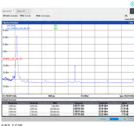
1-N77-3700-3980-PC1.5-30-90-L-4-CP-QPSK-Edge_1RB_Left-1@0-Ant3-1--PASS-see graph
