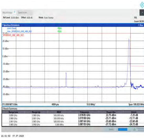
1-N77-3700-3980-PC1.5-30-90-H-5-CP-QPSK-Edge_1RB_Right-1@244-Ant3-1--PASS-see graph
