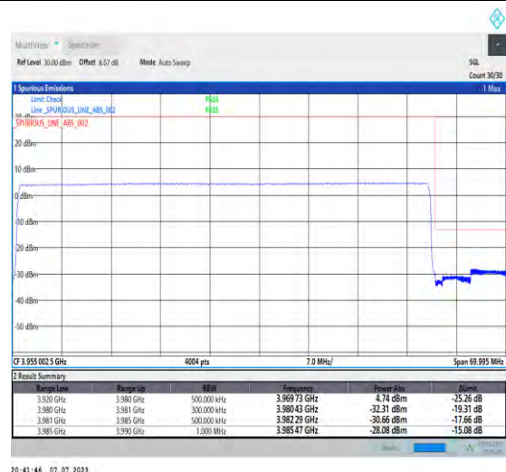
1-N77-3700-3980-PC1.5-30-60-H-6-CP-QPSK-Outet_Full-162@0-Ant3-1--PASS-see graph
