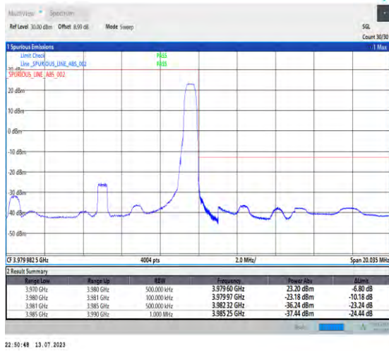
1-N77-3700-3980-PC1.5-30-10-H-2-DFT-PI2BPSK-Edge_1RB_Right-1@23-Ant3-1--PASS-see graph
