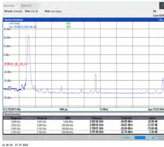
1-N77-3700-3980-PC1.5-30-60-L-1-DFT-PI2BPSK-Edge_1RB_Left-1@0-Ant3-1--PASS-see graph
