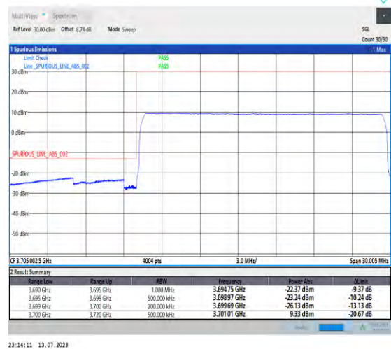
1-N77-3700-3980-PC1.5-30-20-L-6-CP-QPSK-Outer_Full-51@0-Ant3-1--PASS-see graph
