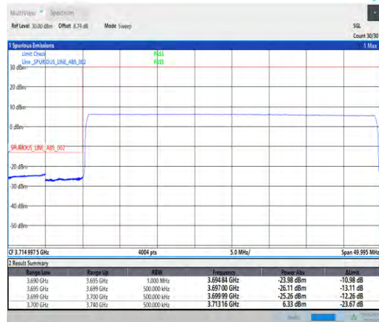
1-N77-3700-3980-PC1.5-30-40-L-3-DFT-PI2BPSK-Outer_Full-100@0-Ant3-1--PASS-see graph
