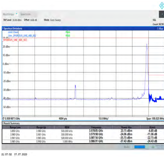
1-N77-3700-3980-PC1.5-30-90-H-2-DFT-PI2BPSK-Edge_1RB_Right-1@244-Ant3-1--PASS-see graph
