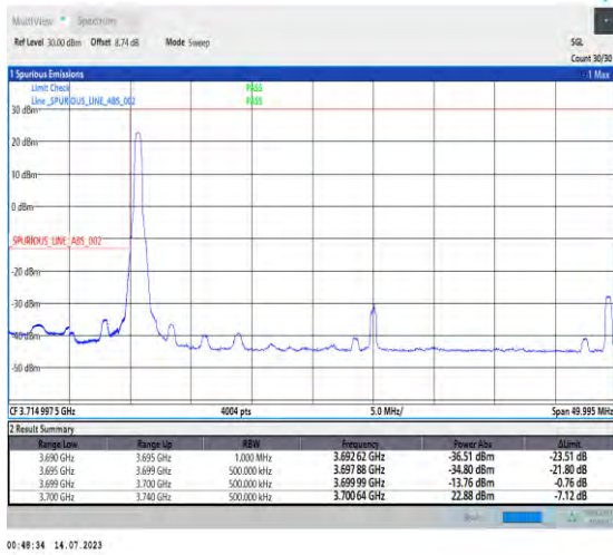
1-N77-3700-3980-PC1.5-30-40-L-1-DFT-PI2BPSK-Edge_1RB_Left-1@0-Ant3-1--PASS-see graph
