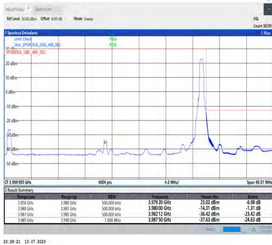
1-N77-3700-3980-PC1.5-30-30-H-2-DFT-PI2BPSK-Edge_1RB_Right-1@77-Ant3-1--PASS-see graph
