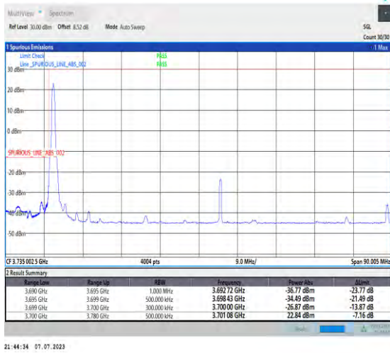
1-N77-3700-3980-PC1.5-30-80-L-1-DFT-PI2BPSK-Edge_1RB_Left-1@0-Ant3-1--PASS-see graph
