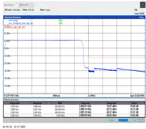
1-N77-3700-3980-PC1.5-30-15-H-3-DFT-PI2BPSK-Outer_Full-36@0-Ant3-1--PASS-see graph
