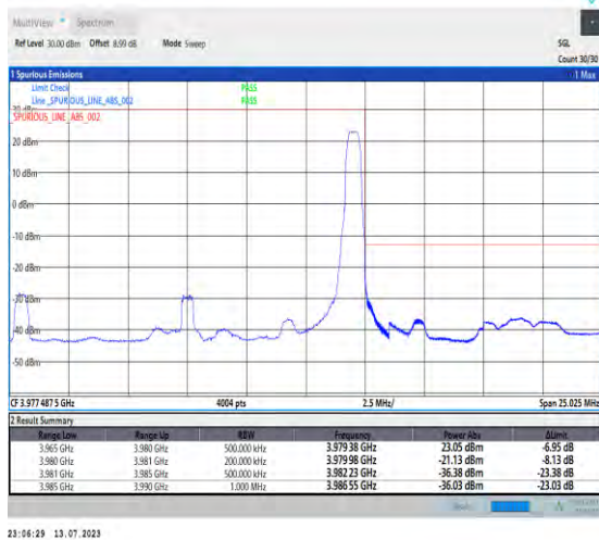
1-N77-3700-3980-PC1.5-30-15-H-5-CP-QPSK-Edge_1RB_Right-1@37-Ant3-1--PASS-see graph
