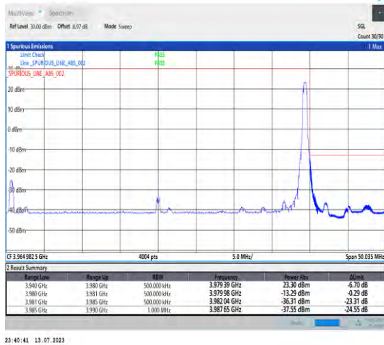
1-N77-3700-3980-PC1.5-30-40-H-2-DFT-PI2BPSK-Edge_1RB_Right-1@105-Ant3-1--PASS-see graph
