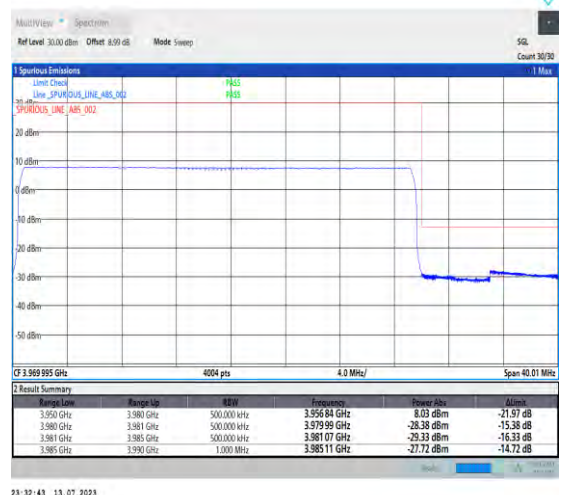
1-N77-3700-3980-PC1.5-30-30-H-6-CP-QPSK-Outer_Full-75@0-Ant3-1--PASS-see graph
