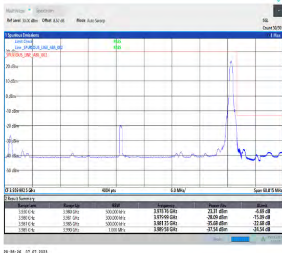
1-N77-3700-3980-PC1.5-30-50-H-5-CP-QPSK-Edge_1RB_Right-1@132-Ant3-1--PASS-see graph
