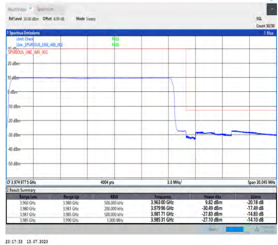
1-N77-3700-3980-PC1.5-30-20-H-3-DFT-PI2BPSK-Outer_Full-50@0-Ant3-1--PASS-see graph
