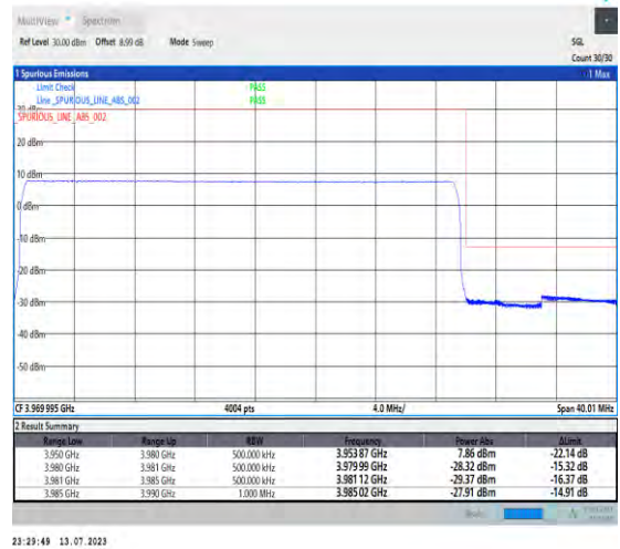
1-N77-3700-3980-PC1.5-30-30-H-3-DFT-PI2BPSK-Outer_Full-75@0-Ant3-1--PASS-see graph
