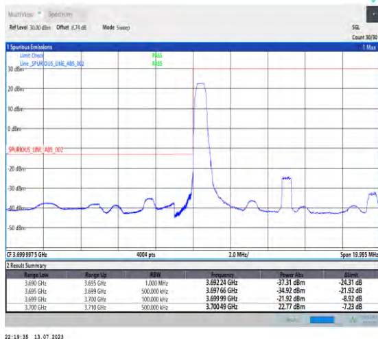
1-N77-3700-3980-PC1.5-30-10-L-4-CP-QPSK-Edge_1RB_Left-1@0-Ant3-1--PASS-see graph
