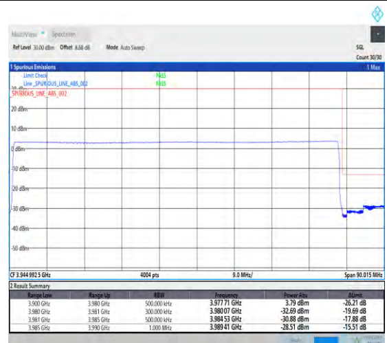
1-N77-3700-3980-PC1.5-30-80-H-3-DFT-PI2BPSK-Outet_Full-100@0-Ant3-1--PASS-see graph
