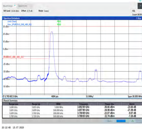
1-N77-3700-3980-PC1.5-30-20-L-4-CP-QPSK-Edge_1RB_Left-1@0-Ant3-1--PASS-see graph
