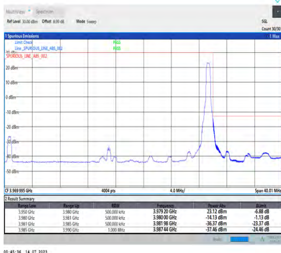
1-N77-3700-3980-PC1.5-30-30-H-5-CP-QPSK-Edge_1RB_Right-1@77-Ant3-1--PASS-see graph
