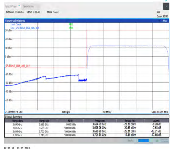
1-N77-3700-3980-PC1.5-30-10-L-6-CP-QPSK-Outer_Full-24@0-Ant3-1--PASS-see graph
