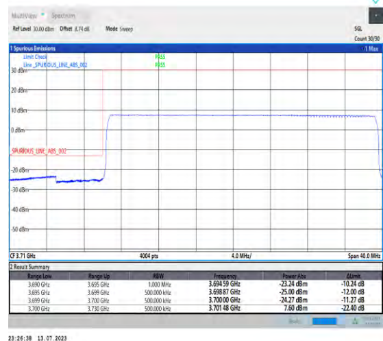
1-N77-3700-3980-PC1.5-30-30-L-6-CP-QPSK-Outer_Full-75@0-Ant3-1--PASS-see graph
