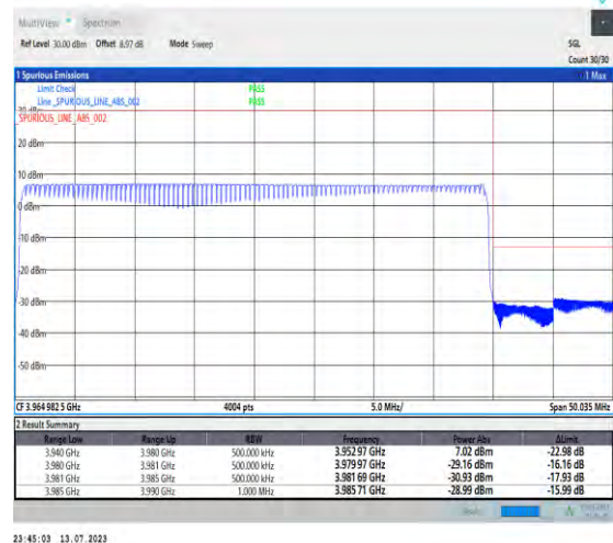
1-N77-3700-3980-PC1.5-30-40-H-6-CP-QPSK-Outet_Full-100@0-Ant3-1--PASS-see graph
