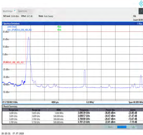
1-N77-3700-3980-PC1.5-30-50-L-4-CP-QPSK-Edge_1RB_Left-1@0-Ant3-1--PASS-see graph
