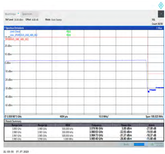
1-N77-3700-3980-PC1.5-30-90-H-6-CP-QPSK-Outer_Full-245@0-Ant3-1--PASS-see graph
