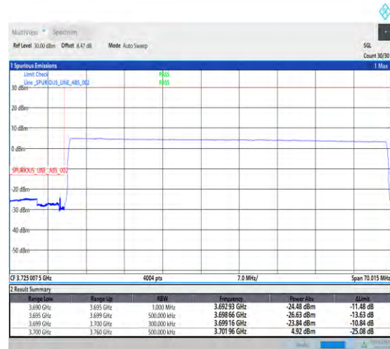
1-N77-3700-3980-PC1.5-30-60-L-3-DFT-PI2BPSK-Outer_Full-162@0-Ant3-1--PASS-see graph
