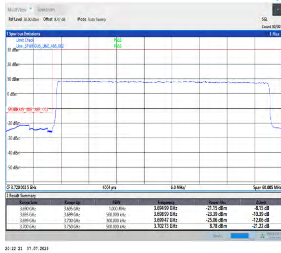
1-N77-3700-3980-PC1.5-30-50-L-3-DFT-PI2BPSK-Outer_Full-128@0-Ant3-1--PASS-see graph
