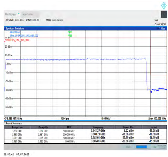
1-N77-3700-3980-PC1.5-30-90-H-3-DFT-PI2BPSK-Outer_Full-240@0-Ant3-1--PASS-see graph
