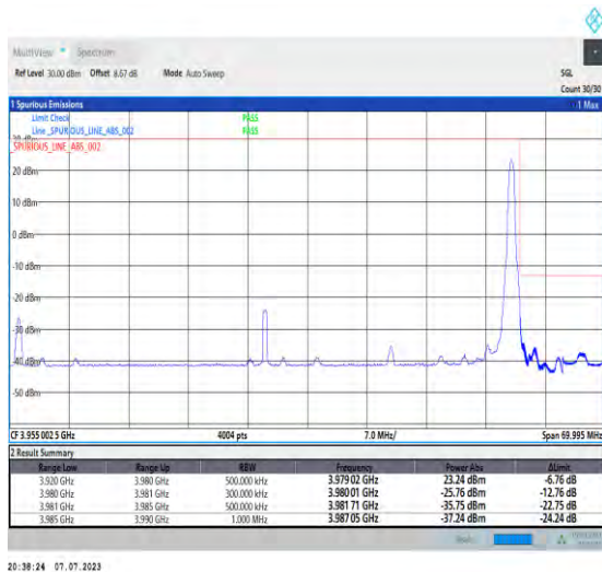
1-N77-3700-3980-PC1.5-30-60-H-2-DFT-PI2BPSK-Edge_1RB_Right-1@161-Ant3-1--PASS-see graph
