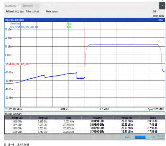
1-N77-3700-3980-PC1.5-30-10-L-3-DFT-PI2BPSK-Outer_Full-24@0-Ant3-1--PASS-see graph
