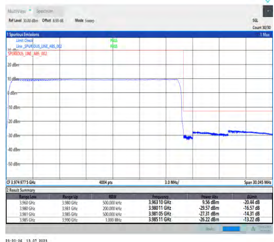
1-N77-3700-3980-PC1.5-30-20-H-6-CP-QPSK-Outer_Full-51@0-Ant3-1--PASS-see graph
