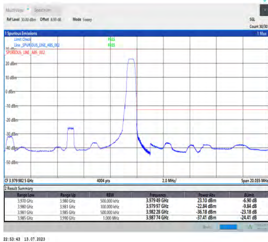
1-N77-3700-3980-PC1.5-30-10-H-5-CP-QPSK-Edge_1RB_Right-1@23-Ant3-1--PASS-see graph
