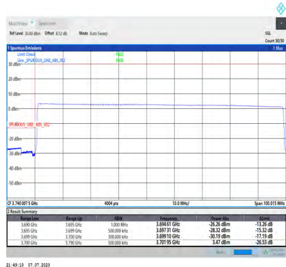
1-N77-3700-3980-PC1.5-30-90-L-6-CP-QPSK-Outer_Full-245@0-Ant3-1--PASS-see graph
