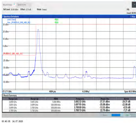
1-N77-3700-3980-PC1.5-30-30-L-1-DFT-PI2BPSK-Edge_1RB_Left-1@0-Ant3-1--PASS-see graph
