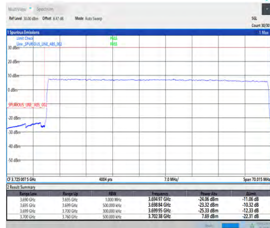
1-N77-3700-3980-PC1.5-30-60-L-3-DFT-PI2BPSK-Outer_Full-162@0-Ant3-1--PASS-see graph
