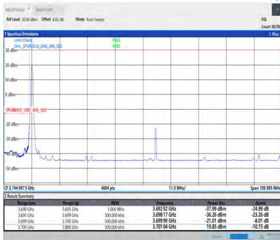
1-N77-3700-3980-PC1-30-100-L-4-CP-QPSK-Edge_1RB_Left-1@0-Ant3-1--PASS-see graph
