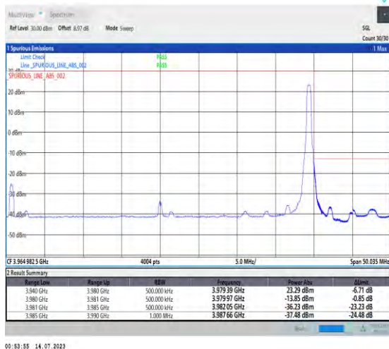
1-N77-3700-3980-PC1.5-30-40-H-5-CP-QPSK-Edge_1RB_Right-1@105-Ant3-1--PASS-see graph
