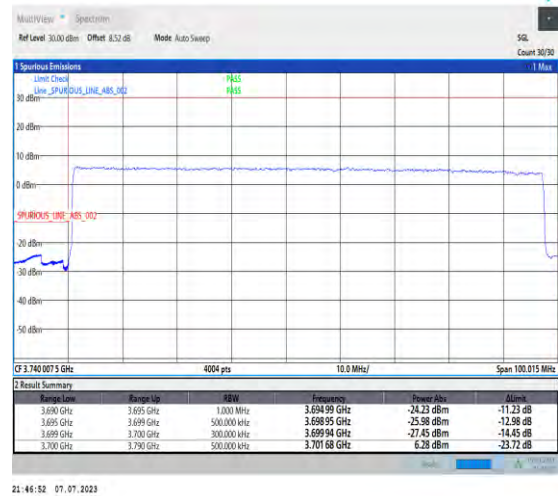
1-N77-3700-3980-PC1.5-30-90-L-3-DFT-PI2BPSK-Outer_Full-240@0-Ant3-1--PASS-see graph
