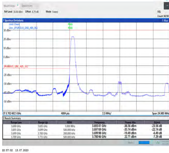
1-N77-3700-3980-PC1.5-30-15-L-1-DFT-PI2BPSK-Edge_1RB_Left-1@0-Ant3-1--PASS-see graph
