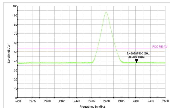
3DH5-Channel 78: Average
