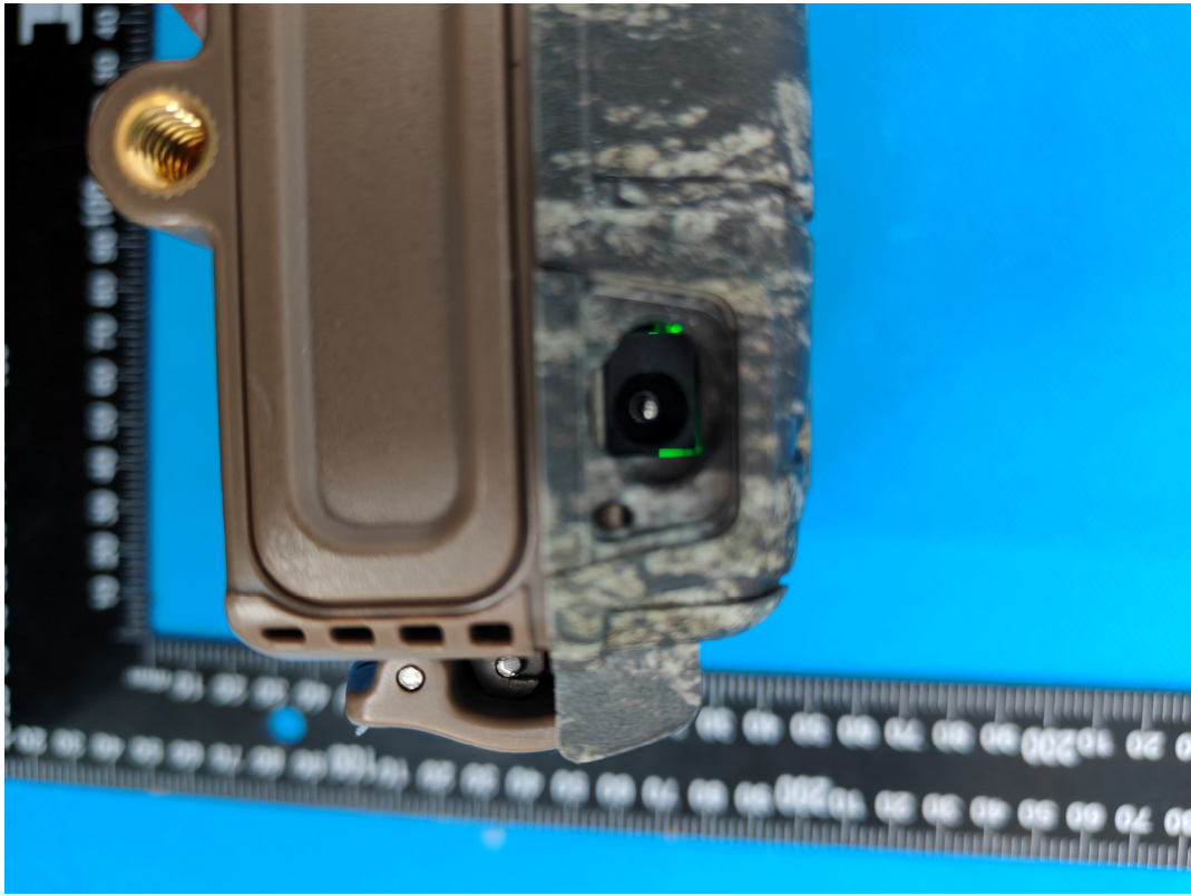
4G Main Antenna Port
