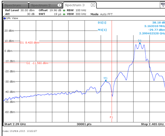
Figure 7.4.1.2-4: Lower Band-edge
