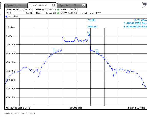
Figure 7.2.2-6: 99% Bandwidth Plot – HCH
