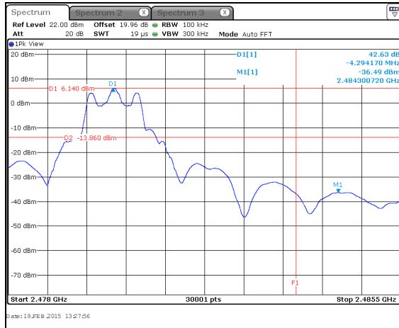
Figure 7.4.1.2-5: Upper Band-edge
