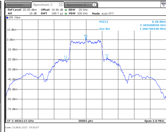
Figure 7.2.2-4: 99% Bandwidth Plot – LCH
