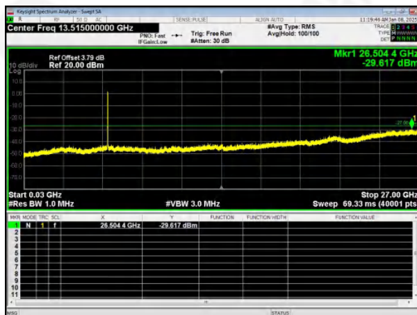
802.11ax40 on channel 159
