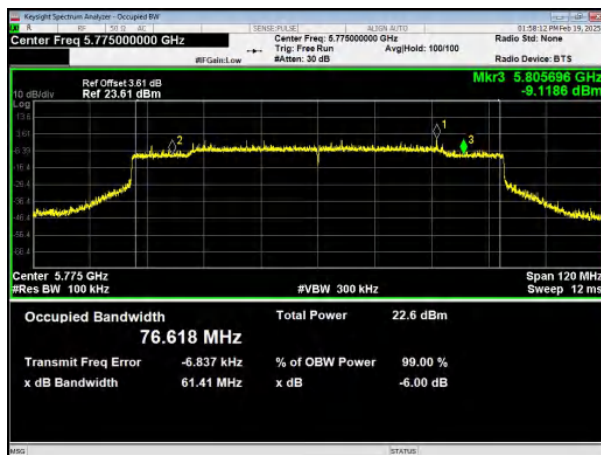
(802.11ax80) Bandwidth plot on channel 155
