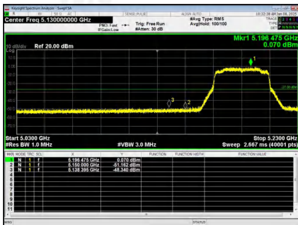
(802.11ax80) Band Edge, Left Side
