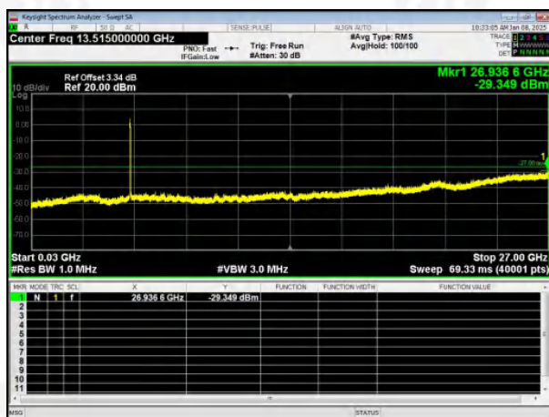
802.11ax40 on channel 46
