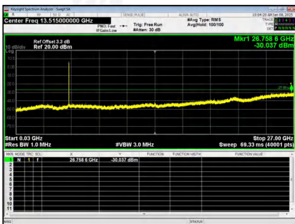
802.11ax20 on channel 36
