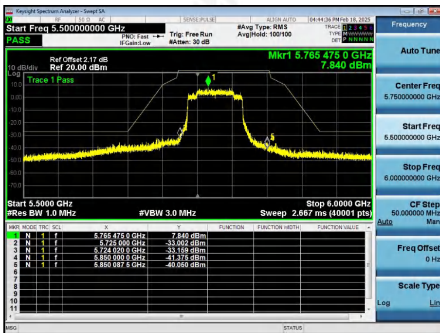
(802.11ax80) Band Edge, Left Side
