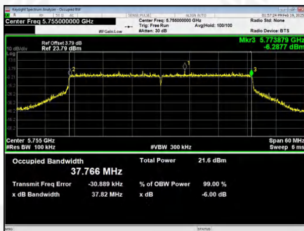
(802.11ax40) Bandwidth plot on channel 151
