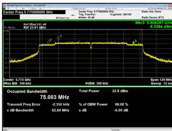
(802.11ac80) Bandwidth plot on channel 155
