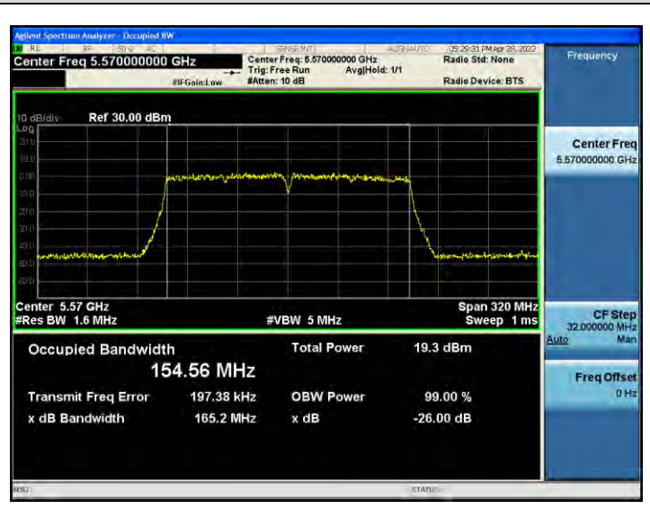
802.11ac_VHT160 UNII 2A BAND 26 dB Bandwidth (CH 114)
