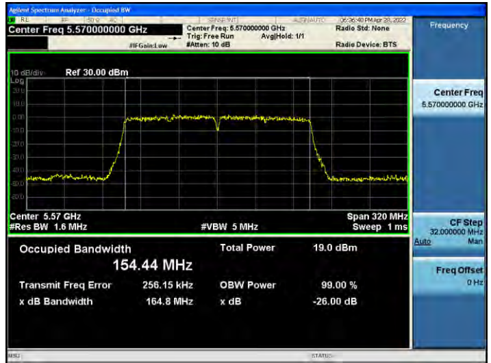
802.11ac_VHT160 UNII 2A BAND 26 dB Bandwidth (CH 114)
