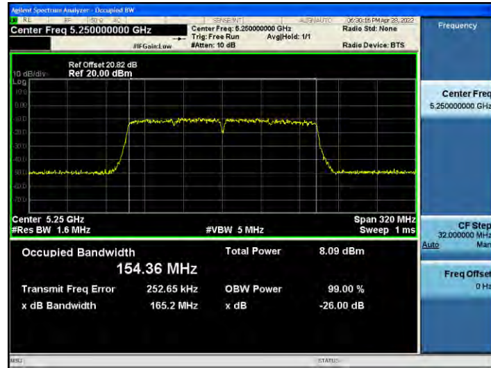
802.11ac_VHT160 UNII 1 BAND 26 dB Bandwidth(CH 50)
