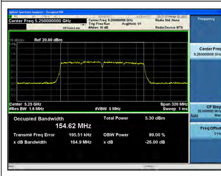
802.11ac_VHT160 UNII 1 BAND 26 dB Bandwidth(CH 50)
