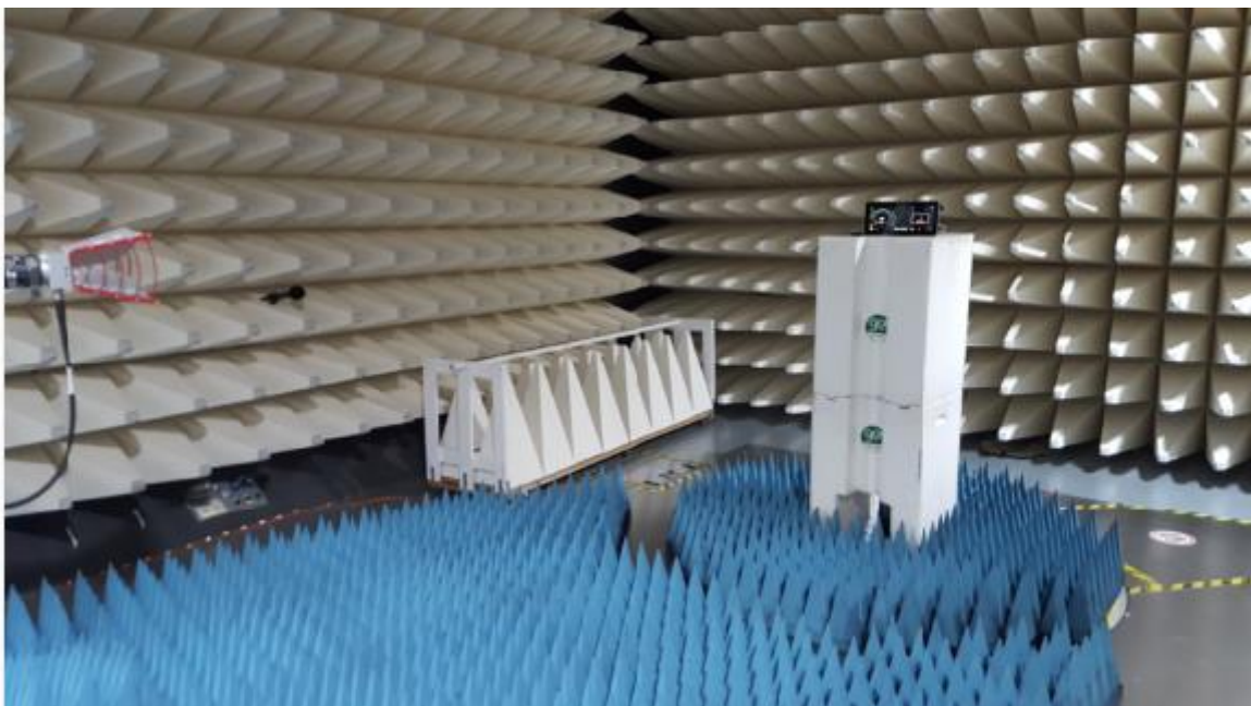
6. Radiated Emission test setup 1
