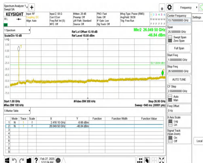
11N40SISO_Ant1_2422_1000~26500
