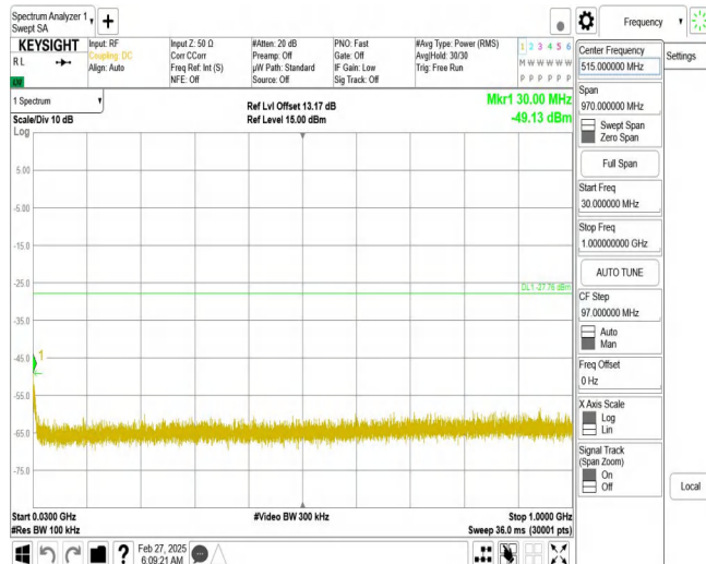
11N40SISO_Ant1_2452_30~1000
