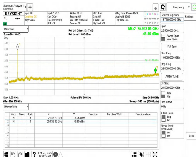
11N40SISO_Ant1_2452_1000~26500
