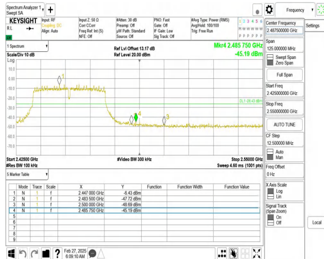
11N40SISO_Ant1_High_2452
