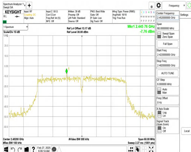
11N40SISO_Ant1_2452_0~Reference
