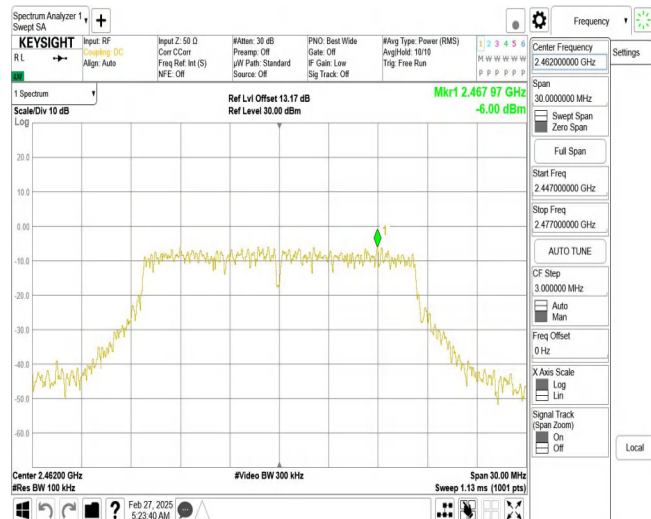
11G_Ant1_2462_0~Reference
