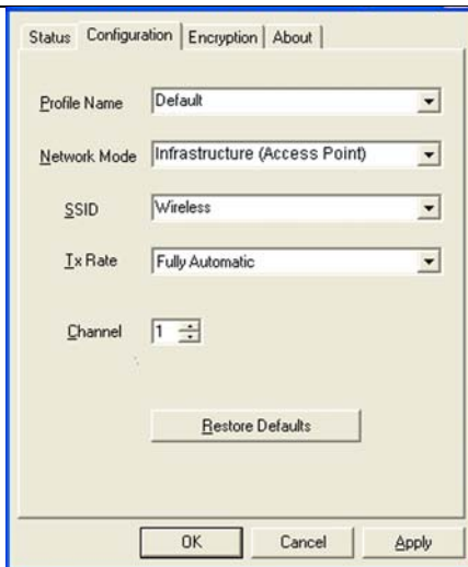
WG511 Configuration Utility
