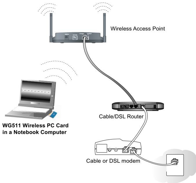
Figure 2-1: NETGEAR WG511 Wireless PC Card in Infrastructure Mode
