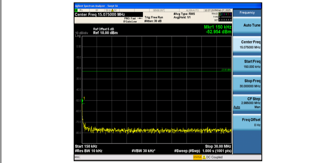
Band26_5MHz_16QAM_26740_1RB#0_0.15~30_0.15~30
