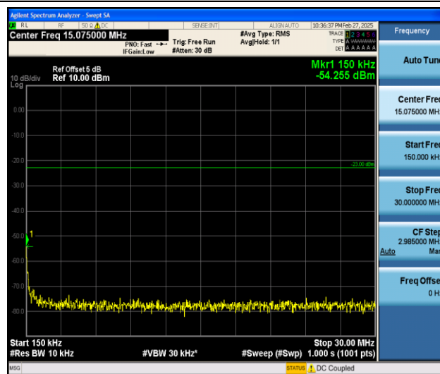
Band26_5MHz_QPSK_26740_1RB#0_0.15~30_0.15~30
