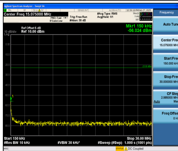
Band26_5MHz_16QAM_26765_1RB#0_0.15~30_0.15~30
