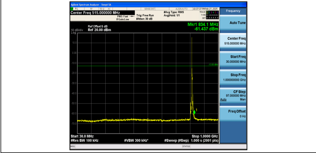
Band26_5MHz_16QAM_26740_1RB#0_30~1000_30~1000
