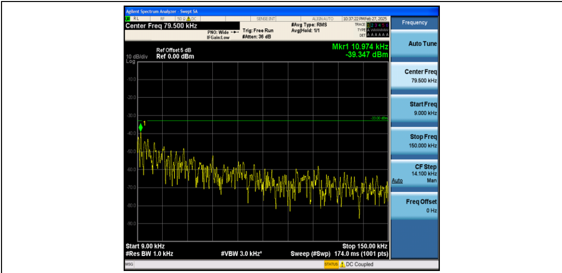
Band26_5MHz_16QAM_26740_1RB#0_0.009~0.15_0.009~0.15
