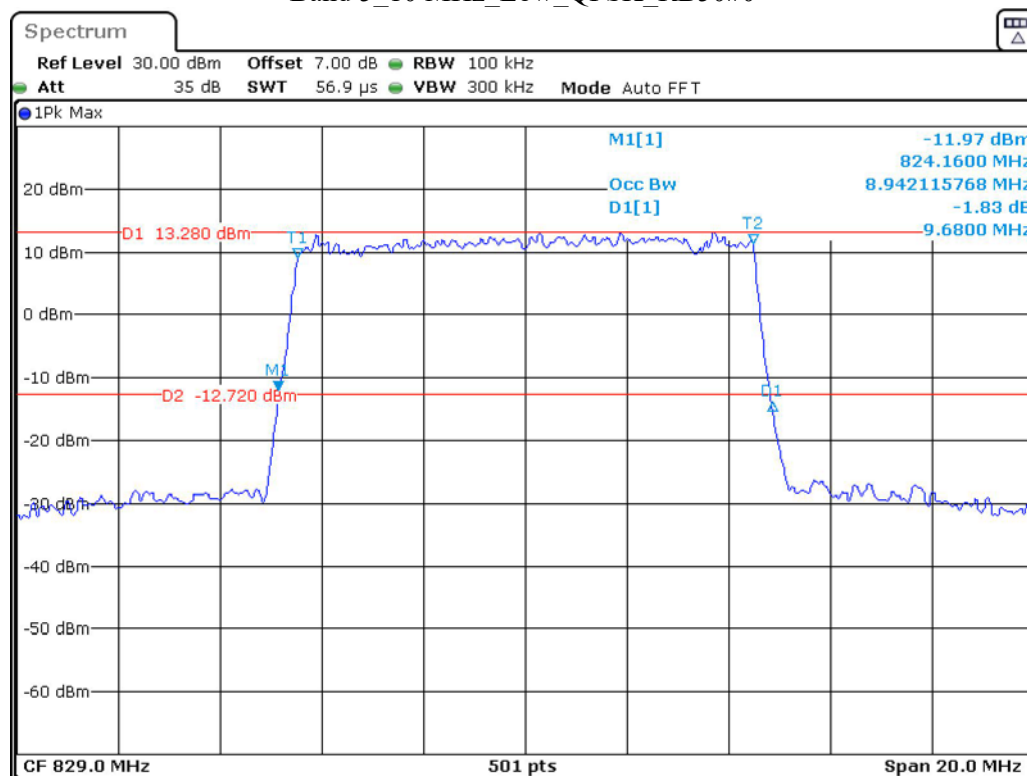
Band 5 10 MHz Low QPSK RB50#0
