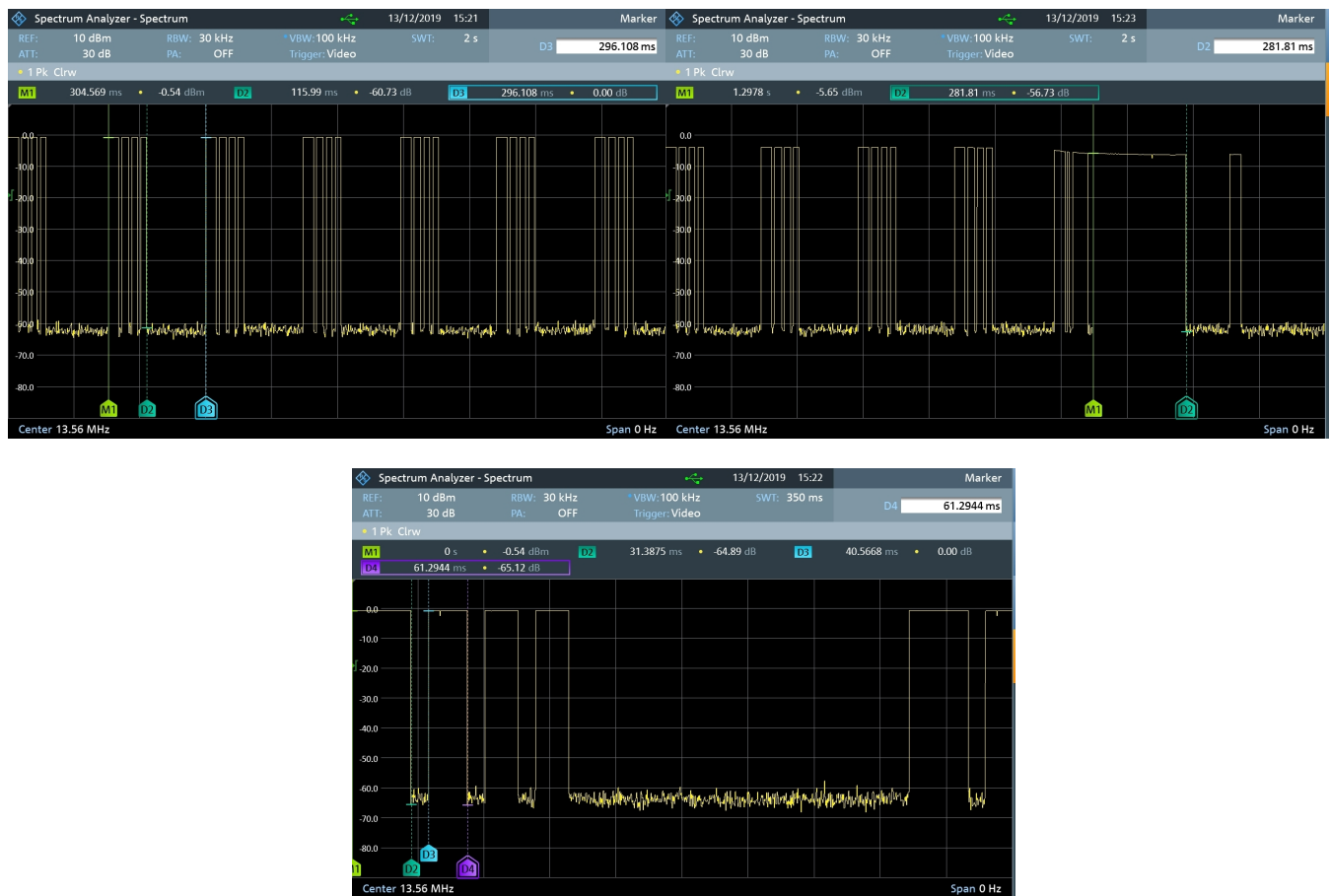
Figure 7(b): Pulsed Emission Characteristics (Duty Cycle).
