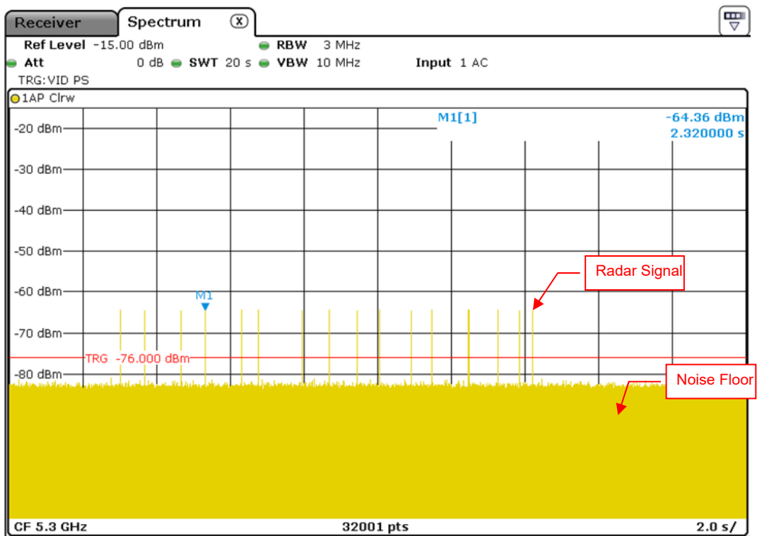
Radar Signal 5
