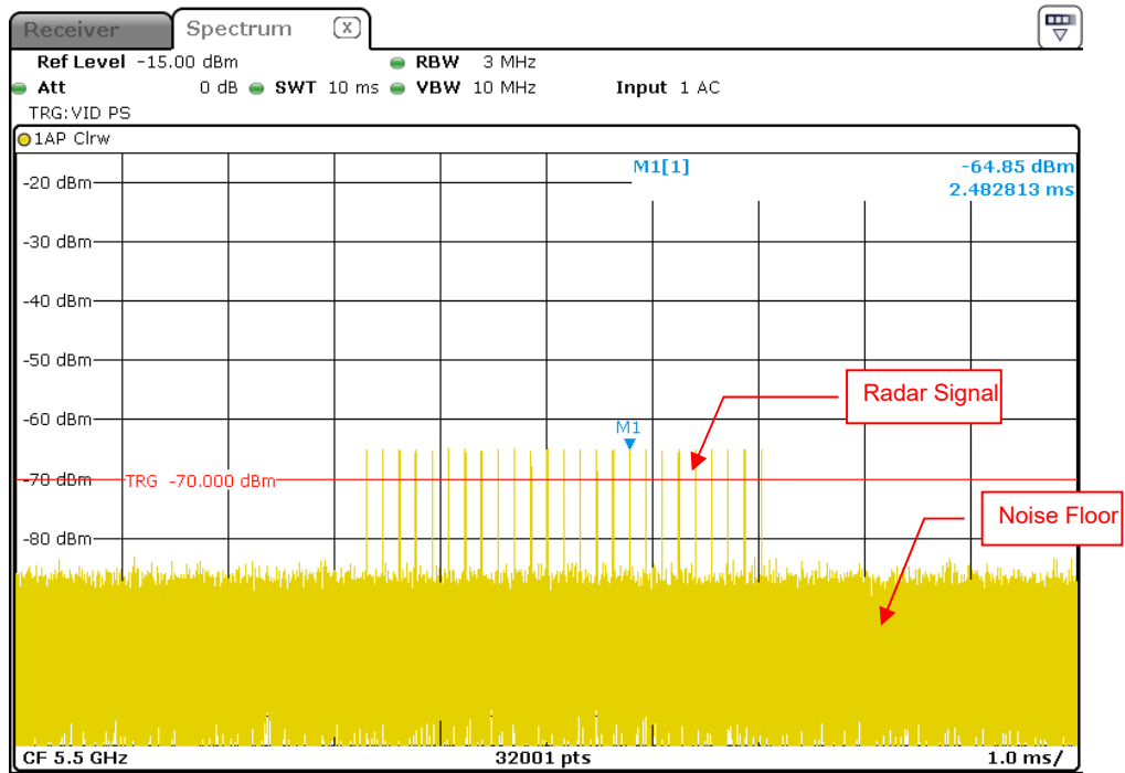
Radar Signal 2
