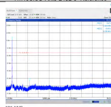
11n40SISO-Ant0-2452-1000~26500
