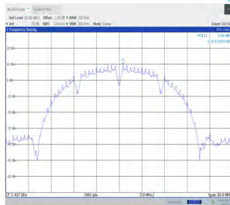
11b-Ant0-2437-0~Reference
