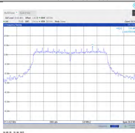
11g-Ant0-2412-0~Reference
