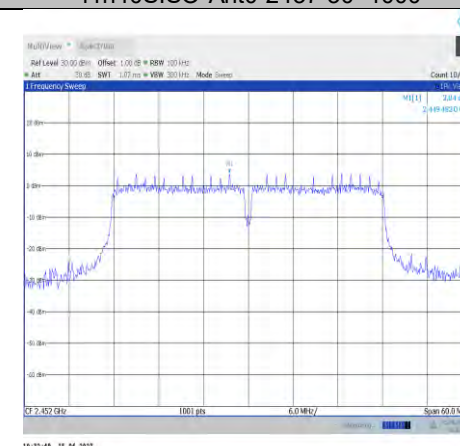
11n40SISO-Ant0-2452-0~Reference
