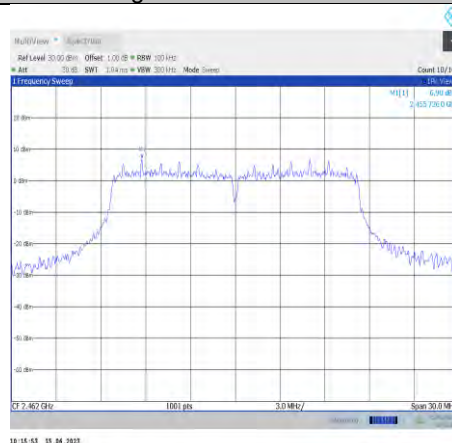
11g-Ant0-2462-0~Reference
