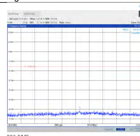
11n40SISO-Ant0-2437-30~1000
