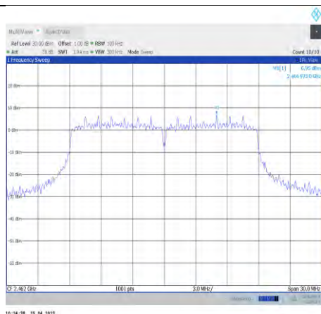
11n20SISO-Ant0-2462-0~Reference
