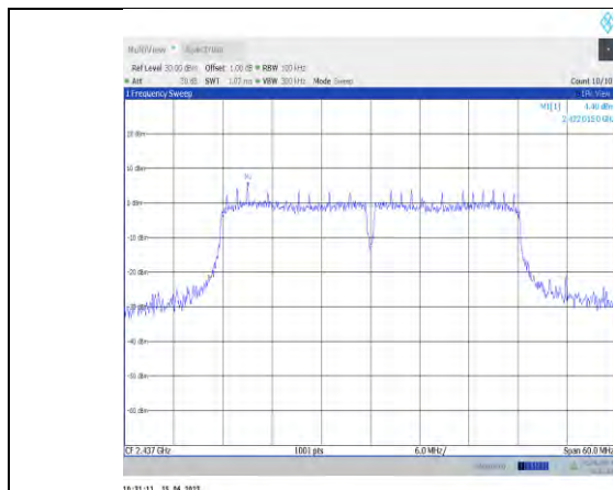
11n40SISO-Ant0-2437-0~Reference
