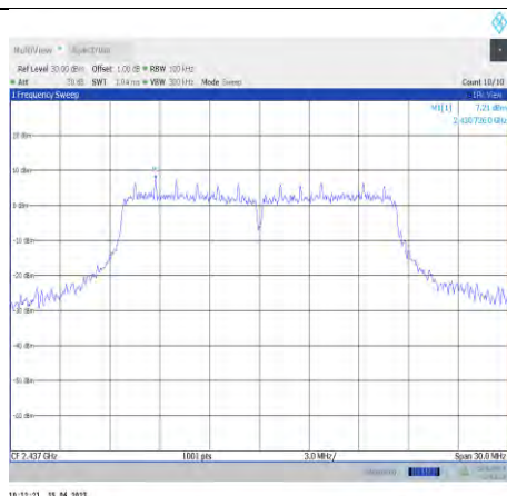
11g-Ant0-2437-0~Reference
