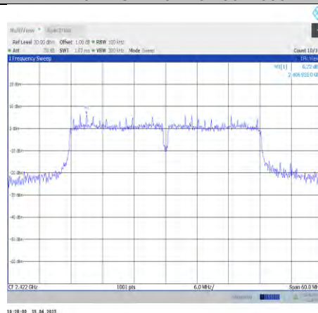
11n40SISO-Ant0-2422-0~Reference
