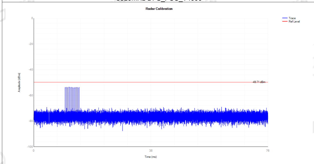
5310MHz DFS_FCC_T5000
