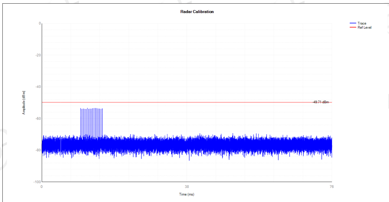
5310MHz DFS_FCC_T4000
