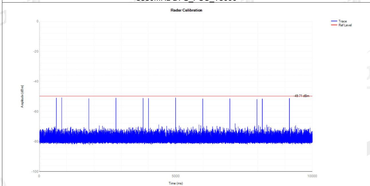
5530MHz DFS_FCC_T6000
