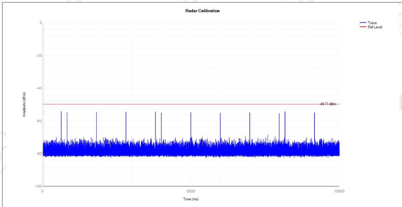
5310MHz DFS_FCC_T6000
