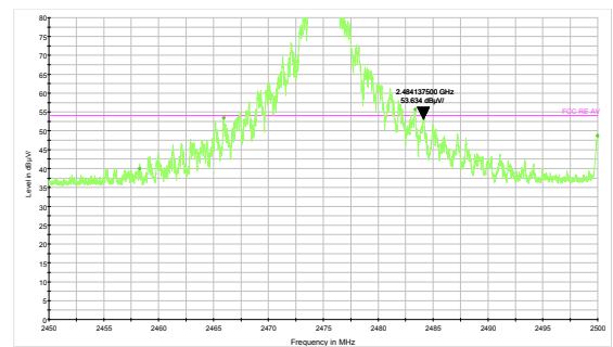
Zigbee-Channel 25: Average
