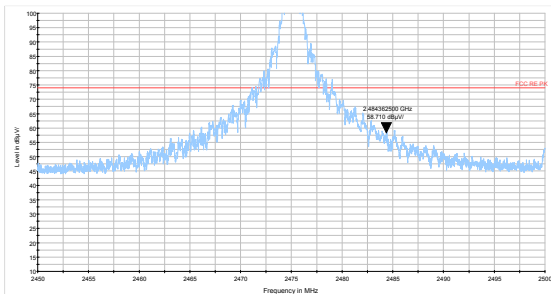
Zigbee-Channel 25: Peak
