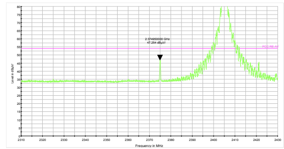
Zigbee-Channel 11: Average
