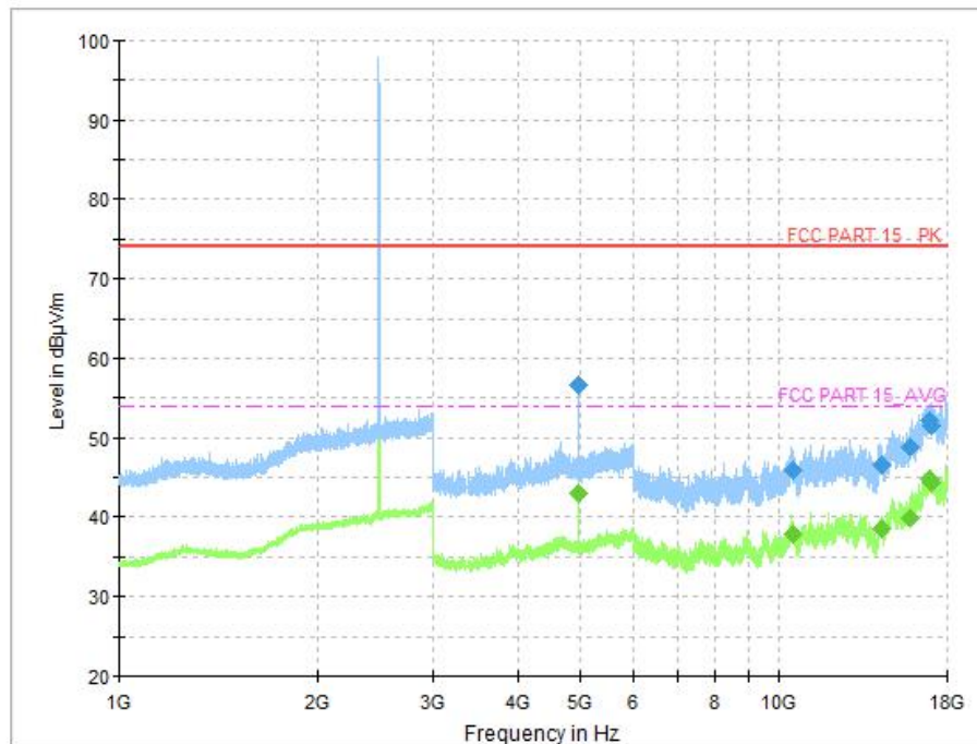
Fig.19 Radiated Spurious Emission (GFSK, Ch39, 1 GHz ~18 GHz), LE 1M
