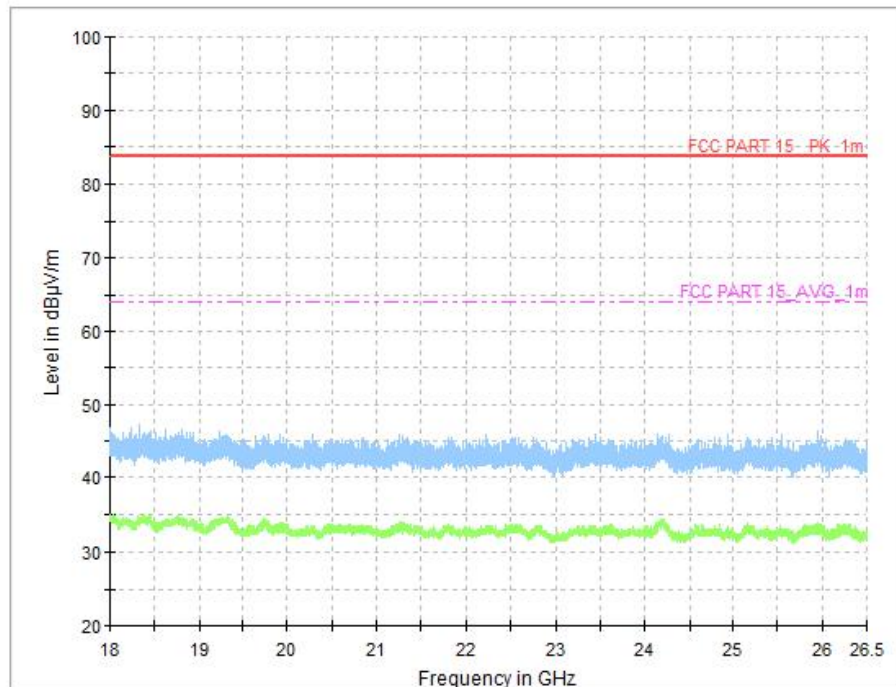
Fig.24 Radiated Spurious Emission (All Channels, 18 GHz-26.5 GHz), LE 1M
