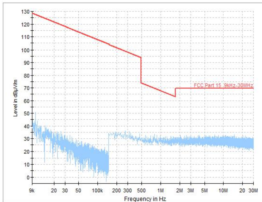
Fig.22 Radiated Spurious Emission (All Channels, 9 kHz-30 MHz), LE 1M
