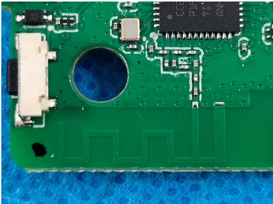
Zigbee Antenna
