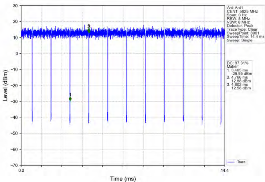
802.11ac(VHT20)_HCH_5825MHz_Ant1_NTNV
