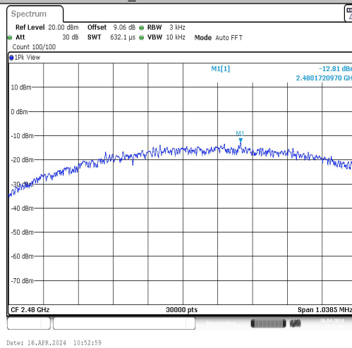
BLE_1M-Ant1-2480-PASS
