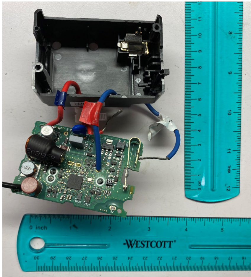
Bottom PCB with Backcover
