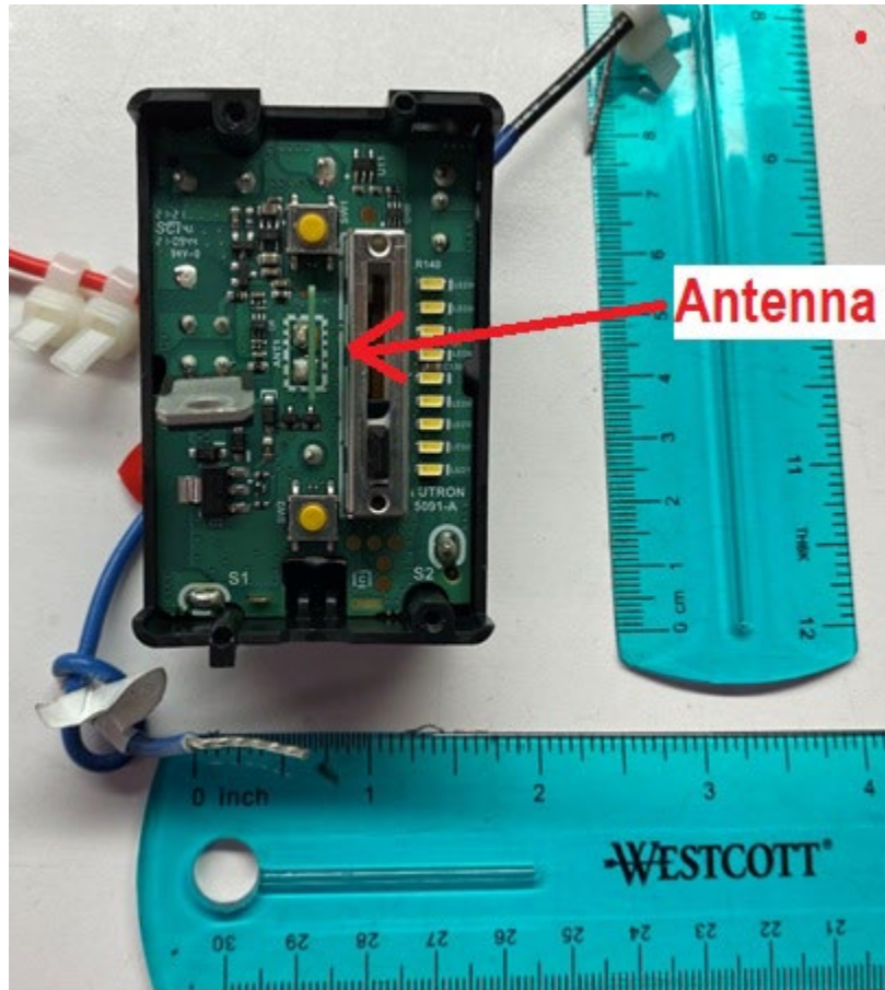
Top PCB (antenna location)
