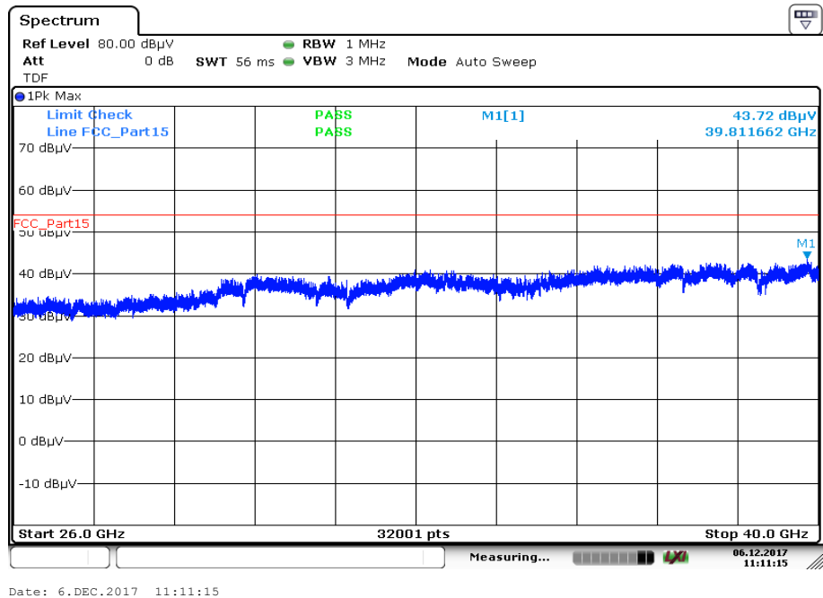
Plot 12: 26 GHz to 40 GHz; vertical & horizontal polarization; U-NII-2C; middle channel
