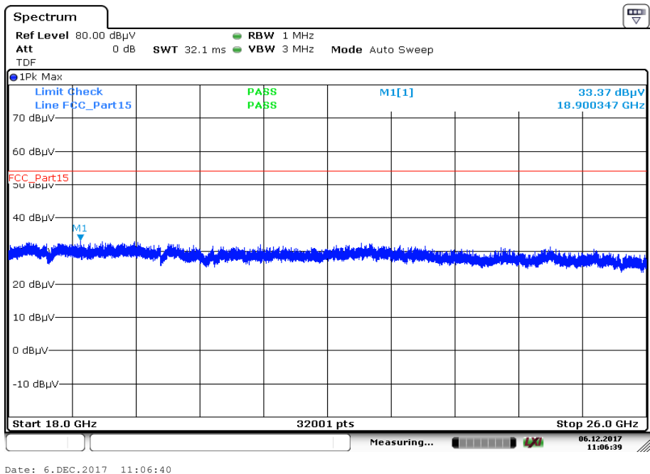
Plot 7: 18 GHz to 26 GHz; vertical & horizontal polarization; U-NII-2A; highest channel
