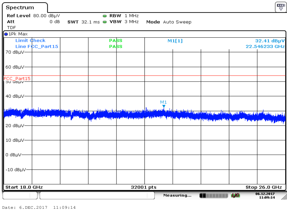
Plot 15: 18 GHz to 26 GHz; vertical & horizontal polarization; U-NII-3; middle channel
