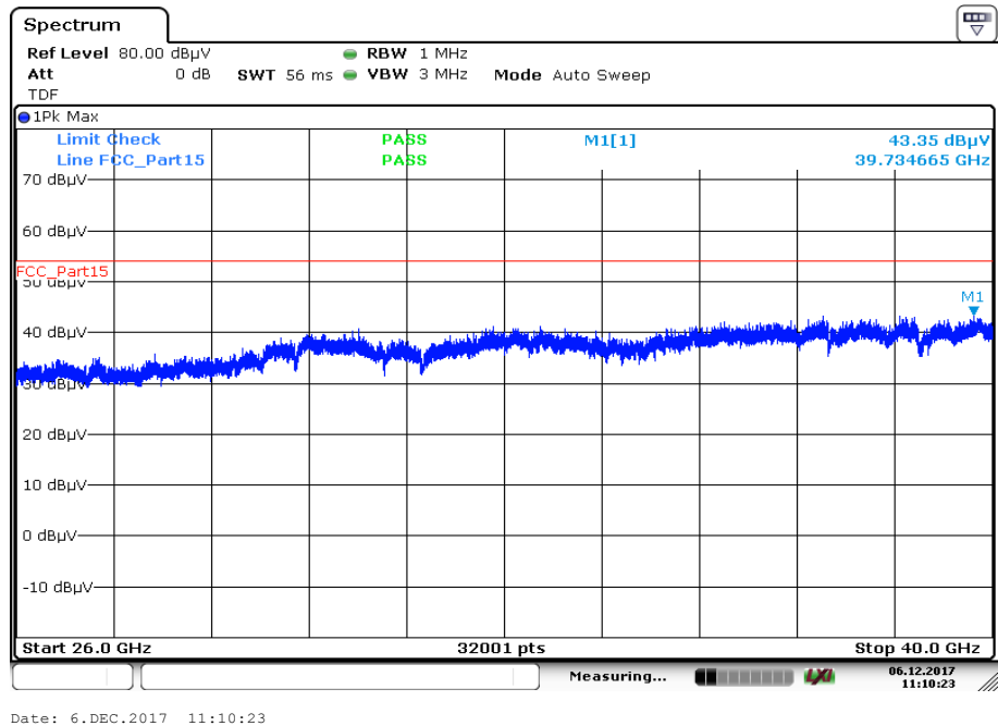
Plot 8: 26 GHz to 40 GHz; vertical & horizontal polarization; U-NII-2A; highest channel
