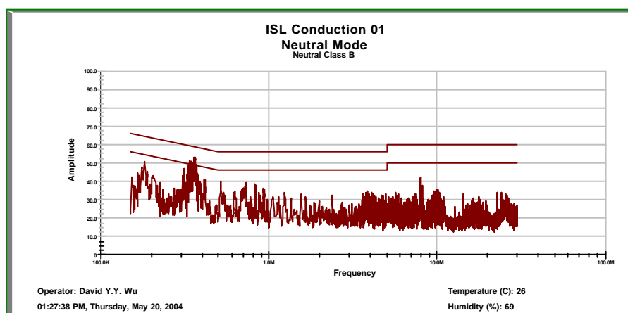
Graph 2.3.2 Power Line Conducted Emissions (Neutral)
