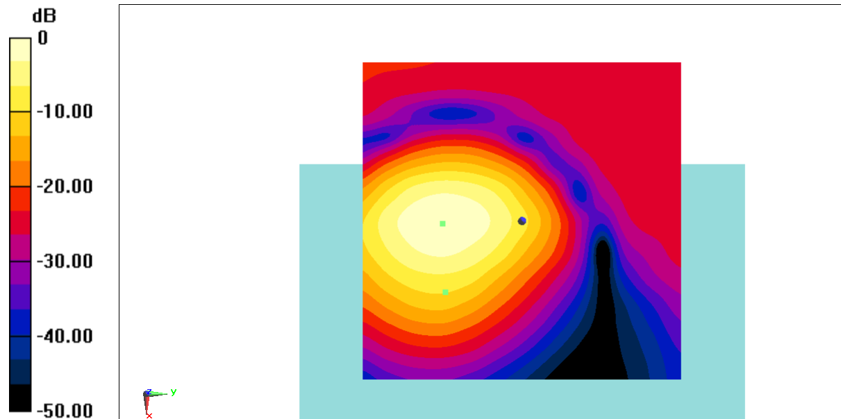
Fig B.4 T-Coil LTEB41 PC2-OTT
