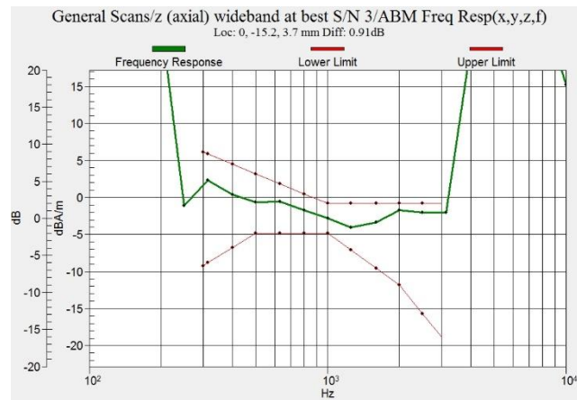
Figure C.1 Frequency Response of LTE B41 PC3
