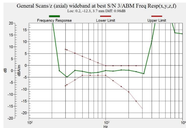
Figure C.2 Frequency Response of LTE B41 PC2 – OTT VoIP
