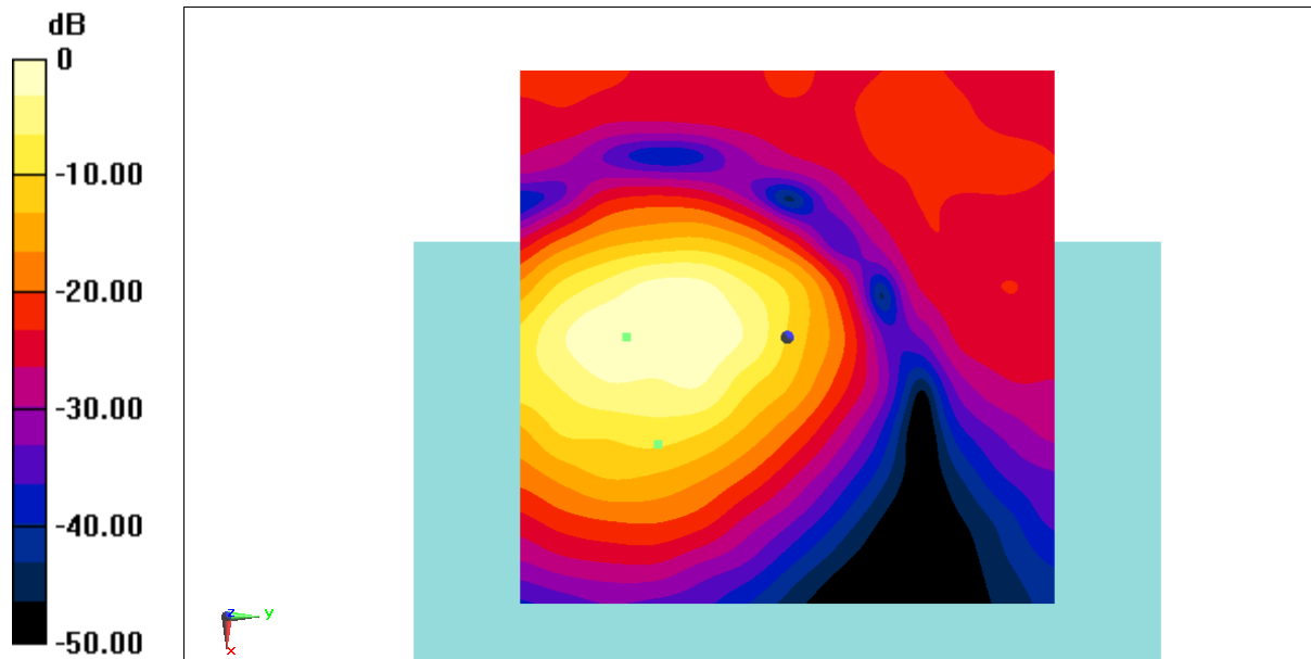
Fig B.2 T-Coil LTE Band41 PC3
