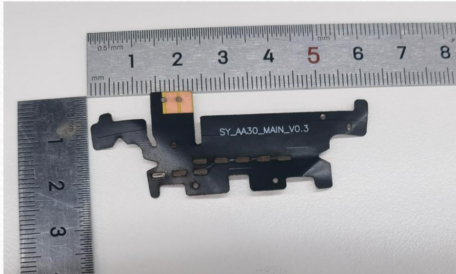
MAIN Antenna
