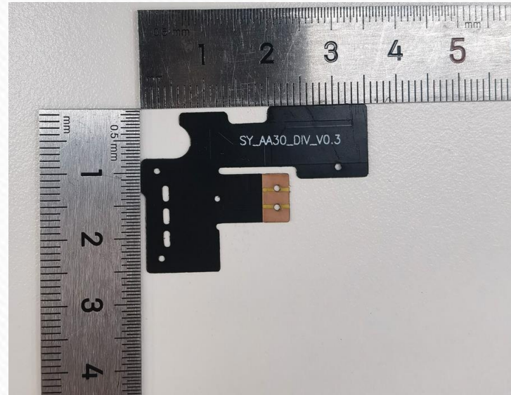
DIV Antenna
