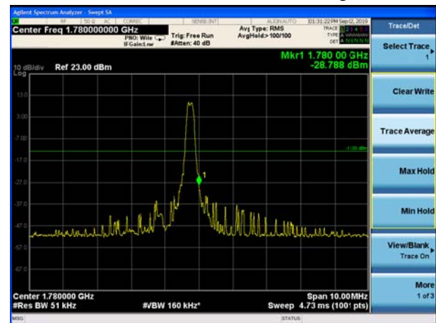
LTE Band 66 QPSK 1.4MHz CH-High, 100%RB
