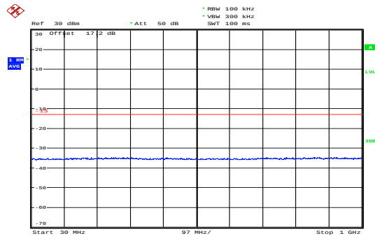
LTE Band 4 1.4MHz CH-Low 30MHz~1GHz
