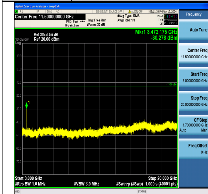
Band4_20MHz_QPSK_20300_1RB#0_3000~20000_3000~20000
