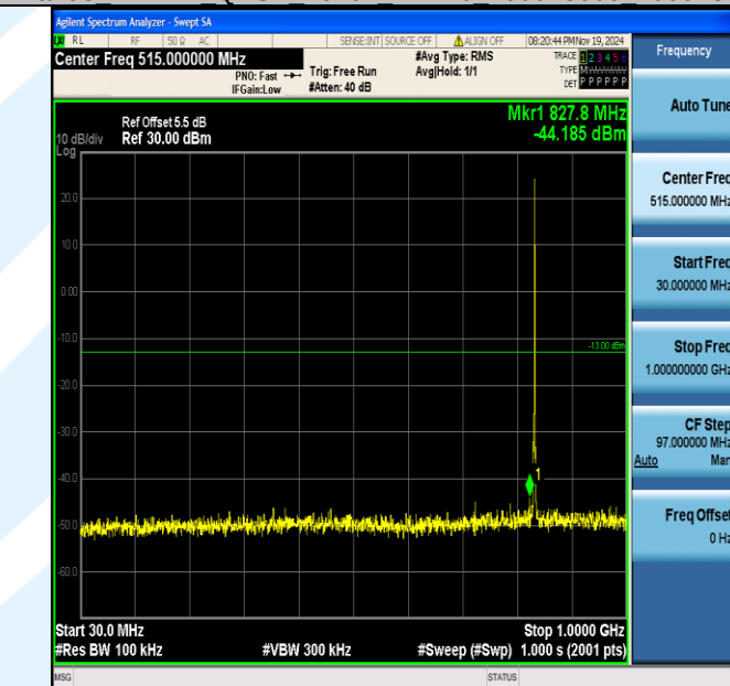
Band5_1.4MHz_QPSK_20525_1RB#0_30~1000_30~1000
