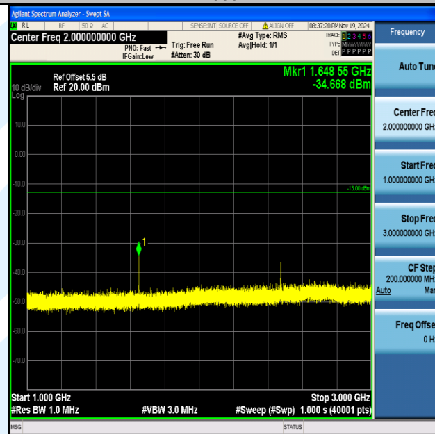
Band5 3MHz QPSK 20415 1RB#0_1000~3000 1000~3000
