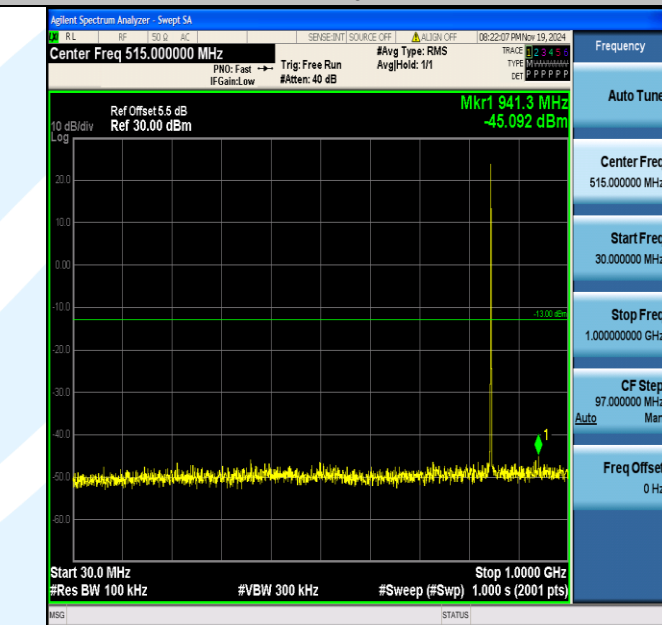
Band5_1.4MHz_16QAM_20643_1RB#0_30~1000_30~1000
