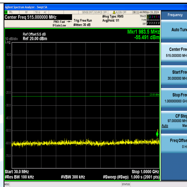
Band4_20MHz_16QAM_20300_1RB#0_30~1000_30~1000
