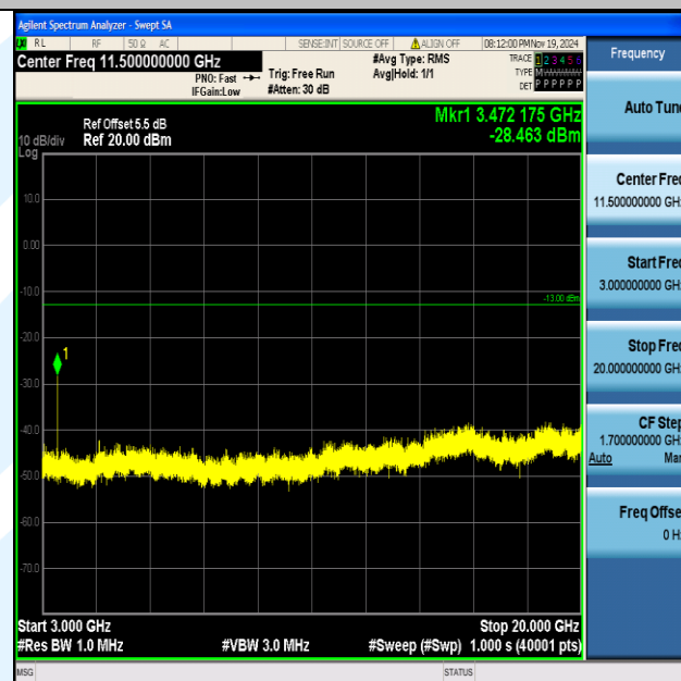
Band4_20MHz_16QAM_20300_1RB#0_3000~20000_3000~20000
