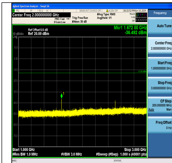
Band5_1.4MHz_QPSK_20525_1RB#0_1000~3000_1000~3000
