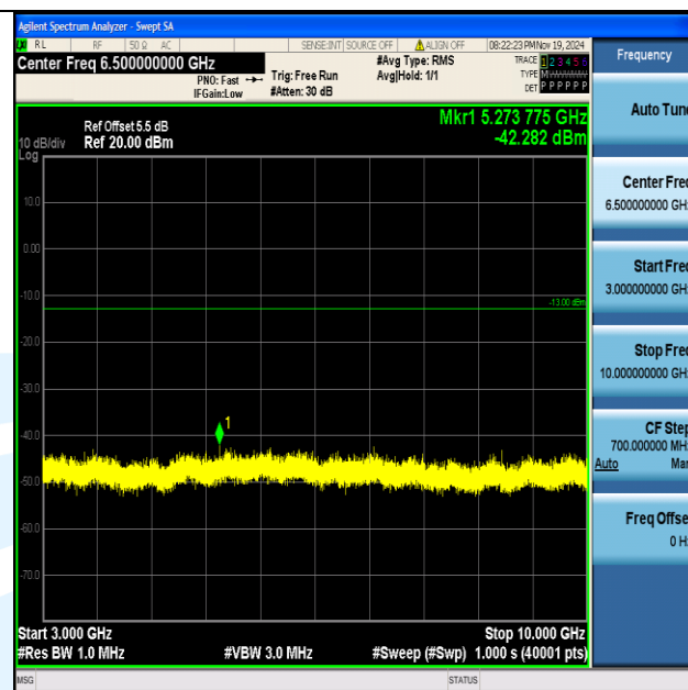
Band5_1.4MHz_16QAM_20643_1RB#0_3000~10000_3000~10000
