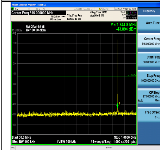
Band5_1.4MHz_QPSK_20643_1RB#0_30~1000_30~1000
