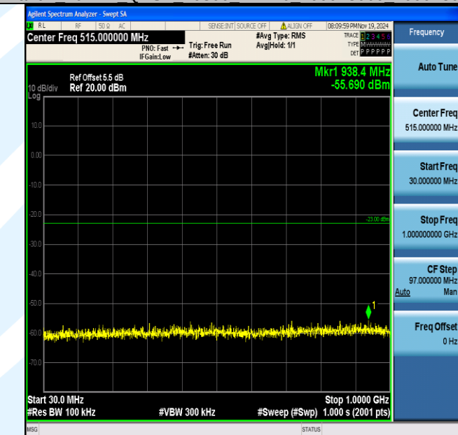
Band4_20MHz_16QAM_20050_1RB#0_30~1000_30~1000
