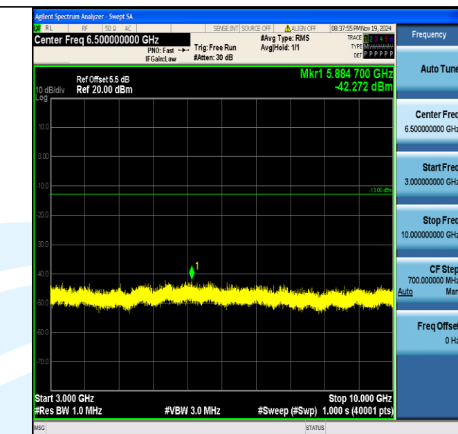
Band5_3MHz_16QAM_20415_1RB#0_3000~10000_3000~10000
