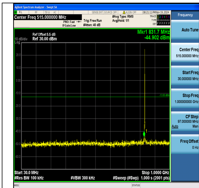
Band5_1.4MHz_16QAM_20525_1RB#0_30~1000_30~1000
