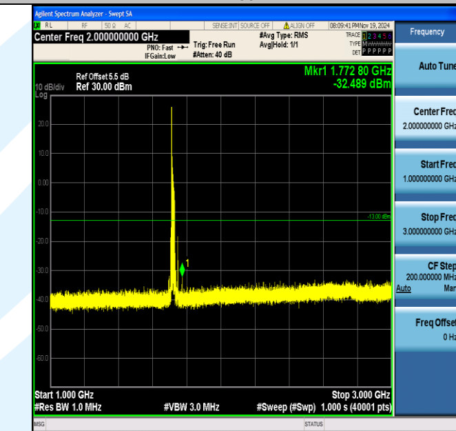
Band4_20MHz_QPSK_20050_1RB#0_1000~3000_1000~3000
