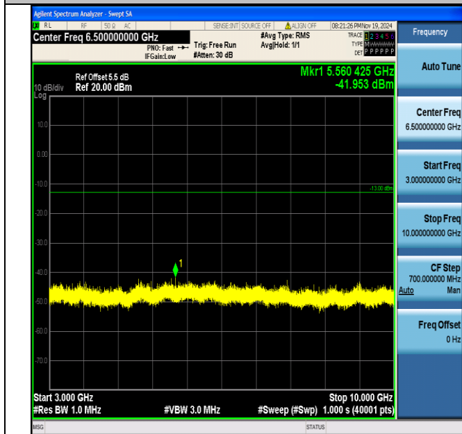
Band5_1.4MHz_16QAM_20525_1RB#0_3000~10000_3000~10000
