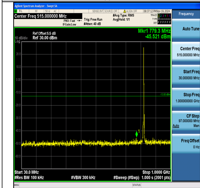
Band5 3MHz QPSK 20415 1RB#0_30~1000 30~1000
