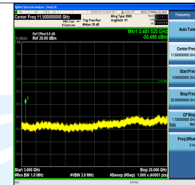
Band4_15MHz_16QAM_20325_1RB#0_3000~20000_3000~20000
