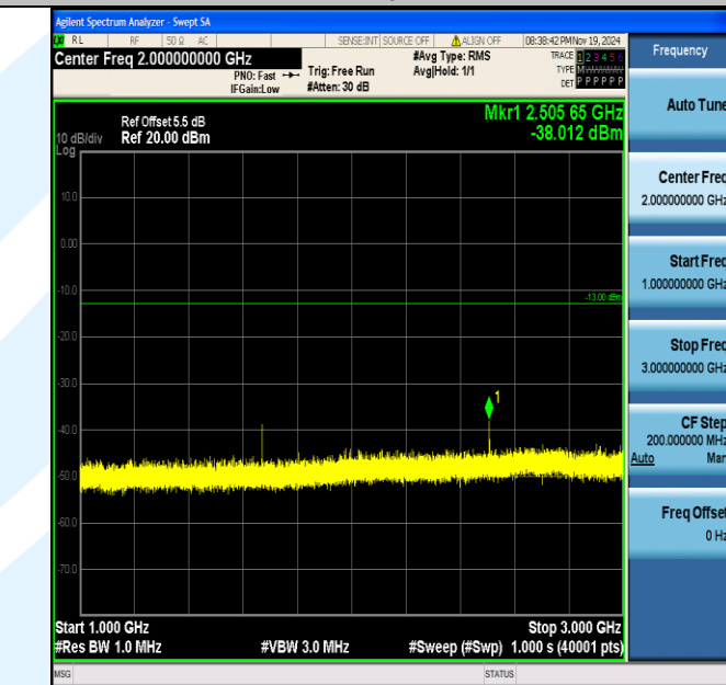
Band5_3MHz_16QAM_20525_1RB#0_1000~3000_1000~3000
