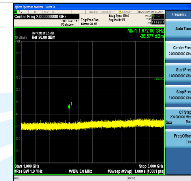
Band5_1.4MHz_16QAM_20525_1RB#0_1000~3000_1000~3000
