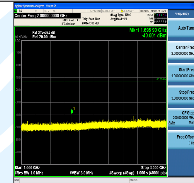
Band5_1.4MHz_QPSK_20643_1RB#0_1000~3000_1000~3000
