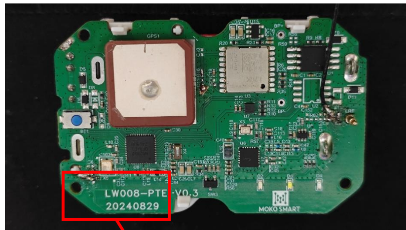
BT Antenna
