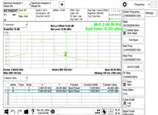
802.11ax_20MHz_2467MHz_RU106_54
