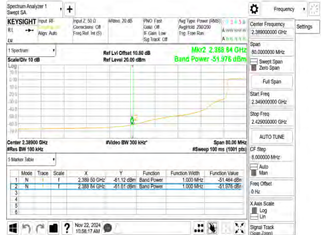
802.11ax_20MHz_2432MHz_RU242
