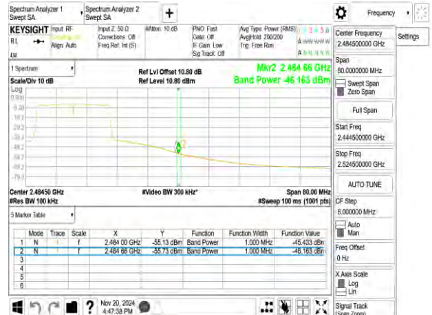
802.11ax_20MHz_2457MHz_RU106_54
