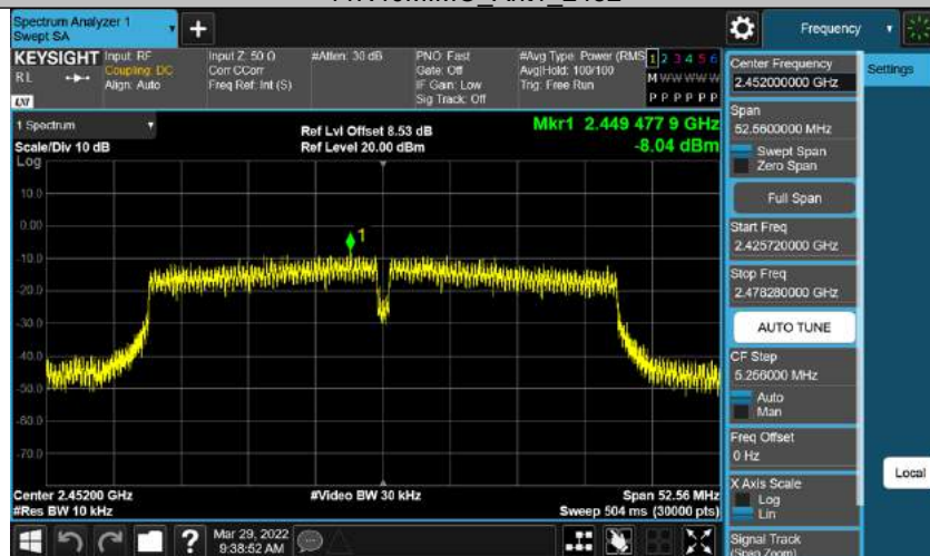
11N40MIMO Ant2 2452
