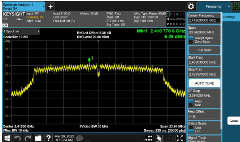
11N20MIMO Ant2 2412
