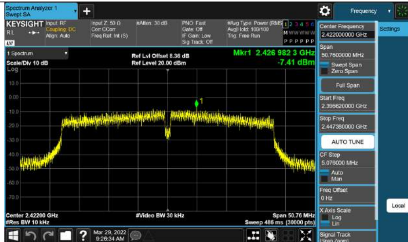
11N40MIMO Ant2 2422
