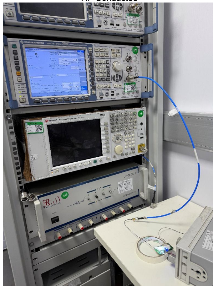
RF Conducted
