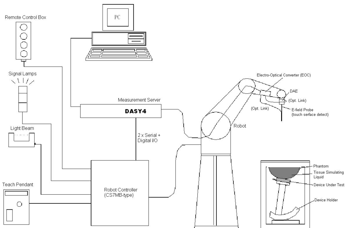
Fig. 5.1 DASY4 system
