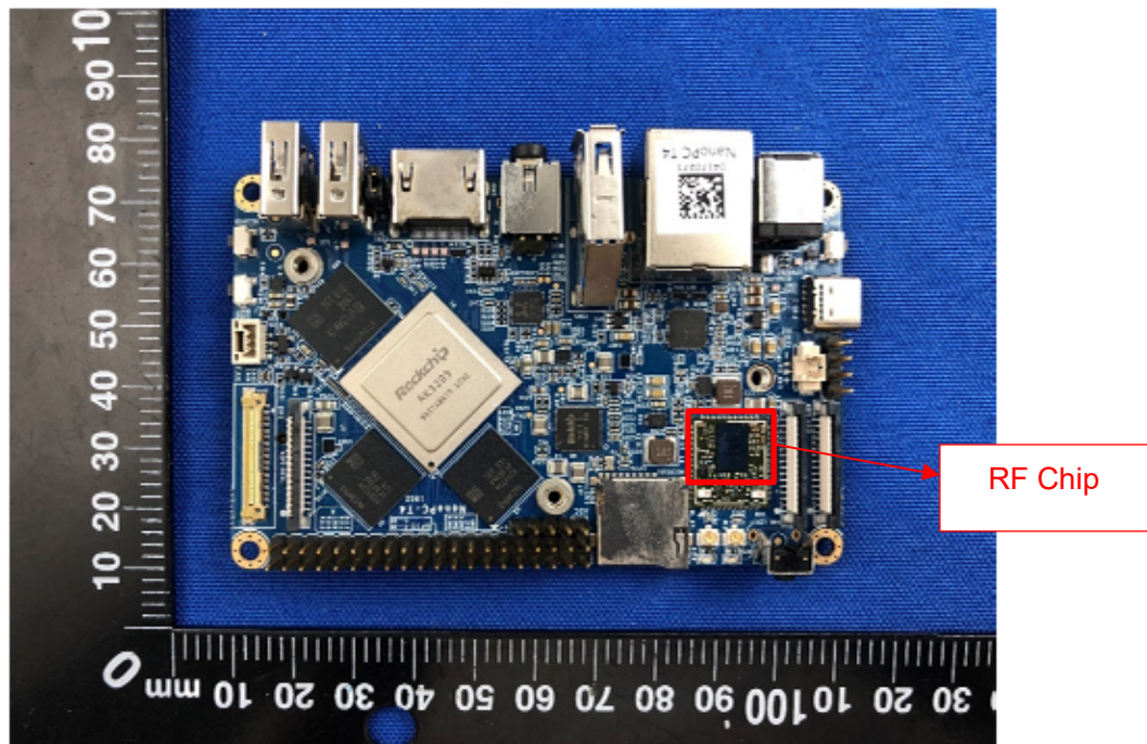
SECONDARY BOARD 1 REAR VIEW (WITHOUT SHIELDING)
