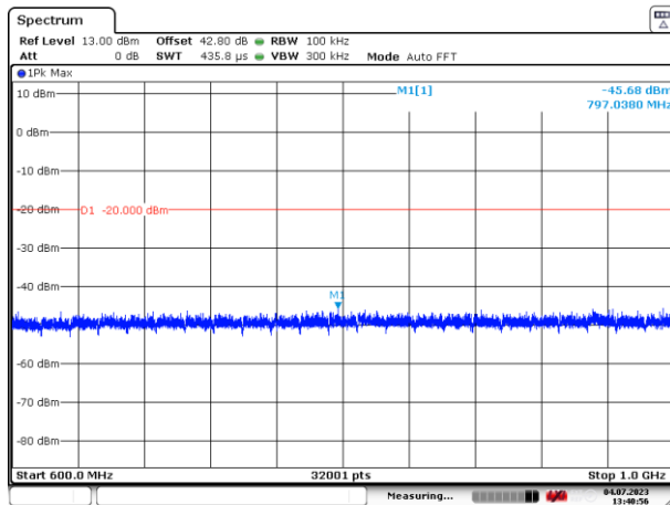
Figure 26: 600 – 1000 MHz
