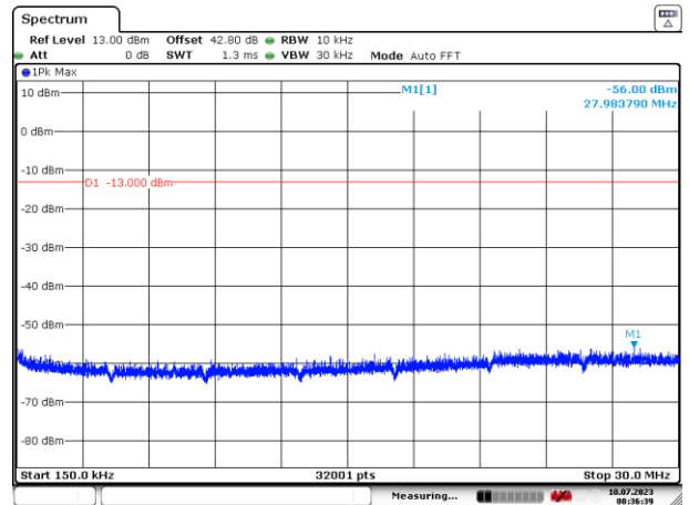
Figure 59: 150 kHz – 30 MHz
