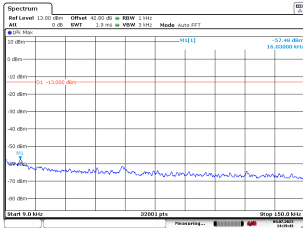
Figure 64: 9 – 150 kHz
