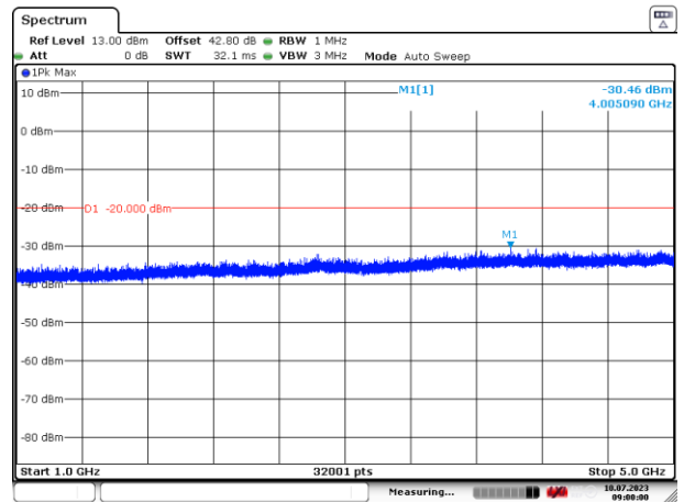
Figure 33: 1000 – 5000 MHz
