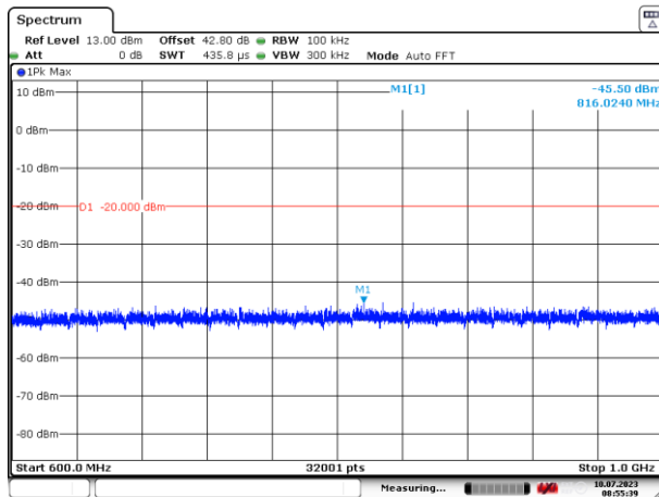
Figure 32: 600 – 1000 MHz
