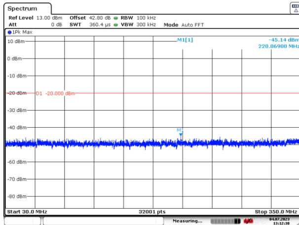
Figure 18: 30 – 350 MHz
