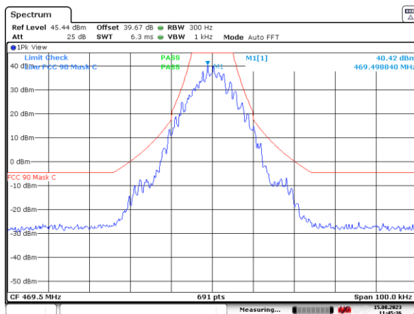
Figure 15: 469.5 MHz
