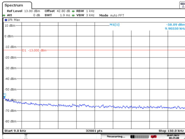
Figure 58: 9 – 150 kHz
