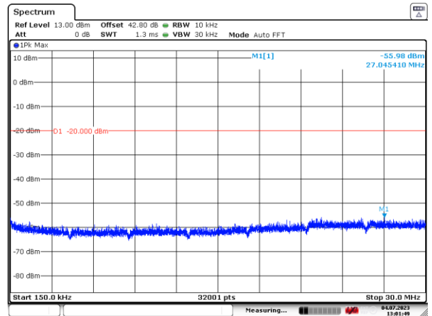
Figure 17: 150 kHz – 30 MHz
