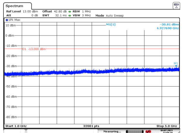
Figure 51: 1000 – 5000 MHz
