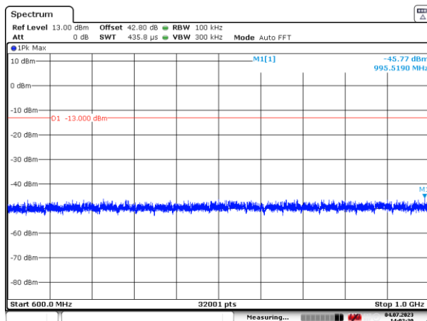
Figure 68: 600 – 1000 MHz
