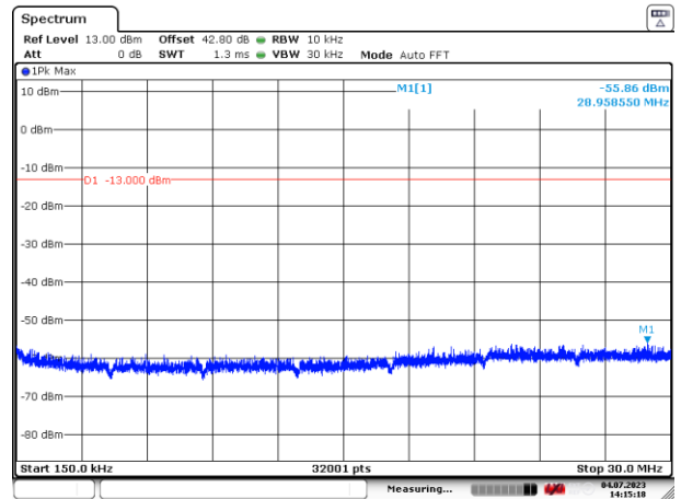
Figure 47: 150 kHz – 30 MHz
