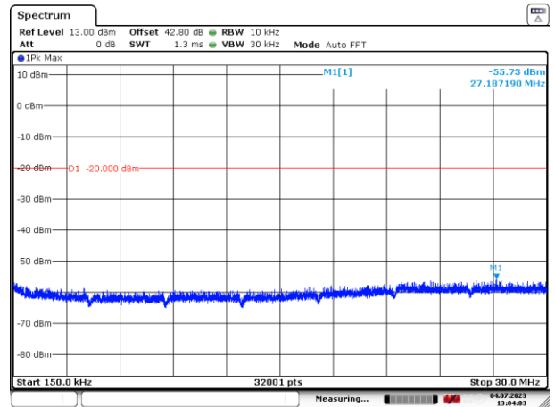
Figure 35: 150 kHz – 30 MHz
