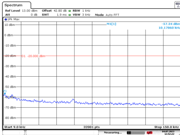
Figure 22: 9 – 150 kHz
