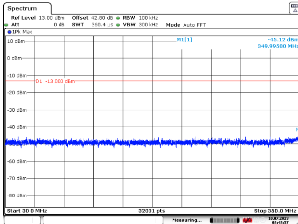
Figure 60: 30 – 350 MHz
