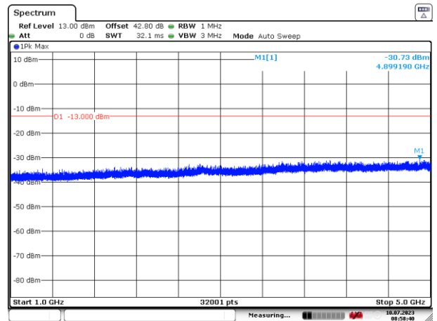
Figure 63: 1000 – 5000 MHz
