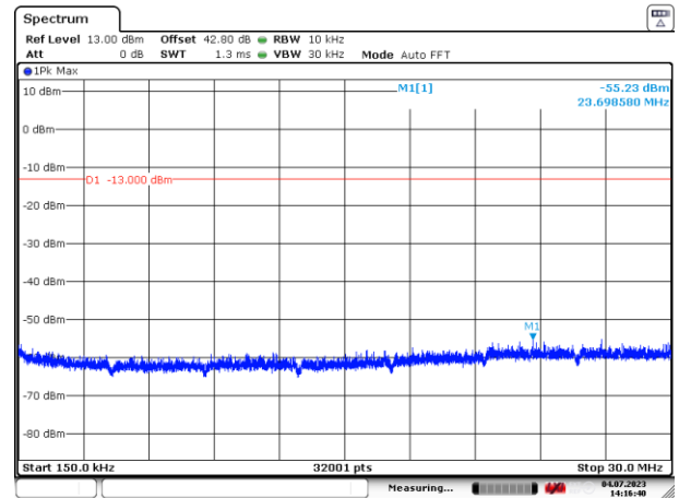
Figure 65: 150 kHz – 30 MHz
