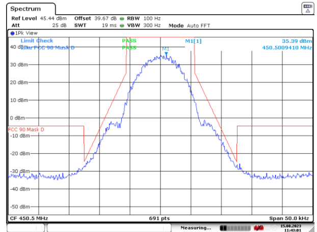
Figure 9: 450.5 MHz
