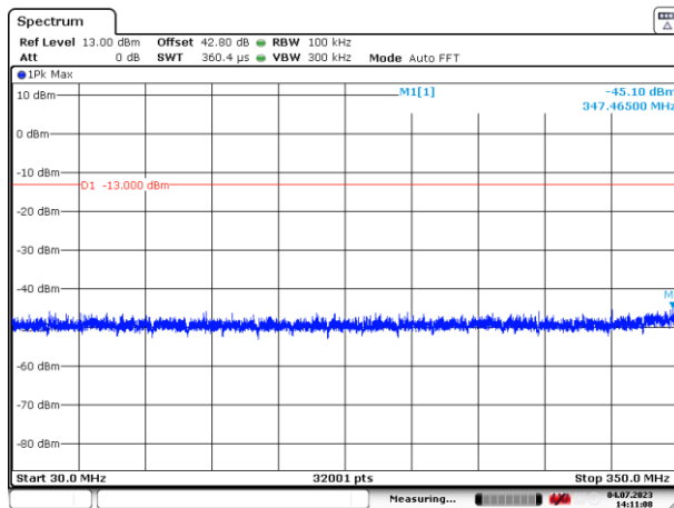
Figure 48: 30 – 350 MHz
