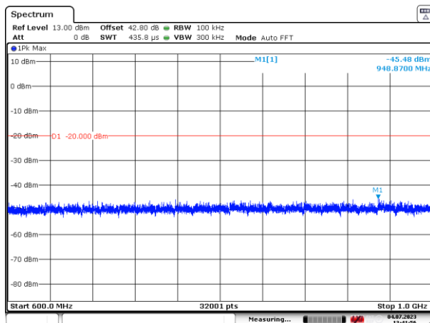
Figure 38: 600 – 1000 MHz
