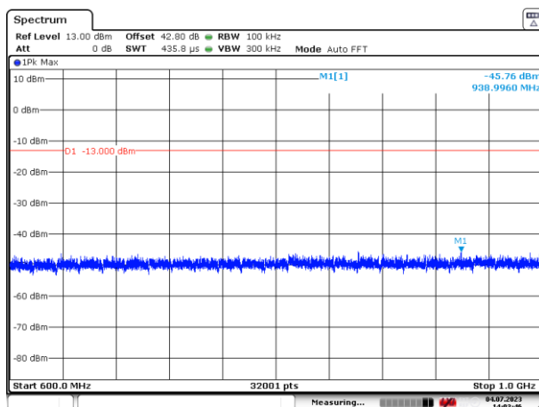
Figure 74: 600 – 1000 MHz
