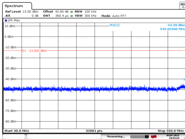
Figure 66: 30 – 350 MHz
