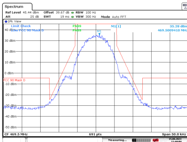
Figure 10: 469.5 MHz
