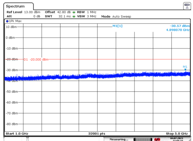
Figure 39: 1000 – 5000 MHz
