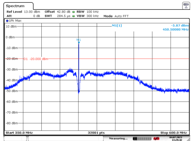
Figure 37: 350 – 600 MHz
