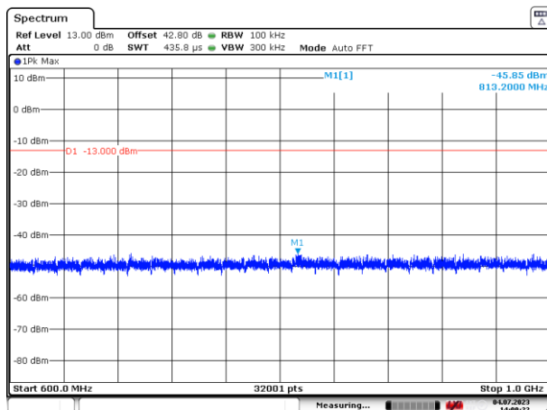
Figure 50: 600 – 1000 MHz
