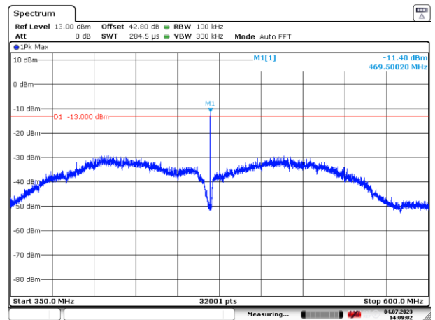
Figure 73: 350 – 600 MHz
