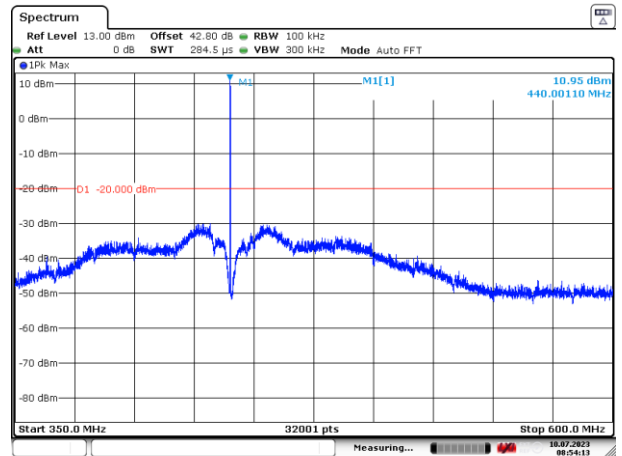
Figure 31: 350 – 600 MHz
