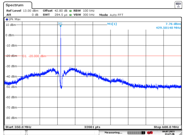
Figure 25: 350 – 600 MHz
