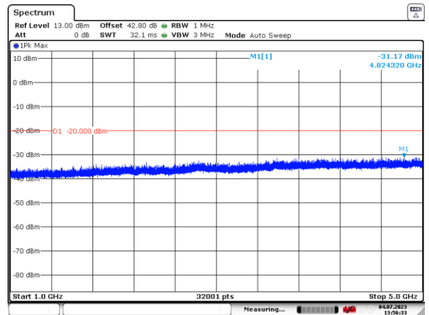
Figure 27: 1000 – 5000 MHz
