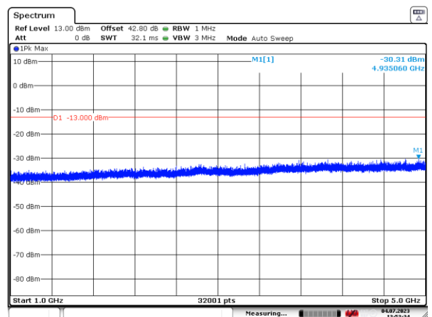
Figure 75: 1000 – 5000 MHz
