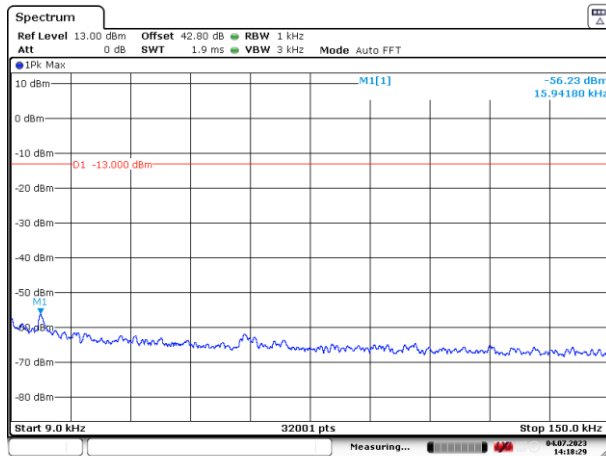
Figure 46: 9 – 150 kHz
