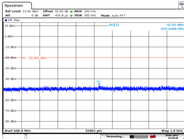
Figure 20: 600 – 1000 MHz
