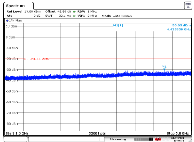
Figure 21: 1000 – 5000 MHz
