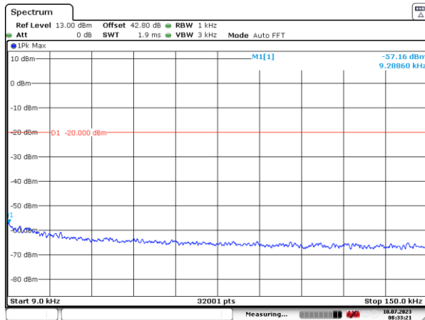
Figure 28: 9 – 150 kHz
