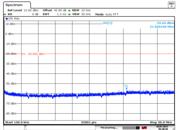
Figure 29: 150 kHz – 30 MHz
