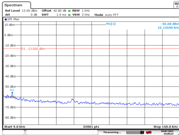
Figure 70: 9 – 150 kHz
