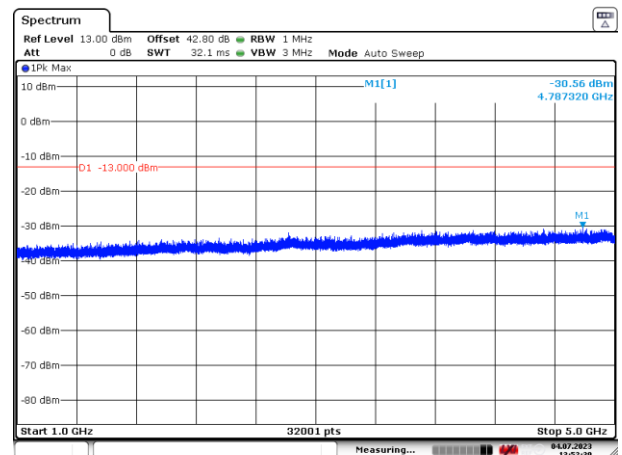
Figure 69: 1000 – 5000 MHz
