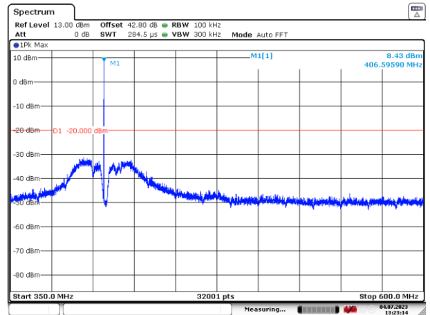
Figure 19: 350 – 600 MHz
