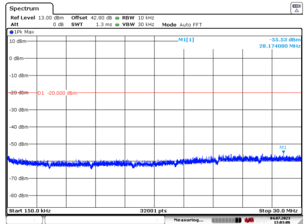
Figure 23: 150 kHz – 30 MHz
