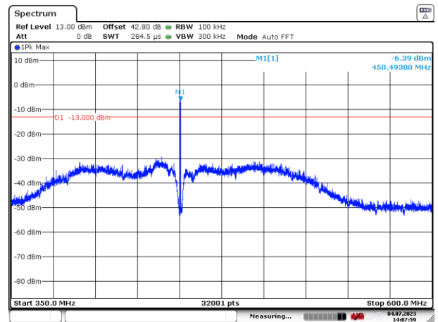
Figure 67: 350 – 600 MHz
