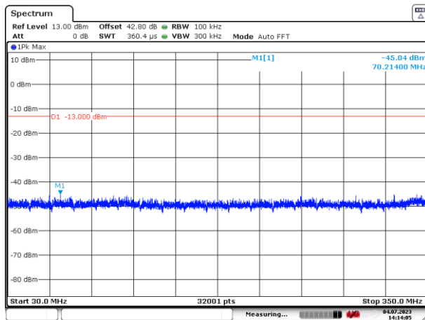
Figure 72: 30 – 350 MHz
