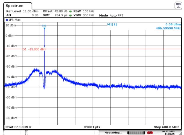
Figure 49: 350 – 600 MHz
