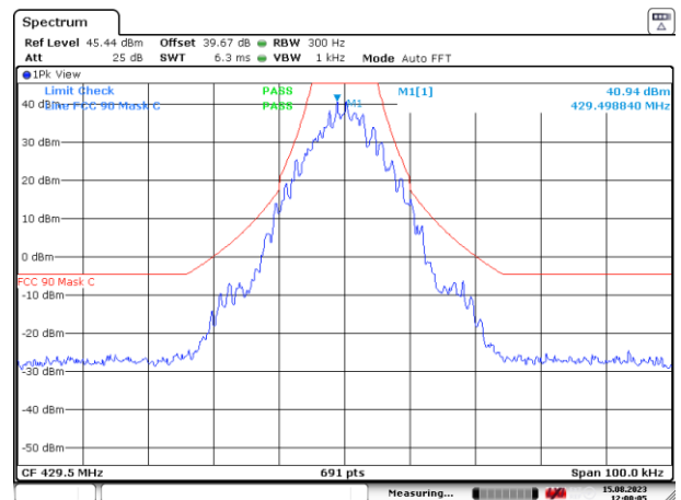
Figure 12: 429.5 MHz
