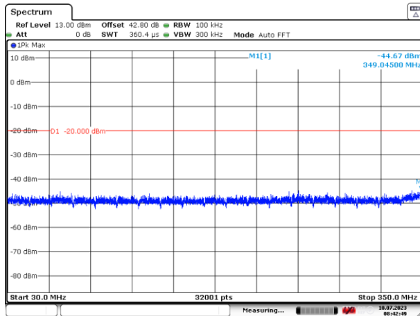
Figure 30: 30 – 350 MHz
