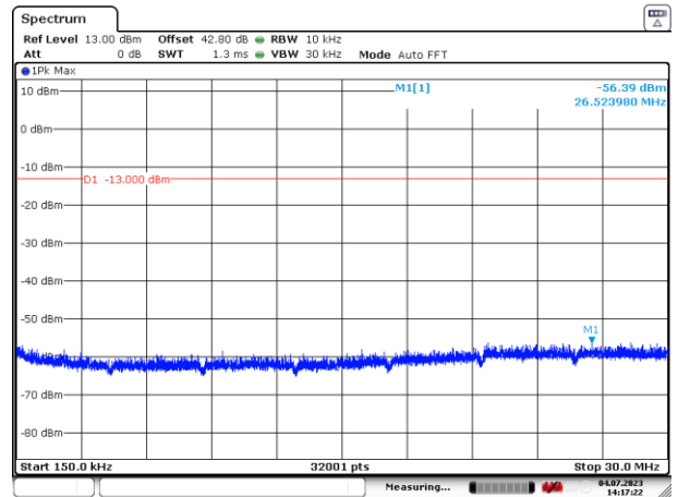
Figure 71: 150 kHz – 30 MHz
