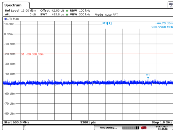
Figure 44: 600 – 1000 MHz
