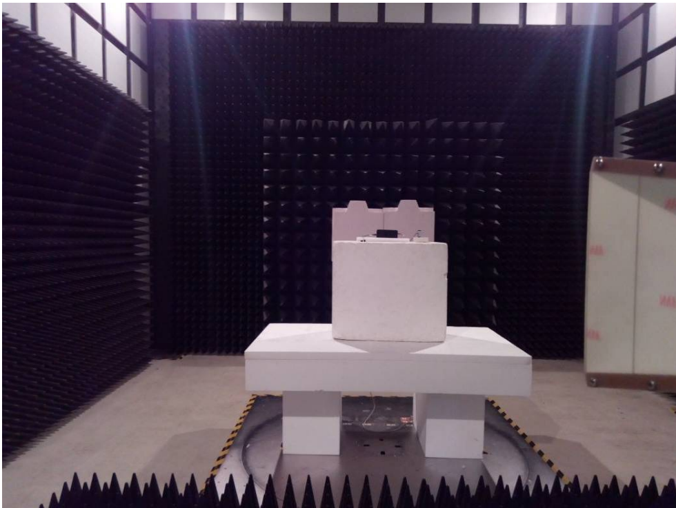
Radiated Emissions View (Above 1 GHz)
