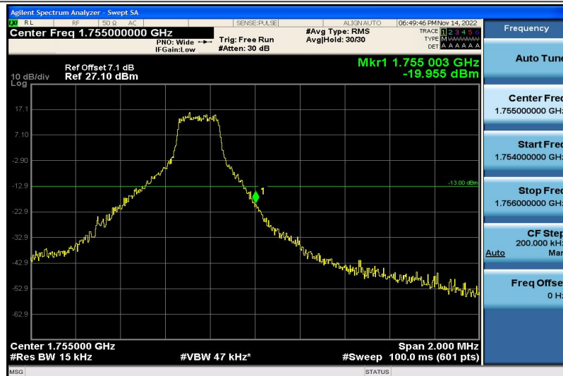
Band4-1.4MHz-QPSK-20393-1RB#5
