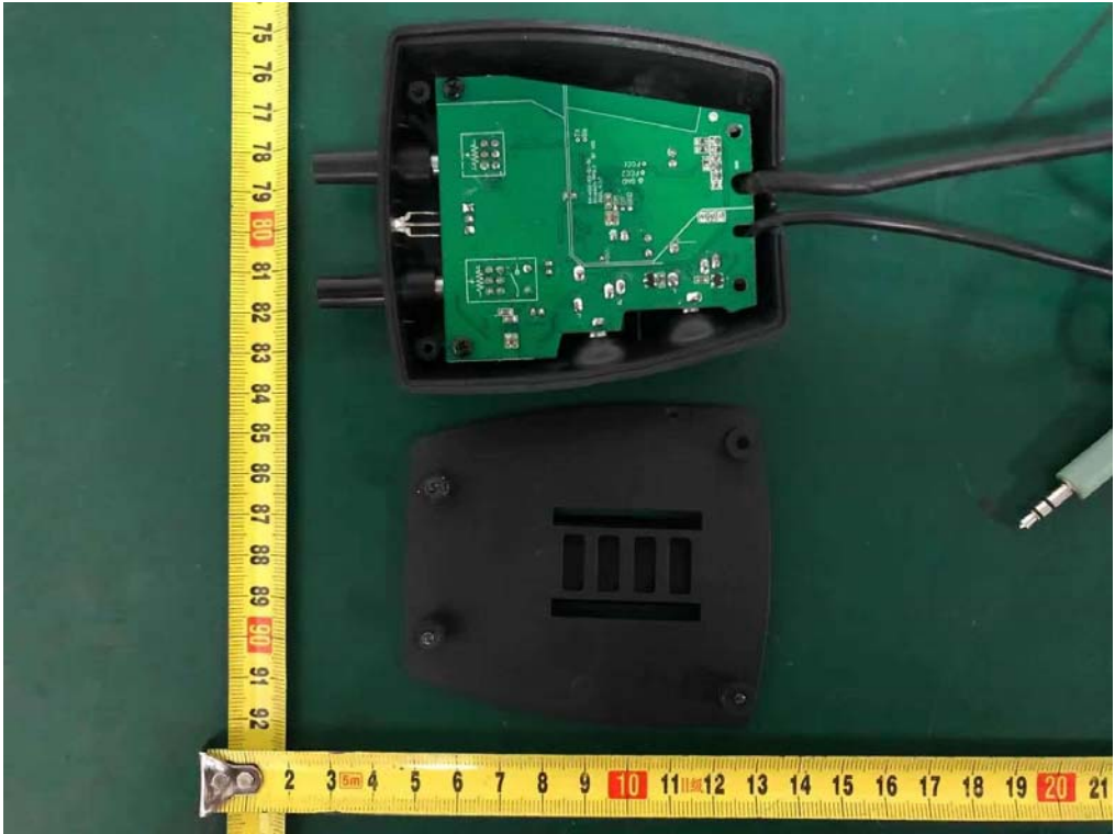
Internal Photos M/N: ProMedia 2.1 BT
